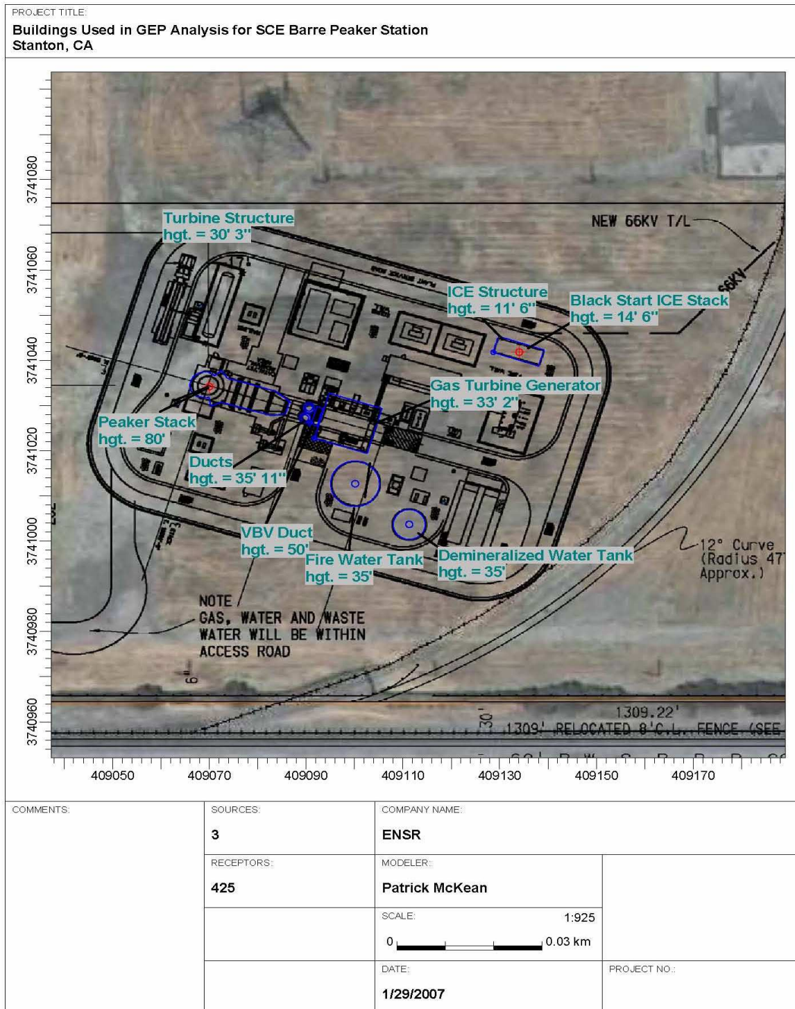
Figure C-1. Simplified Plot Plan
