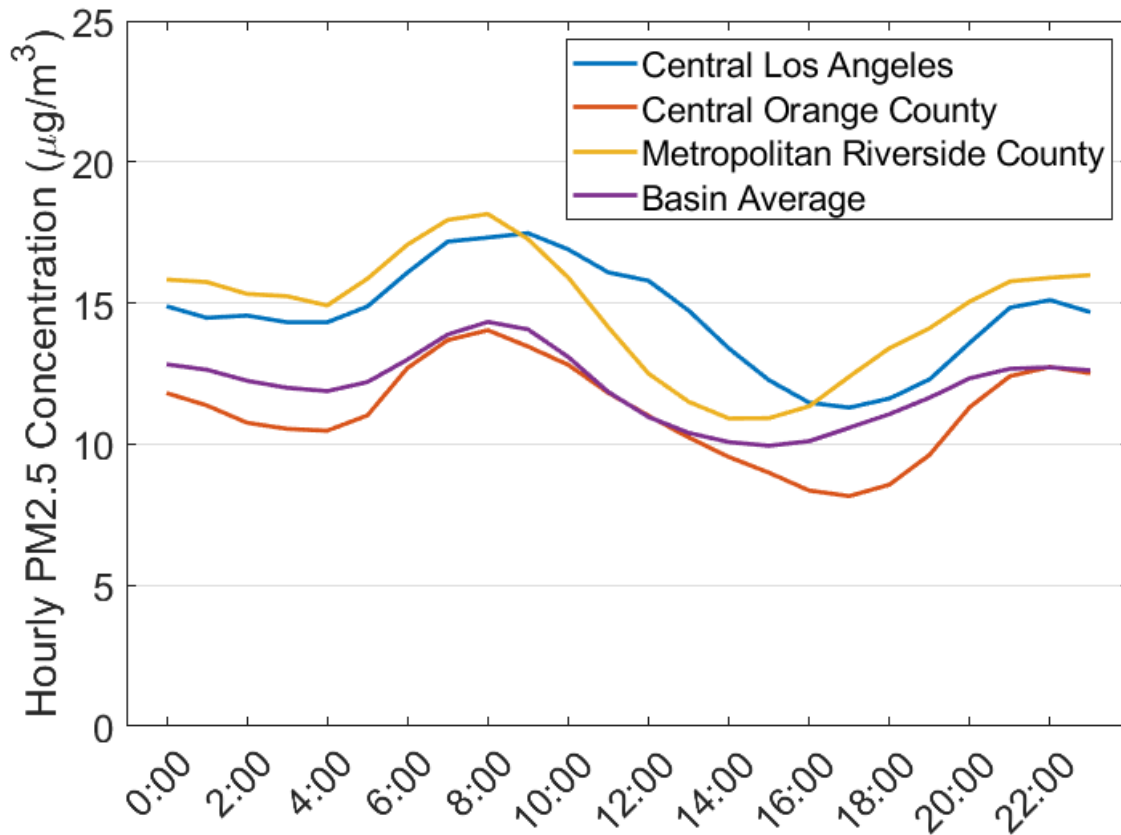
FIGURE 2-23 DIURNAL VARIATION OF HOURLY FEM PM2.5 CONCENTRATIONS, 2018–2020
