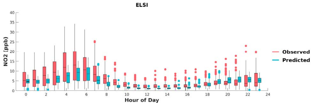
FIGURE H-6: BOX PLOTS OF OBSERVED VS. PREDICTED HOURLY NO 2 DURING MAY 1 ST TO SEPTEMBER 30 TH , 2018, AT LAKE ELSINORE. HORIZONTAL LINES INDICATE 25 TH , 50 TH (MEDIAN), AND 75 TH PERCENTILES.
