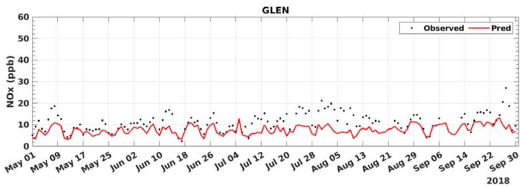
FIGURE D-8: 2018 DAILY AVERAGED NOX MODEL PREDICTION AND MEASUREMENT COMPARISON AT GLENDORA
