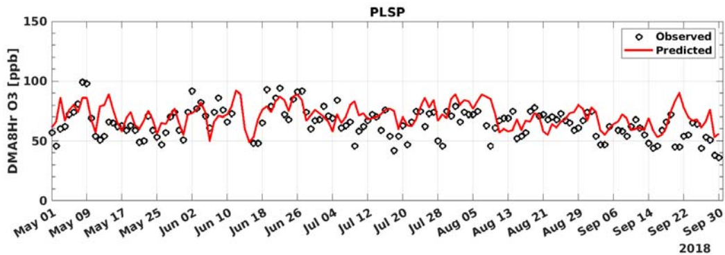
FIGURE A-17: 2018 MAXIMUM DAILY AVERAGE 8-HOUR (MDA8) OZONE MODEL PREDICTION AND MEASUREMENT COMPARISON AT PALM SPRINGS
