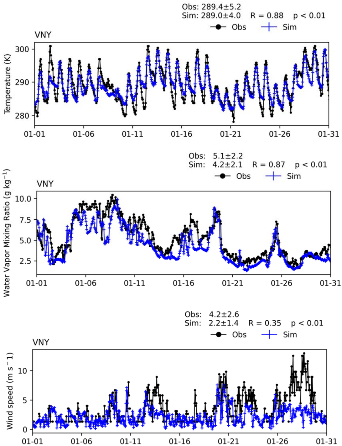
FIGURE V-A23 TIME SERIES OF HOURLY MEASUREMENTS AND WRF BASE SIMULATIONS AT VAN NUYS AIRPORT (VNY) FOR JANUARY 2018
