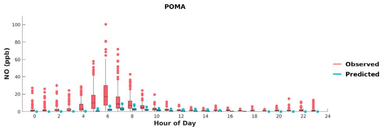
FIGURE G-15: BOX PLOTS OF OBSERVED VS. PREDICTED HOURLY NO DURING MAY 1 ST TO SEPTEMBER 30 TH , 2018, AT POMONA. HORIZONTAL LINES INDICATE 25 TH , 50 TH (MEDIAN), AND 75 TH PERCENTILES.
