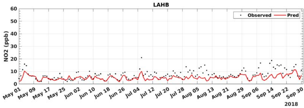
FIGURE C-10: 2018 DAILY AVERAGED NO2 MODEL PREDICTION AND MEASUREMENT COMPARISON AT LA HABRA
