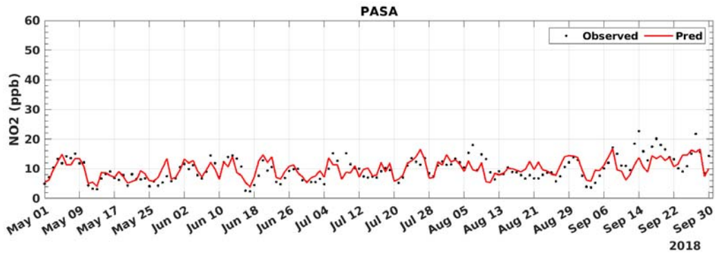
FIGURE C-13: 2018 DAILY AVERAGED NO2 MODEL PREDICTION AND MEASUREMENT COMPARISON AT PASADENA
