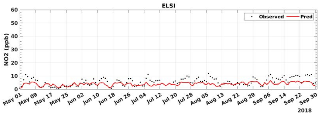
FIGURE C-6: 2018 DAILY AVERAGED NO2 MODEL PREDICTION AND MEASUREMENT COMPARISON AT LAKE ELSINORE
