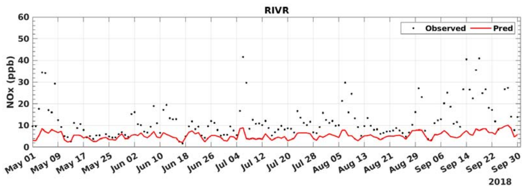
FIGURE D-18: 2018 DAILY AVERAGED NOX MODEL PREDICTION AND MEASUREMENT COMPARISON AT RIVERSIDE
