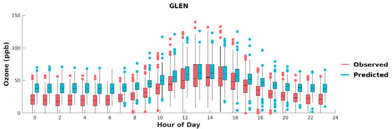
FIGURE F-9: BOX PLOTS OF OBSERVED VS. PREDICTED HOURLY OZONE DURING MAY 1 ST TO SEPTEMBER 30 TH , 2018, AT GLENDORA. HORIZONTAL LINES INDICATE 25 TH , 50 TH (MEDIAN), AND 75 TH PERCENTILES.
