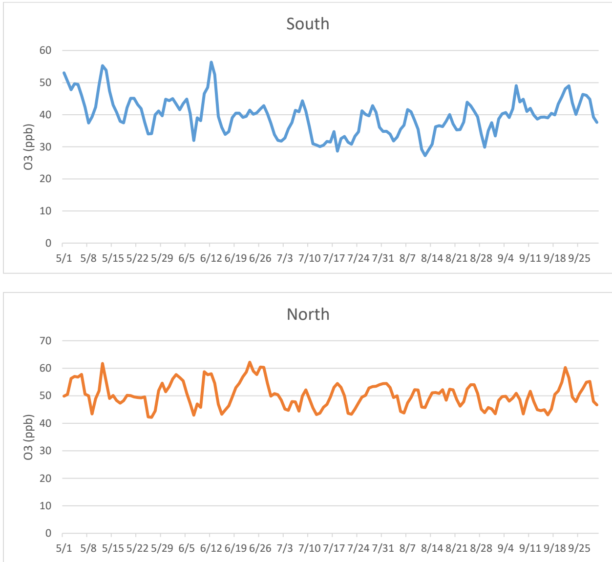
FIGURE V-4-21 SURFACE OZONE CONCENTRATION ALONG THE SOUTH AND NORTH BOUNDARIES
