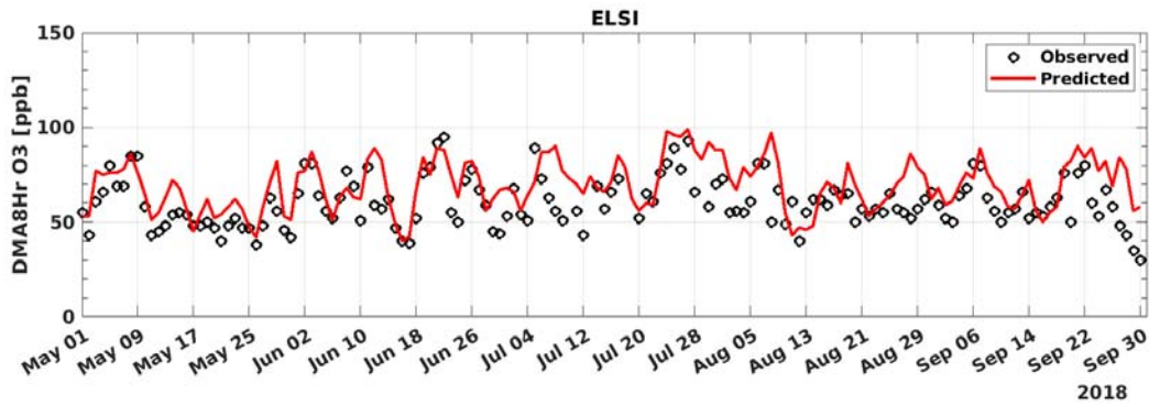
FIGURE A-7: 2018 MAXIMUM DAILY AVERAGE 8-HOUR (MDA8) OZONE MODEL PREDICTION AND MEASUREMENT COMPARISON AT LAKE ELSINORE
