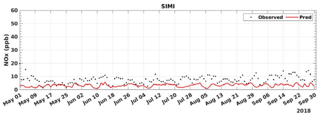
FIGURE D-20: 2018 DAILY AVERAGED NOX MODEL PREDICTION AND MEASUREMENT COMPARISON AT SIMI VALLEY
