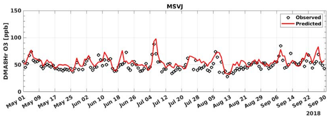
FIGURE A-15: 2018 MAXIMUM DAILY AVERAGE 8-HOUR (MDA8) OZONE MODEL PREDICTION AND MEASUREMENT COMPARISON AT MISSION VIEJO
