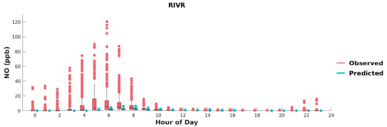
FIGURE G-18: BOX PLOTS OF OBSERVED VS. PREDICTED HOURLY NO DURING MAY 1 ST TO SEPTEMBER 30 TH , 2018, AT RIVERSIDE. HORIZONTAL LINES INDICATE 25 TH , 50 TH (MEDIAN), AND 75 TH PERCENTILES.
