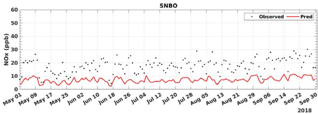
FIGURE D-21: 2018 DAILY AVERAGED NOX MODEL PREDICTION AND MEASUREMENT COMPARISON AT SAN BERNARDINO
