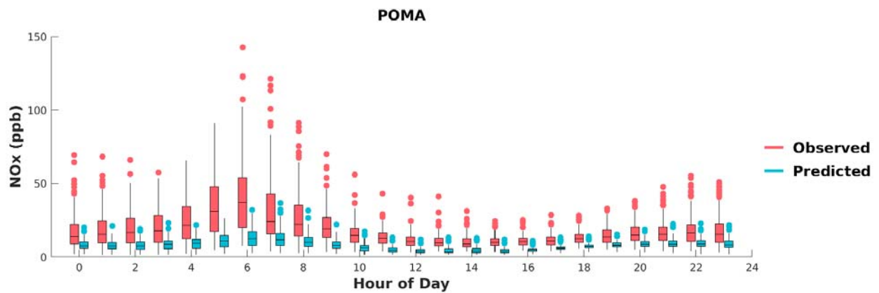
FIGURE I-16: BOX PLOTS OF OBSERVED VS. PREDICTED HOURLY NOX DURING MAY 1 ST TO SEPTEMBER 30 TH , 2018, AT POMONA. HORIZONTAL LINES INDICATE 25 TH , 50 TH (MEDIAN), AND 75 TH PERCENTILES.
