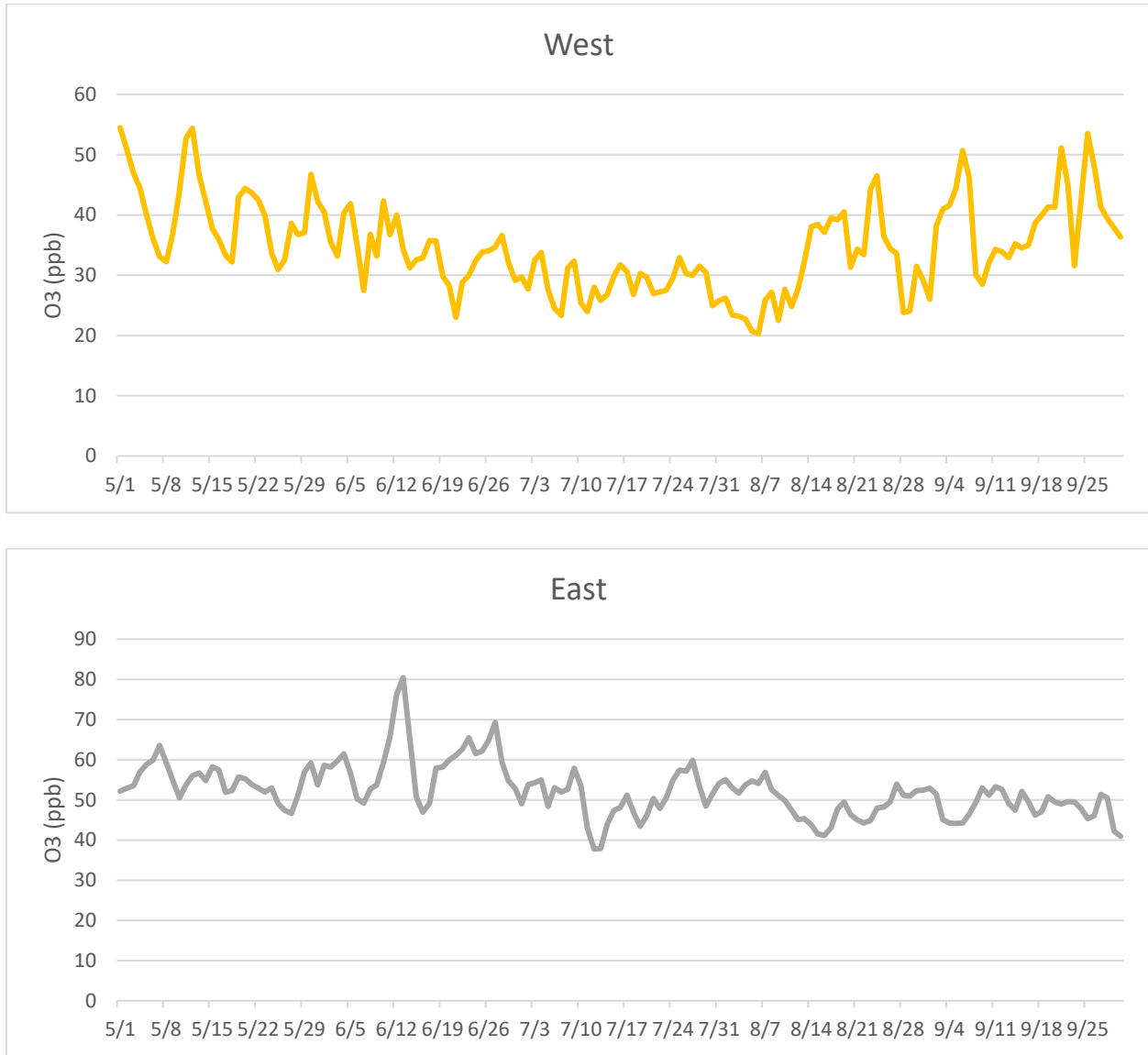
FIGURE V-4-22 SURFACE OZONE CONCENTRATION ALONG THE WEST AND EAST BOUNDARIES
