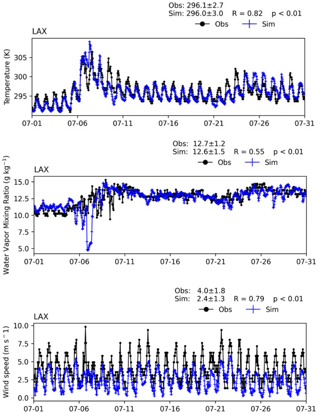
FIGURE V-A6 TIME SERIES OF HOURLY MEASUREMENTS AND WRF BASE SIMULATIONS AT LOS ANGELES AIRPORT (LAX) FOR JULY 2018
