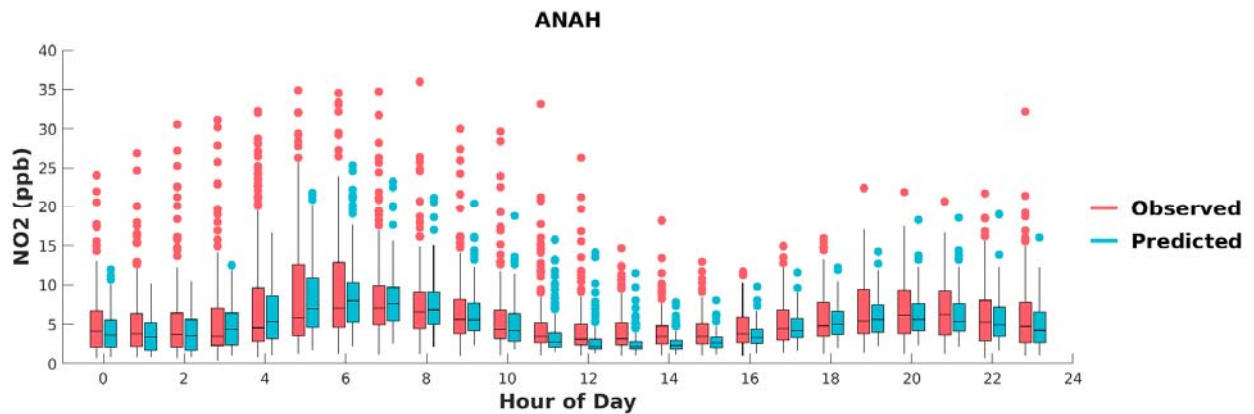
FIGURE H-1: BOX PLOTS OF OBSERVED VS. PREDICTED HOURLY NO2 DURING MAY 1 ST TO SEPTEMBER 30 TH , 2018, AT ANAHEIM. HORIZONTAL LINES INDICATE 25 TH , 50 TH (MEDIAN), AND 75 TH PERCENTILES.
