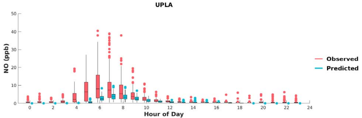
FIGURE G-22: BOX PLOTS OF OBSERVED VS. PREDICTED HOURLY NO DURING MAY 1 ST TO SEPTEMBER 30 TH , 2018, AT UPLAND. HORIZONTAL LINES INDICATE 25 TH , 50 TH (MEDIAN), AND 75 TH PERCENTILES.
