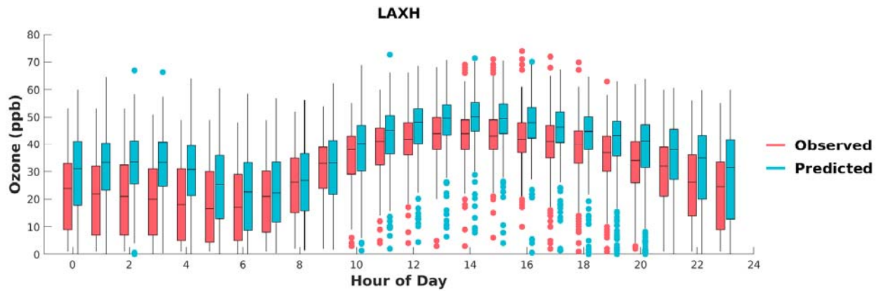
FIGURE F-14: BOX PLOTS OF OBSERVED VS. PREDICTED HOURLY OZONE DURING MAY 1 ST TO SEPTEMBER 30 TH , 2018, AT LAX. HORIZONTAL LINES INDICATE 25 TH , 50 TH (MEDIAN), AND 75 TH PERCENTILES.
