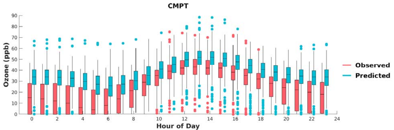
FIGURE F-5: BOX PLOTS OF OBSERVED VS. PREDICTED HOURLY OZONE DURING MAY 1 ST TO SEPTEMBER 30 TH , 2018, AT COMPTON. HORIZONTAL LINES INDICATE 25 TH , 50 TH (MEDIAN), AND 75 TH PERCENTILES.
