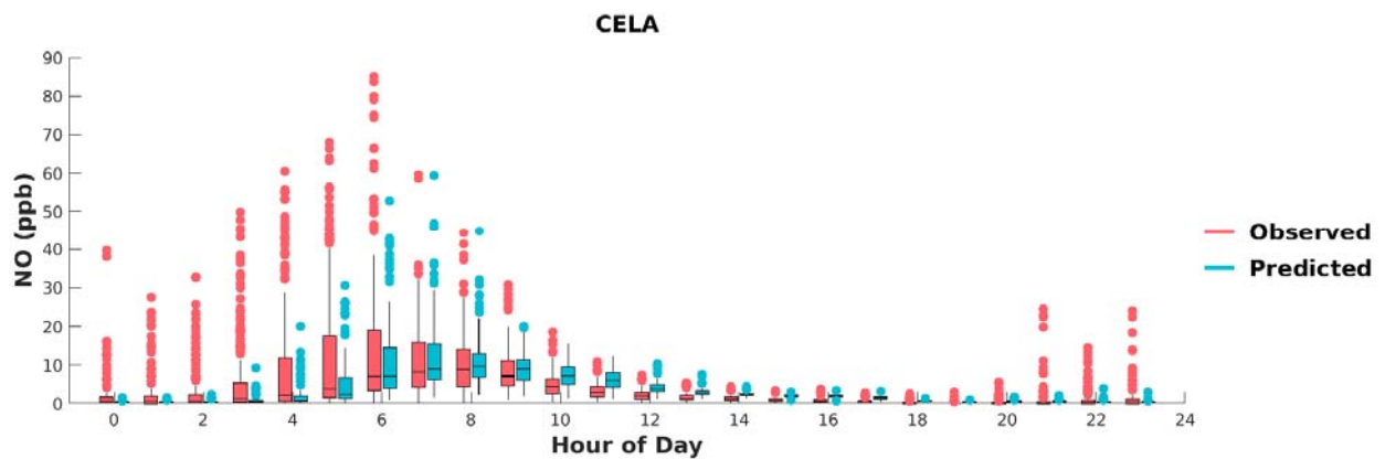
FIGURE G-4: BOX PLOTS OF OBSERVED VS. PREDICTED HOURLY NO DURING MAY 1 ST TO SEPTEMBER 30 TH , 2018, AT CENTRAL LOS ANGELES. HORIZONTAL LINES INDICATE 25 TH , 50 TH (MEDIAN), AND 75 TH PERCENTILES.
