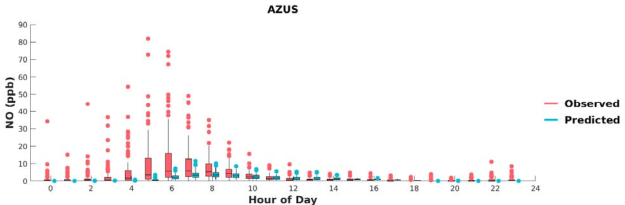
FIGURE G-2: BOX PLOTS OF OBSERVED VS. PREDICTED HOURLY NO DURING MAY 1 ST TO SEPTEMBER 30 TH , 2018, AT AZUSA. HORIZONTAL LINES INDICATE 25 TH , 50 TH (MEDIAN), AND 75 TH PERCENTILES.
