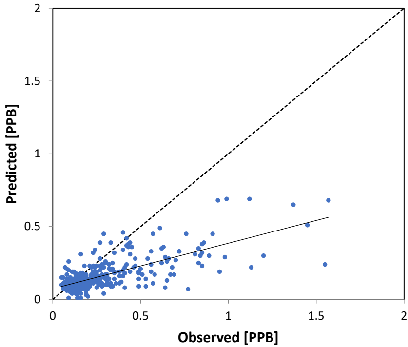
Figure 6. Scatter Plot of Predicted vs. Observed Concentrations Benzene
