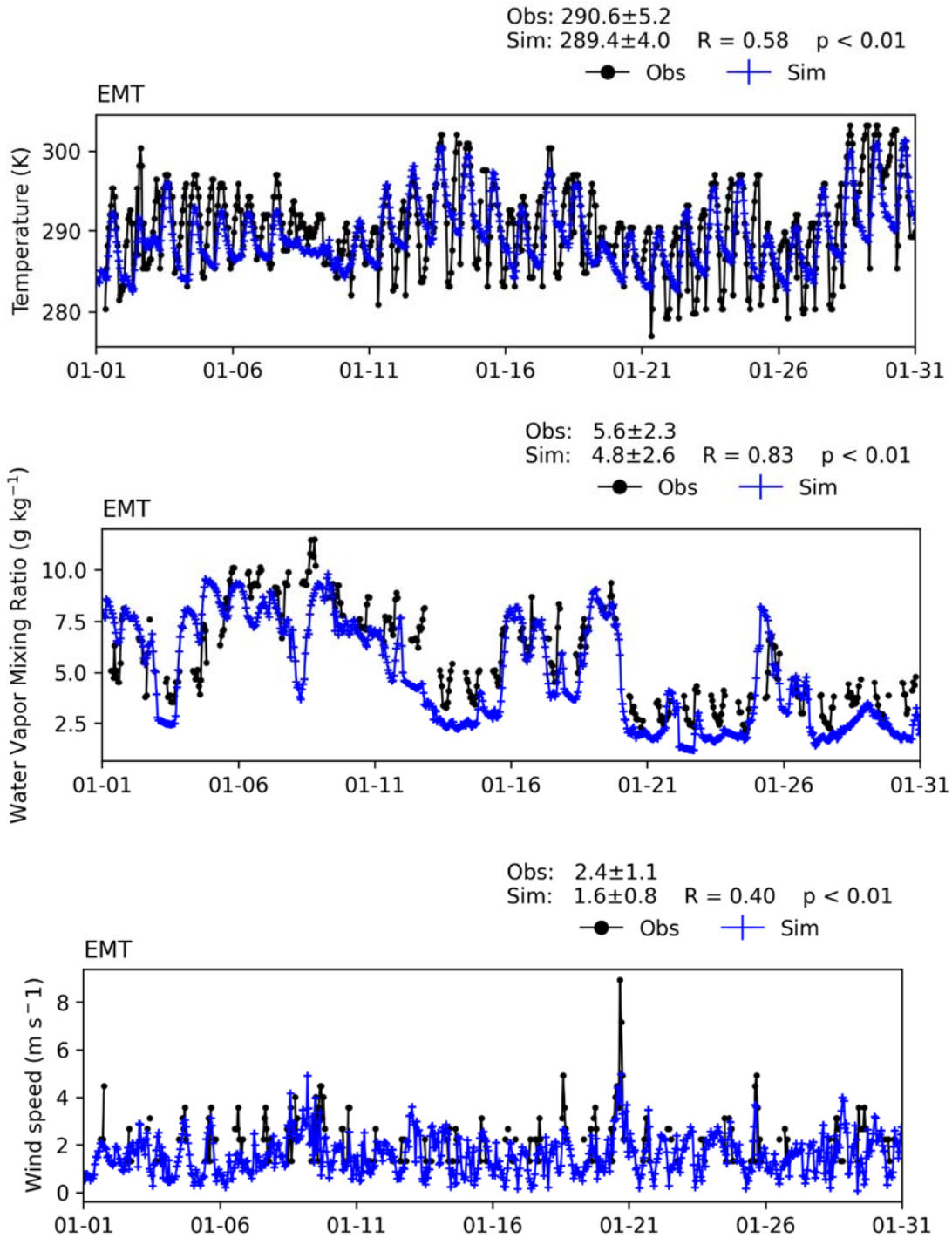
FIGURE V-A3 TIME SERIES OF HOURLY MEASUREMENTS AND WRF BASE SIMULATIONS AT EI MONTE (EMT) FOR JANUARY 2018
