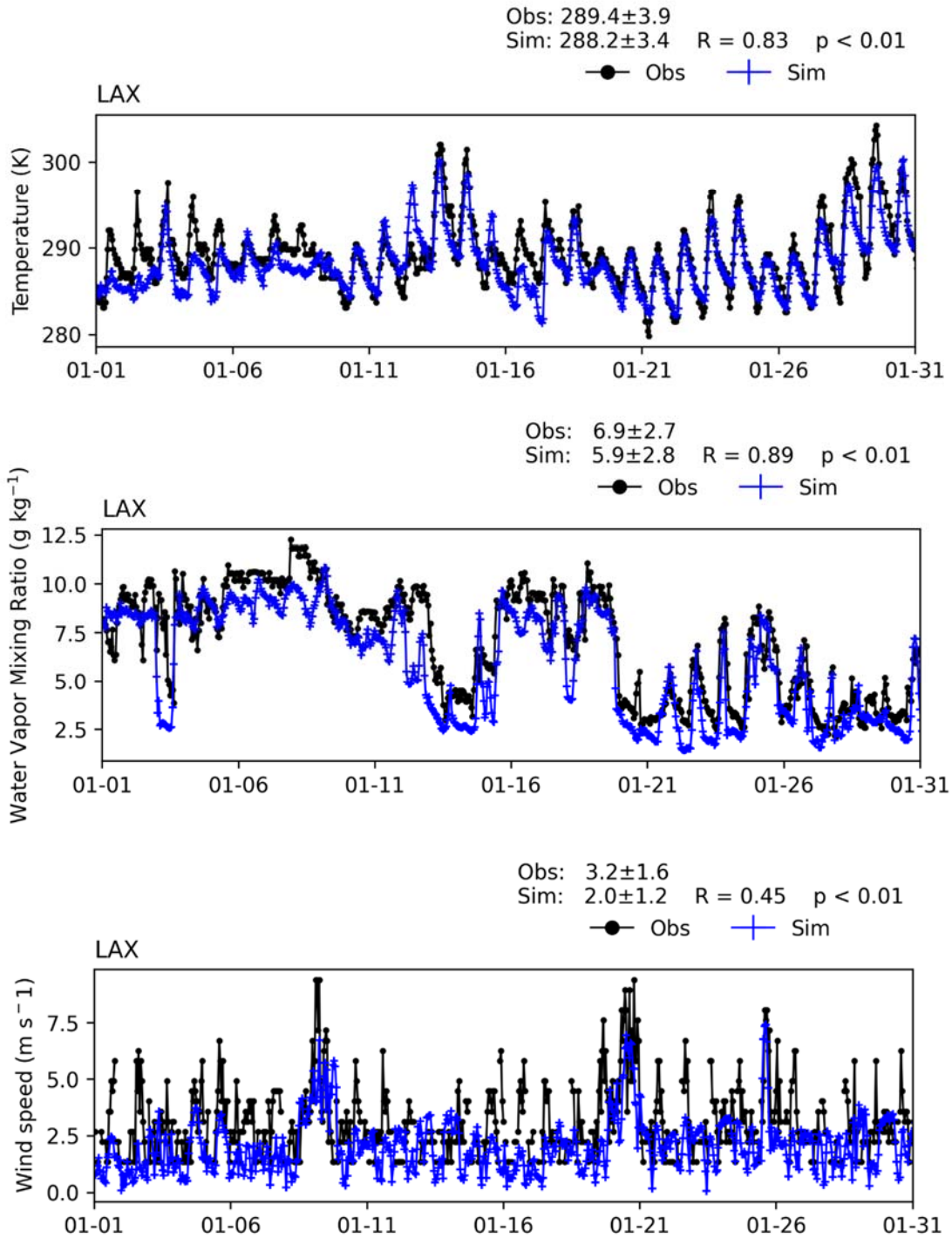
FIGURE V-A5 TIME SERIES OF HOURLY MEASUREMENTS AND WRF BASE SIMULATIONS AT LOS ANGELES AIRPORT (LAX) FOR JANUARY 2018
