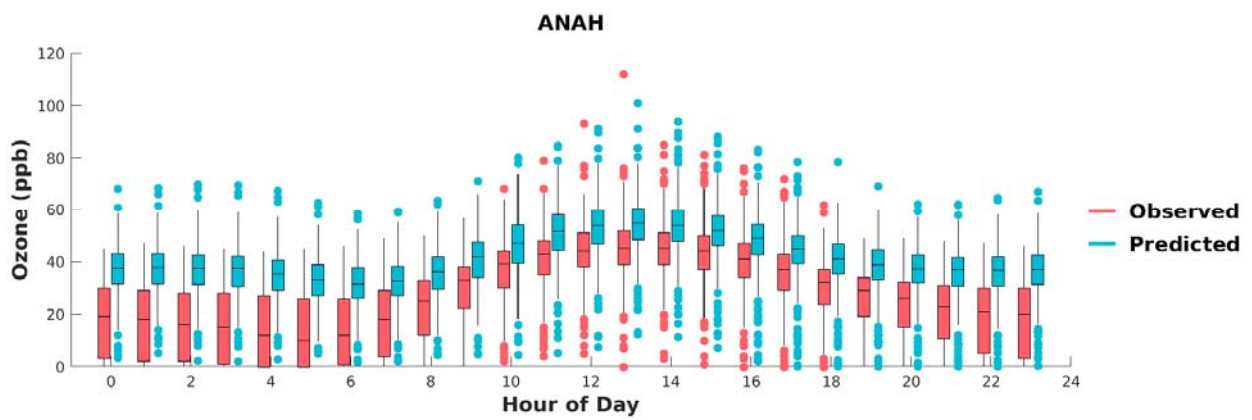
FIGURE F-1: BOX PLOTS OF OBSERVED VS. PREDICTED HOURLY OZONE DURING MAY 1 ST TO SEPTEMBER 30 TH , 2018, AT ANAHEIM. HORIZONTAL LINES INDICATE 25 TH , 50 TH (MEDIAN), AND 75 TH PERCENTILES.
