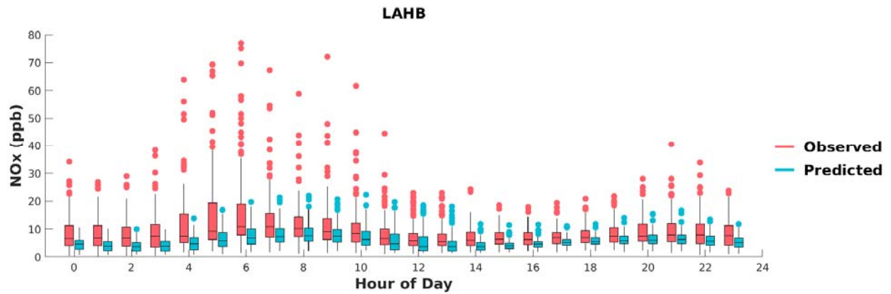
FIGURE I-10: BOX PLOTS OF OBSERVED VS. PREDICTED HOURLY NOx DURING MAY 1 ST TO SEPTEMBER 30 TH , 2018, AT LA HABRA. HORIZONTAL LINES INDICATE 25 TH , 50 TH (MEDIAN), AND 75 TH PERCENTILES.
