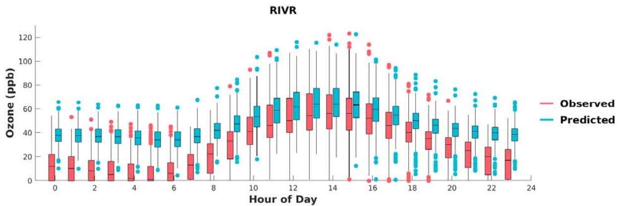
FIGURE F-25: BOX PLOTS OF OBSERVED VS. PREDICTED HOURLY OZONE DURING MAY 1 ST TO SEPTEMBER 30 TH , 2018, AT RIVERSIDE. HORIZONTAL LINES INDICATE 25 TH , 50 TH (MEDIAN), AND 75 TH PERCENTILES.
