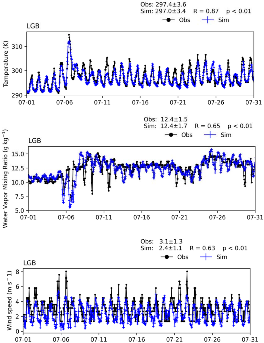
FIGURE V-A8 TIME SERIES OF HOURLY MEASUREMENTS AND WRF BASE SIMULATIONS AT LONG BEACH AIRPORT (LGB) FOR JULY 2018
