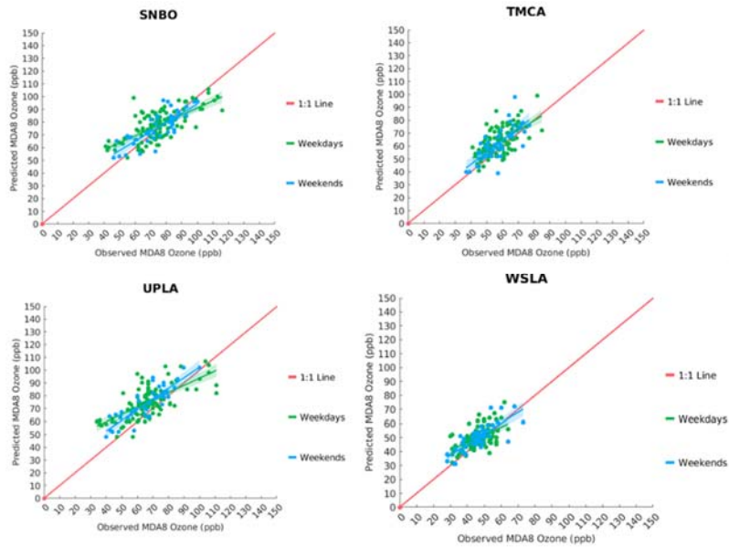
FIGURE K-5: SCATTER PLOT OF OBSERVED VS. PREDICTED MDAS OZONE DURING MAY 1 ST TO SEPTEMBER 30 TH , 2018, AT SAN BERNARDION (SNBO), TEMACULA (TMCA), UPLAND (UPLA), AND WEST LOS ANGELES (WSLA). GREEN AND BLUE LINES INDICATE GENERAL LINEAR MODEL FIT WITH 95% CONFIDENCE INTERVAL (SHADED AREA). THE RED LINE INDICATES 1:1 LINE.
