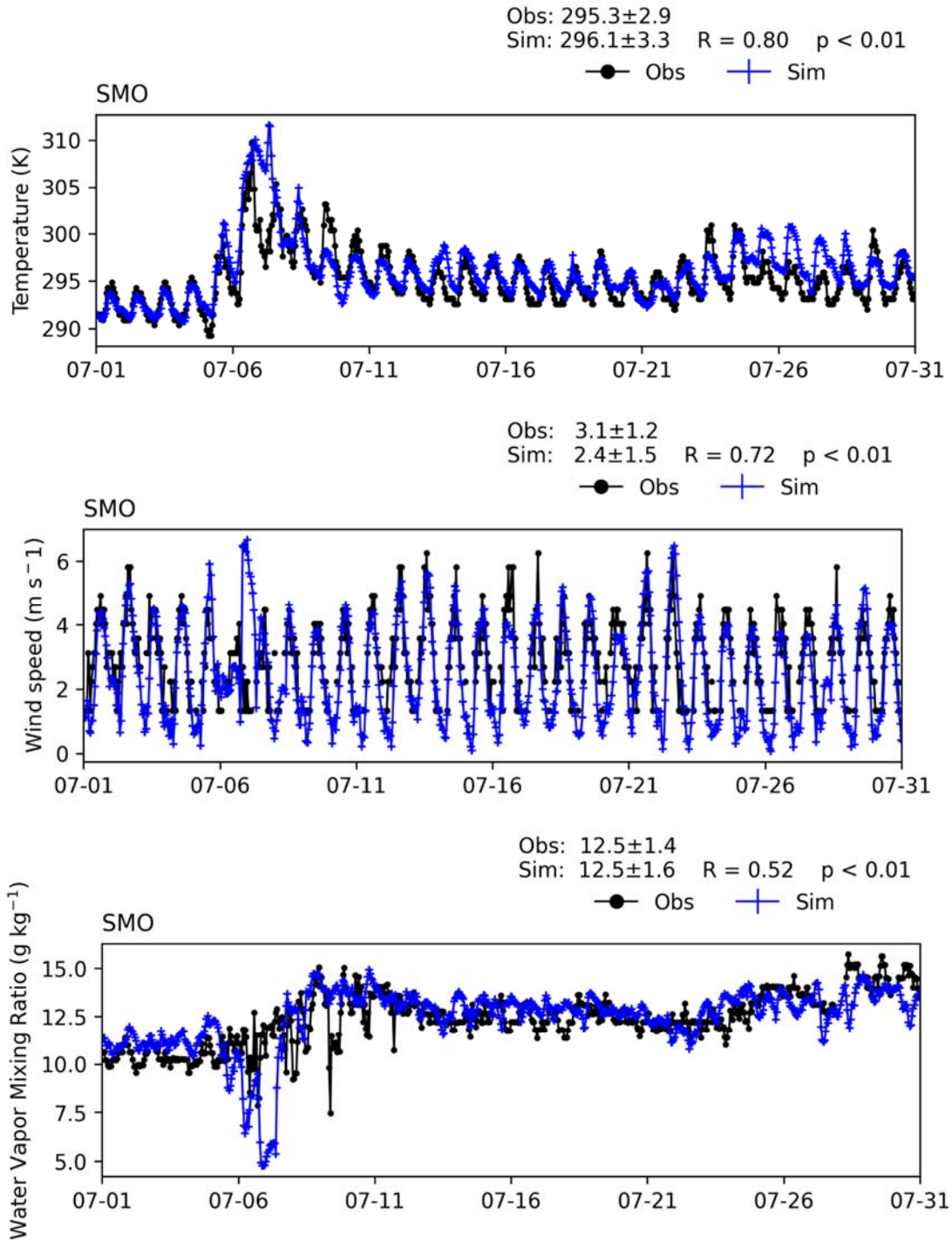
FIGURE V-A18 TIME SERIES OF HOURLY MEASUREMENTS AND WRF BASE SIMULATIONS AT SANTA MONICA AIRPORT (SMO) FOR JULY 2018
