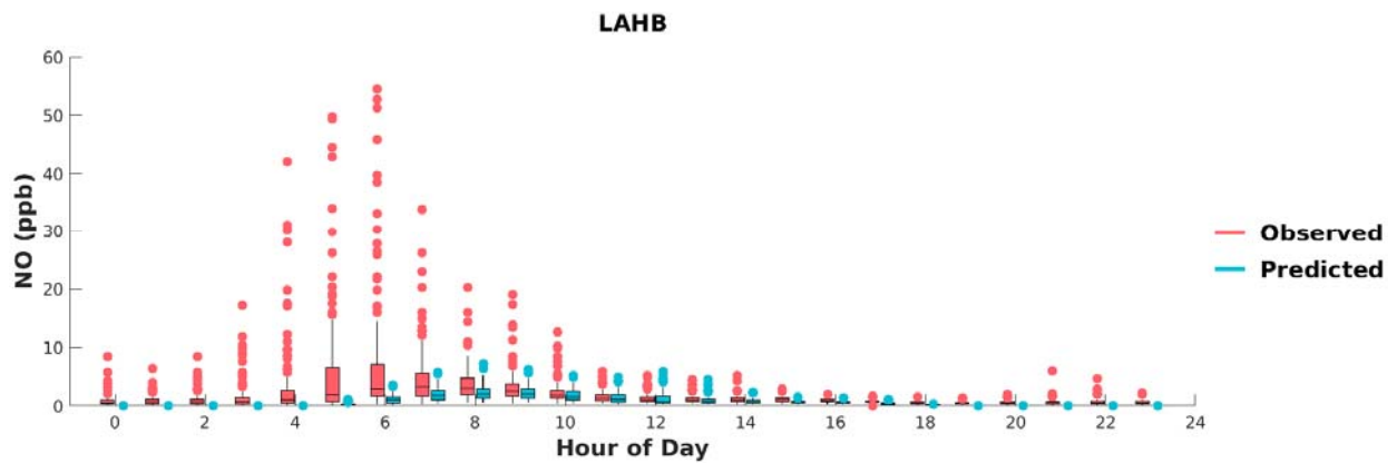
FIGURE G-10: BOX PLOTS OF OBSERVED VS. PREDICTED HOURLY NO DURING MAY 1 ST TO SEPTEMBER 30 TH , 2018, AT LA HABRA. HORIZONTAL LINES INDICATE 25 TH , 50 TH (MEDIAN), AND 75 TH PERCENTILES.
