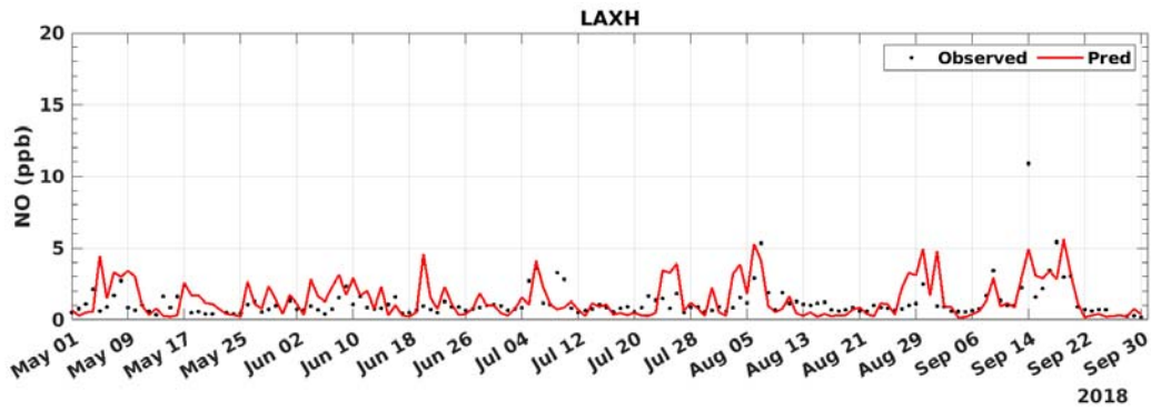
FIGURE B-13: 2018 DAILY AVERAGED NO MODEL PREDICTION AND MEASUREMENT COMPARISON AT LAX
