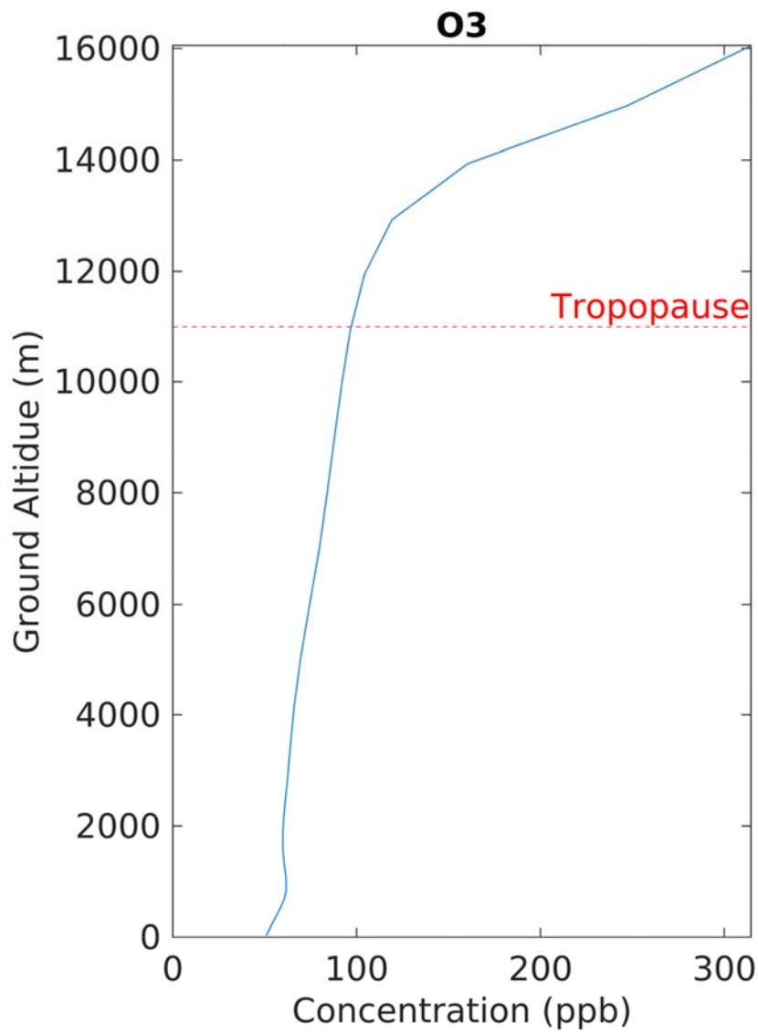
Figure 3: Vertical profile of O3 averaged over the Basin during July 2018
