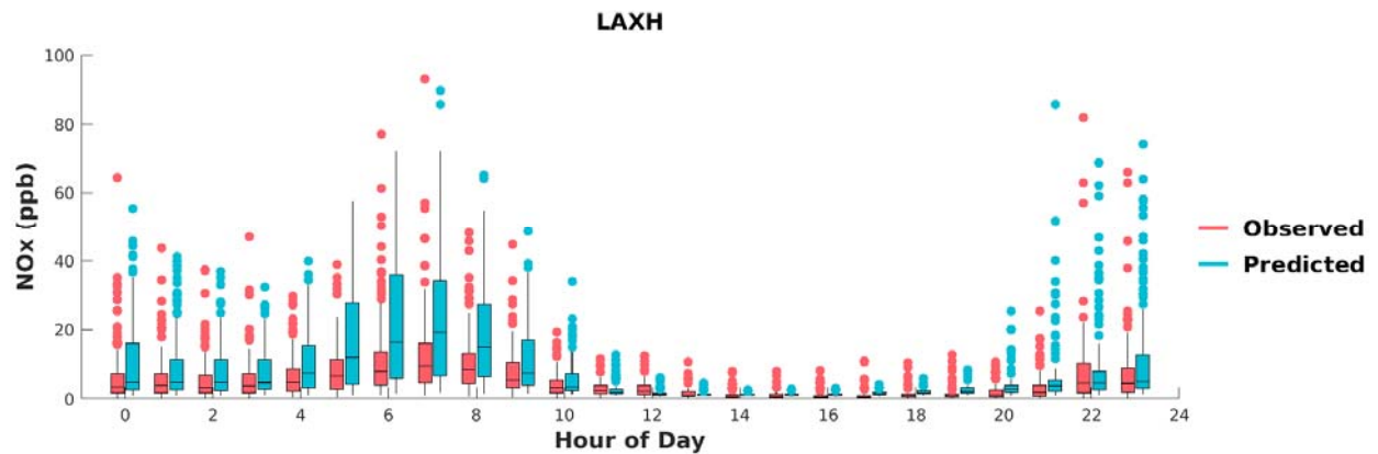
FIGURE I-11: BOX PLOTS OF OBSERVED VS. PREDICTED HOURLY NOx DURING MAY 1 ST TO SEPTEMBER 30 TH , 2018, AT LAX. HORIZONTAL LINES INDICATE 25 TH , 50 TH (MEDIAN), AND 75 TH PERCENTILES.
