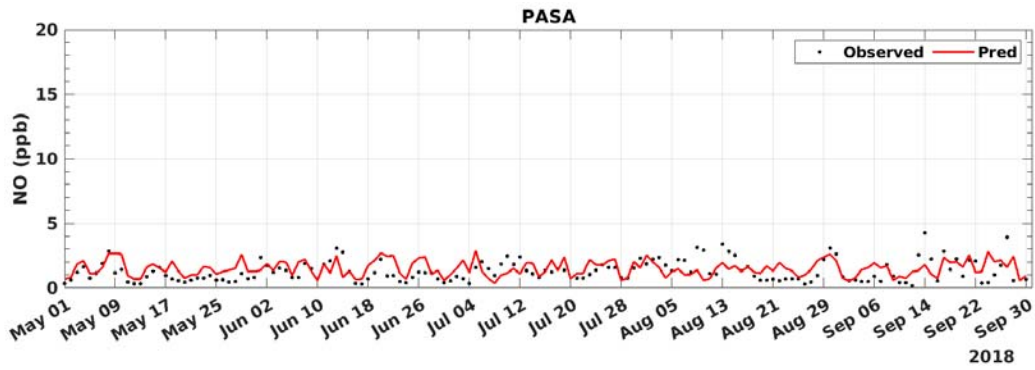
FIGURE B-16: 2018 DAILY AVERAGED NO MODEL PREDICTION AND MEASUREMENT COMPARISON AT PASADENA
