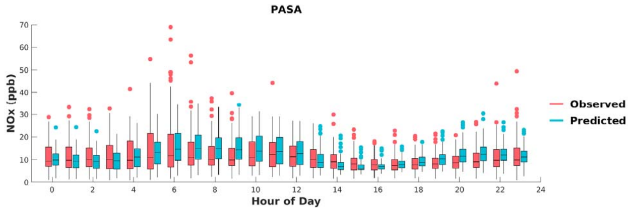
FIGURE I-13: BOX PLOTS OF OBSERVED VS. PREDICTED HOURLY NOX DURING MAY 1 ST TO SEPTEMBER 30 TH , 2018, AT PASADENA. HORIZONTAL LINES INDICATE 25 TH , 50 TH (MEDIAN), AND 75 TH PERCENTILES.
