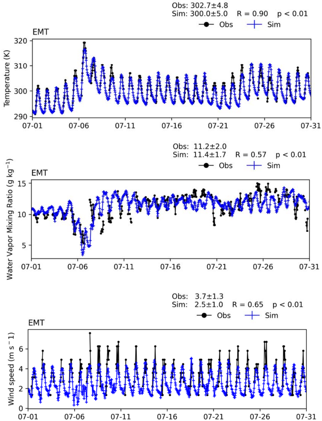
FIGURE V-A4 TIME SERIES OF HOURLY MEASUREMENTS AND WRF BASE SIMULATIONS AT EI MONTE (EMT) FOR JULY 2018
