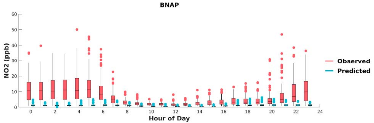
FIGURE H-3: BOX PLOTS OF OBSERVED VS. PREDICTED HOURLY NO 2 DURING MAY 1 ST TO SEPTEMBER 30 TH , 2018, AT BANNING. HORIZONTAL LINES INDICATE 25 TH , 50 TH (MEDIAN), AND 75 TH PERCENTILES.
