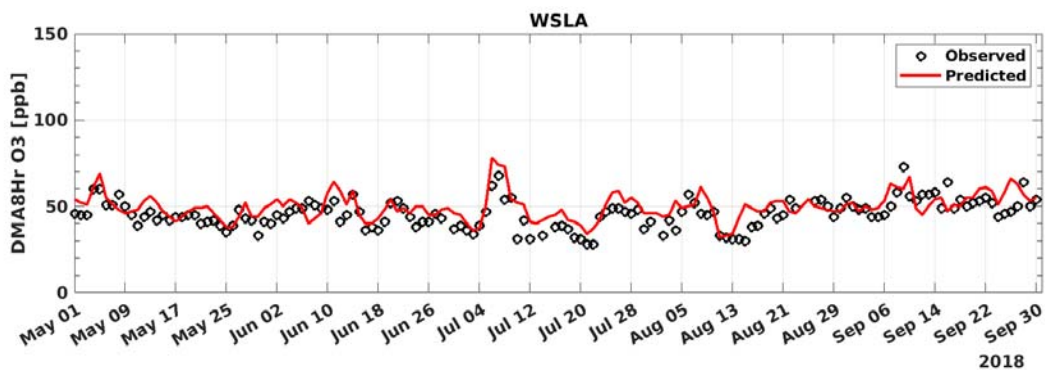
FIGURE A-27: 2018 MAXIMUM DAILY AVERAGE 8-HOUR (MDA8) OZONE MODEL PREDICTION AND MEASUREMENT COMPARISON AT WEST LOS ANGELES
