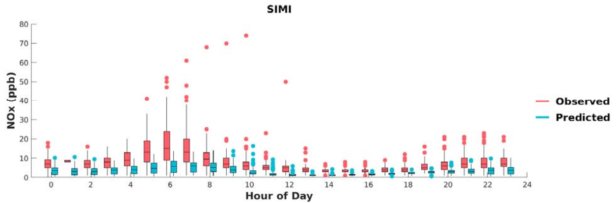
FIGURE I-20: BOX PLOTS OF OBSERVED VS. PREDICTED HOURLY NOx DURING MAY 1 ST TO SEPTEMBER 30 TH , 2018, AT SIMI VALLEY. HORIZONTAL LINES INDICATE 25 TH , 50 TH (MEDIAN), AND 75 TH PERCENTILES.
