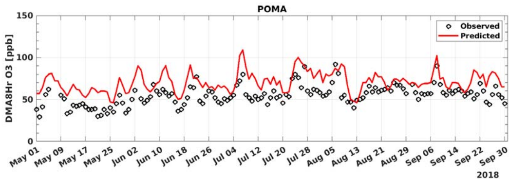
FIGURE A-18: 2018 MAXIMUM DAILY AVERAGE 8-HOUR (MDA8) OZONE MODEL PREDICTION AND MEASUREMENT COMPARISON AT POMONA
