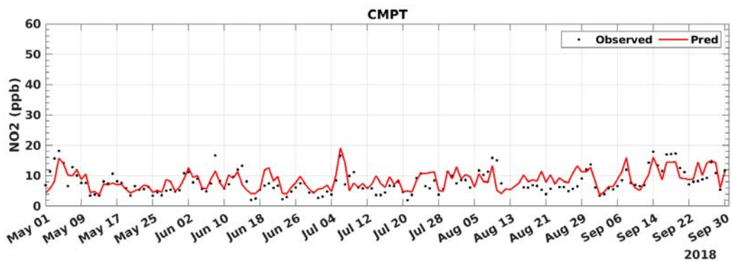
FIGURE C-5: 2018 DAILY AVERAGED NO2 MODEL PREDICTION AND MEASUREMENT COMPARISON AT COMPTON
