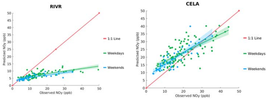
FIGURE O-1: SCATTER PLOT OF OBSERVED VS. PREDICTED DAILY AVERAGE NOy DURING MAY 1 ST TO SEPTEMBER 30 TH , 2018, AT RIVERSIDE (RIVR) AND CENTRAL LOS ANGELES (CELA). GREEN AND BLUE LINES INDICATE GENERAL LINEAR MODEL FIT WITH 95% CONFIDENCE INTERVAL (SHADED AREA). THE RED LINE INDICATES 1:1 LINE.
