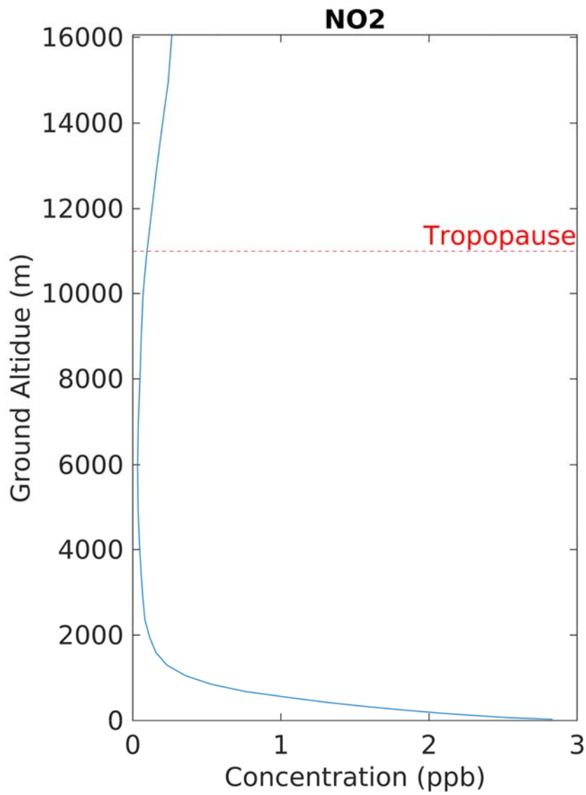
Figure 2: Vertical profile of NO2 averaged over the Basin during July 2018
