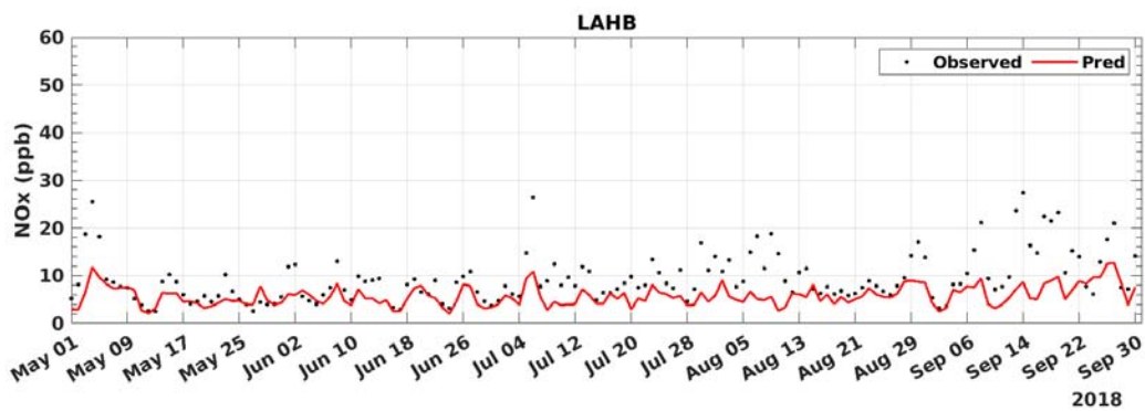
FIGURE D-11: 2018 DAILY AVERAGED NOX MODEL PREDICTION AND MEASUREMENT COMPARISON AT LA HABRA
