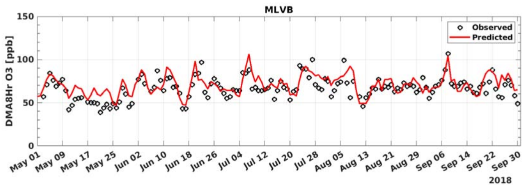
FIGURE A-142: 2018 MAXIMUM DAILY AVERAGE 8-HOUR (MDA8) OZONE MODEL PREDICTION AND MEASUREMENT COMPARISON AT MIRA LOMA
