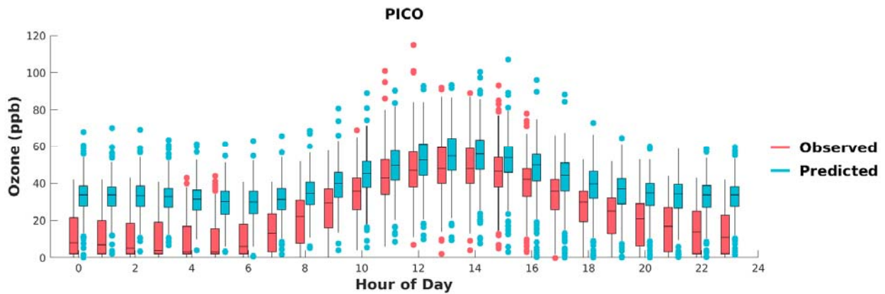
FIGURE F-20: BOX PLOTS OF OBSERVED VS. PREDICTED HOURLY OZONE DURING MAY 1 ST TO SEPTEMBER 30 TH , 2018, AT PICO RIVERO. HORIZONTAL LINES INDICATE 25 TH , 50 TH (MEDIAN), AND 75 TH PERCENTILES.
