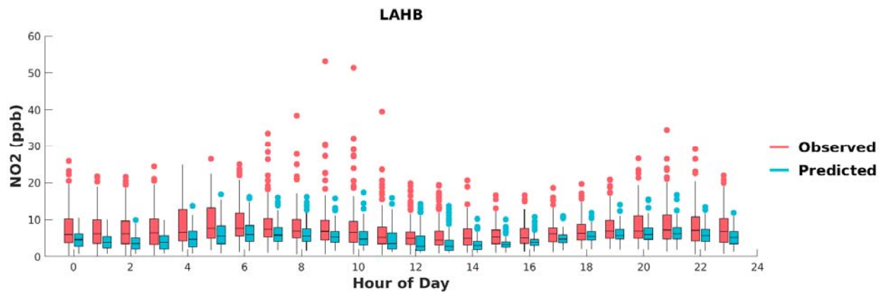
FIGURE H-10: BOX PLOTS OF OBSERVED VS. PREDICTED HOURLY NO 2 DURING MAY 1 ST TO SEPTEMBER 30 TH , 2018, AT LA HABRA. HORIZONTAL LINES INDICATE 25 TH , 50 TH (MEDIAN), AND 75 TH PERCENTILES.
