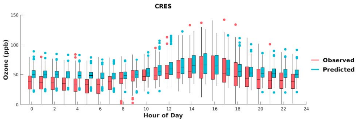
FIGURE F-6: BOX PLOTS OF OBSERVED VS. PREDICTED HOURLY OZONE DURING MAY 1 ST TO SEPTEMBER 30 TH , 2018, AT CRESTLINE. HORIZONTAL LINES INDICATE 25 TH , 50 TH (MEDIAN), AND 75 TH PERCENTILES.
