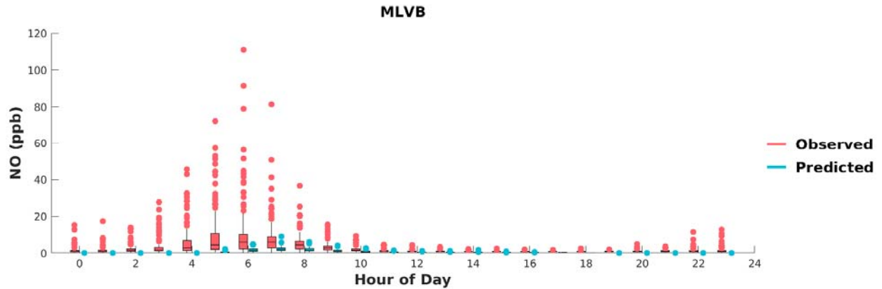
FIGURE G-12: BOX PLOTS OF OBSERVED VS. PREDICTED HOURLY NO DURING MAY 1 ST TO SEPTEMBER 30 TH , 2018, AT MIRA LOMA VAN BUREN. HORIZONTAL LINES INDICATE 25 TH , 50 TH (MEDIAN), AND 75 TH PERCENTILES.
