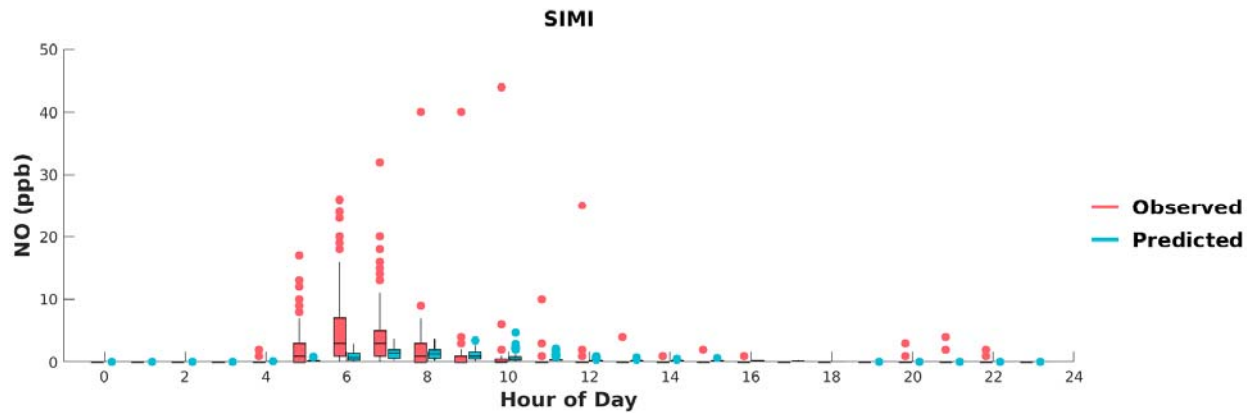
FIGURE G-20: BOX PLOTS OF OBSERVED VS. PREDICTED HOURLY NO DURING MAY 1 ST TO SEPTEMBER 30 TH , 2018, AT SIMI VALLEY. HORIZONTAL LINES INDICATE 25 TH , 50 TH (MEDIAN), AND 75 TH PERCENTILES.
