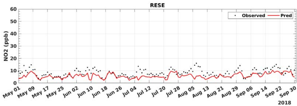
FIGURE C-18: 2018 DAILY AVERAGED NO2 MODEL PREDICTION AND MEASUREMENT COMPARISON AT RESEDA
