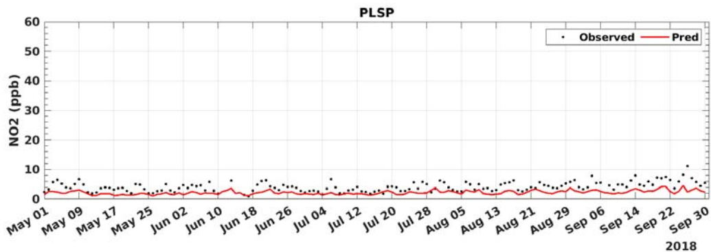
FIGURE C-15: 2018 DAILY AVERAGED NO2 MODEL PREDICTION AND MEASUREMENT COMPARISON AT PALM SPRINGS
