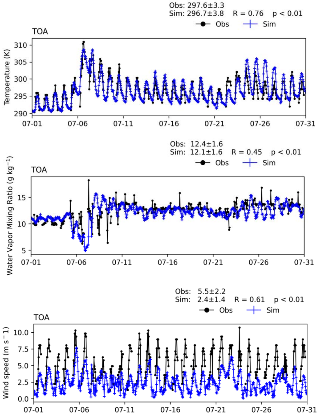
FIGURE V-A22 TIME SERIES OF HOURLY MEASUREMENTS AND WRF BASE SIMULATIONS AT TORRANCE (TOA) FOR JULY 2018
