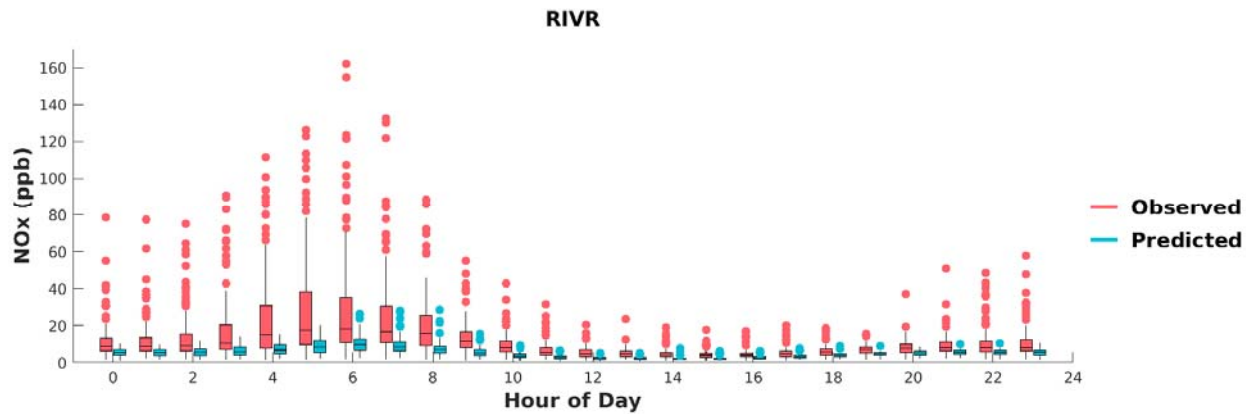
FIGURE I-18: BOX PLOTS OF OBSERVED VS. PREDICTED HOURLY NOX DURING MAY 1 ST TO SEPTEMBER 30 TH , 2018, AT RIVERSIDE. HORIZONTAL LINES INDICATE 25 TH , 50 TH (MEDIAN), AND 75 TH PERCENTILES.
