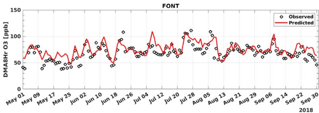
FIGURE A-8: 2018 MAXIMUM DAILY AVERAGE 8-HOUR (MDA8) OZONE MODEL PREDICTION AND MEASUREMENT COMPARISON AT FONTANA
