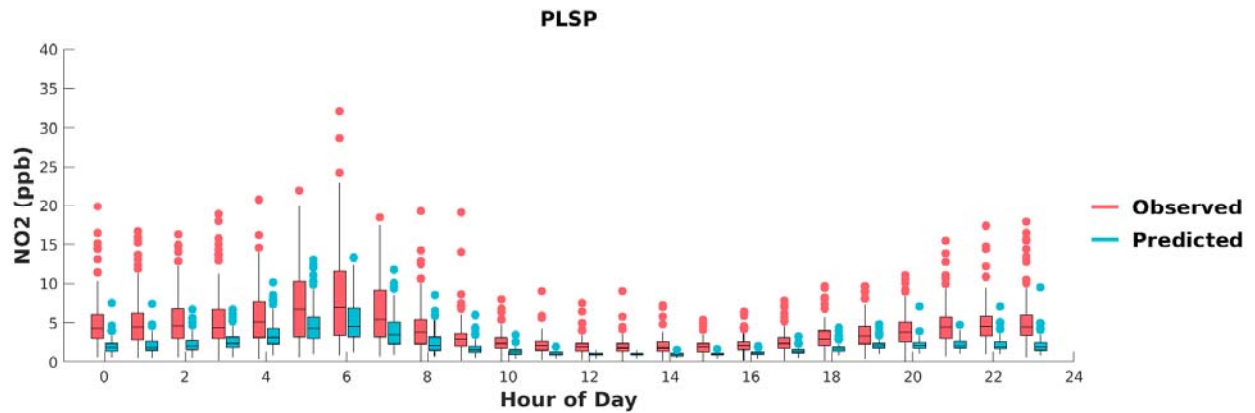
FIGURE H-16: BOX PLOTS OF OBSERVED VS. PREDICTED HOURLY NO 2 DURING MAY 1 ST TO SEPTEMBER 30 TH , 2018, AT PALM SPRINGS. HORIZONTAL LINES INDICATE 25 TH , 50 TH (MEDIAN), AND 75 TH PERCENTILES.
