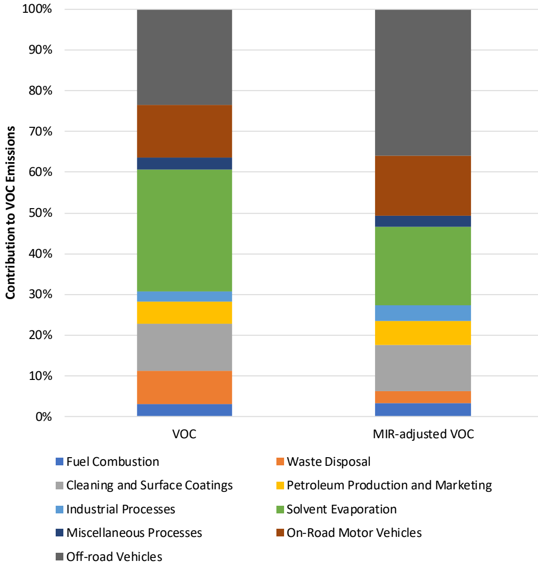
FIGURE V-4-32 CONTRIBUTION TO TOTAL VOC EMISSIONS BY MAJOR SOURCE CATEGORY WITH AND WITHOUT ADJUSTING FOR REACTIVITY, FOR THE YEAR 2018
