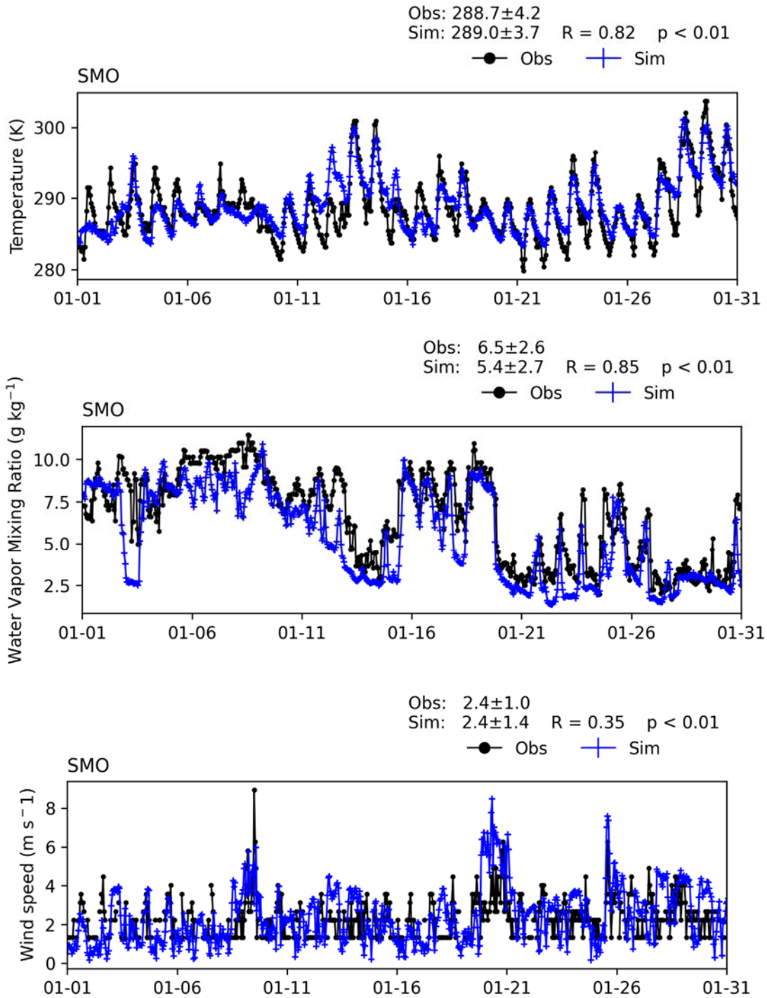
FIGURE V-A17 TIME SERIES OF HOURLY MEASUREMENTS AND WRF BASE SIMULATIONS AT SANTA MONICA AIRPORT (SMO) FOR JANUARY 2018
