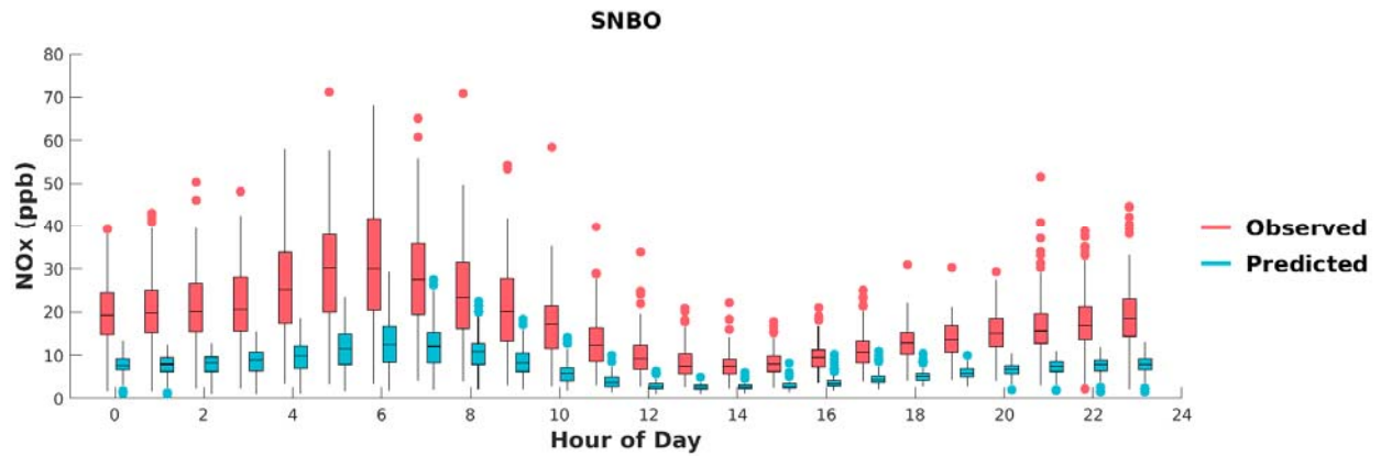
FIGURE I-21: BOX PLOTS OF OBSERVED VS. PREDICTED HOURLY NOx DURING MAY 1 ST TO SEPTEMBER 30 TH , 2018, AT SAN BERNARDINO. HORIZONTAL LINES INDICATE 25 TH , 50 TH (MEDIAN), AND 75 TH PERCENTILES.
