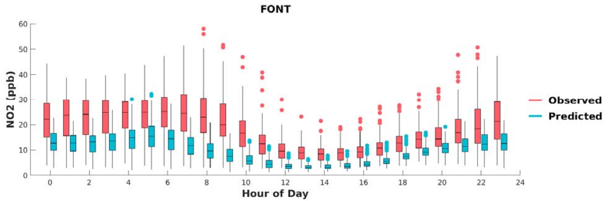
FIGURE H-7: BOX PLOTS OF OBSERVED VS. PREDICTED HOURLY NO 2 DURING MAY 1 ST TO SEPTEMBER 30 TH , 2018, AT FONTANA. HORIZONTAL LINES INDICATE 25 TH , 50 TH (MEDIAN), AND 75 TH PERCENTILES.
