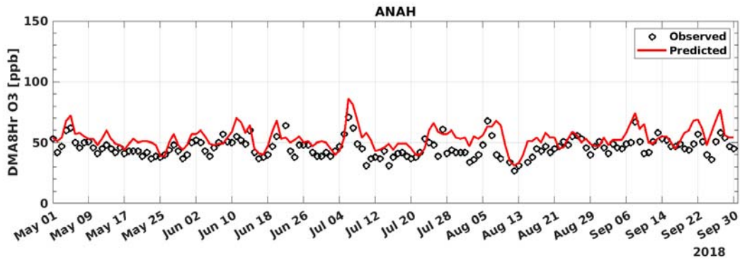
FIGURE A-1: 2018 MAXIMUM DAILY AVERAGE 8-HOUR (MDA8) OZONE MODEL PREDICTION AND MEASUREMENT COMPARISON AT ANAHEIM
