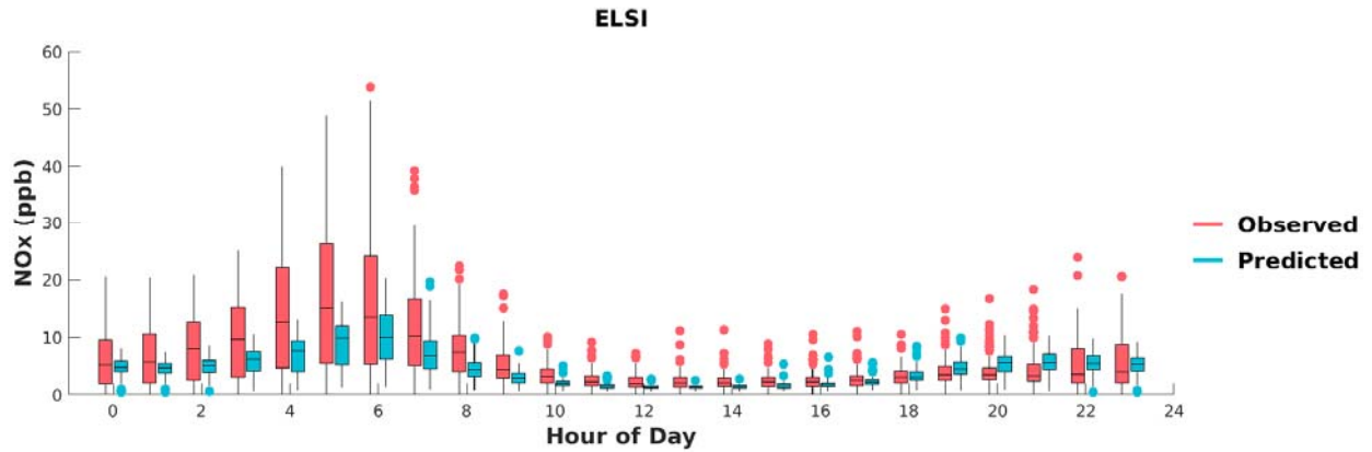
FIGURE I-6: BOX PLOTS OF OBSERVED VS. PREDICTED HOURLY NOX DURING MAY 1 ST TO SEPTEMBER 30 TH , 2018, AT LAKE ELSINORE. HORIZONTAL LINES INDICATE 25 TH , 50 TH (MEDIAN), AND 75 TH PERCENTILES.
