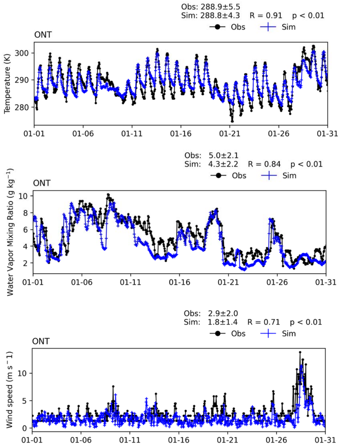
FIGURE V-A9 TIME SERIES OF HOURLY MEASUREMENTS AND WRF BASE SIMULATIONS AT ONTARIO INTERNATIONAL AIRPORT (ONT) FOR JANUARY 2018
