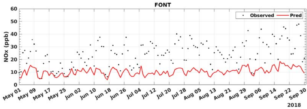
FIGURE D-7: 2018 DAILY AVERAGED NOX MODEL PREDICTION AND MEASUREMENT COMPARISON AT FONTANA
