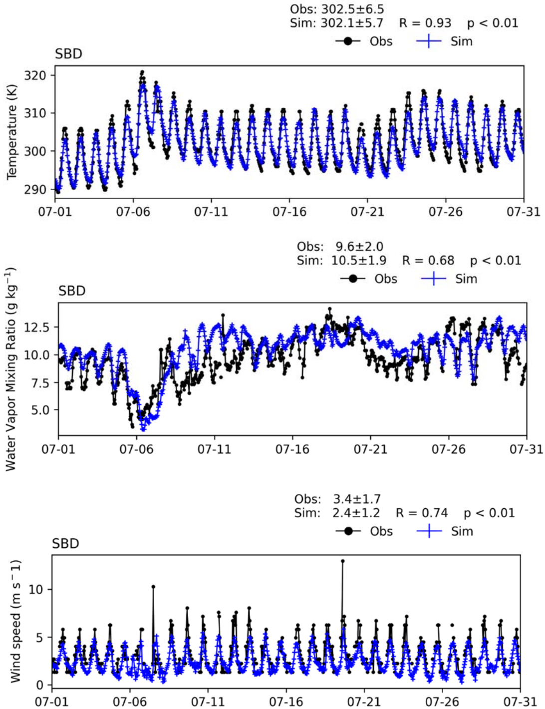
FIGURE V-A16 TIME SERIES OF HOURLY MEASUREMENTS AND WRF BASE SIMULATIONS AT SAN BERNARDINO INTERNATIONAL AIRPORT (SBD) FOR JULY 2018
