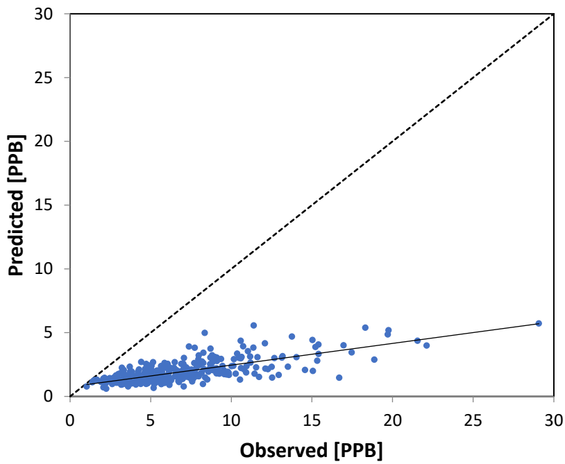
Figure 8. Scatter Plot of Predicted vs. Observed Concentrations Acetone
