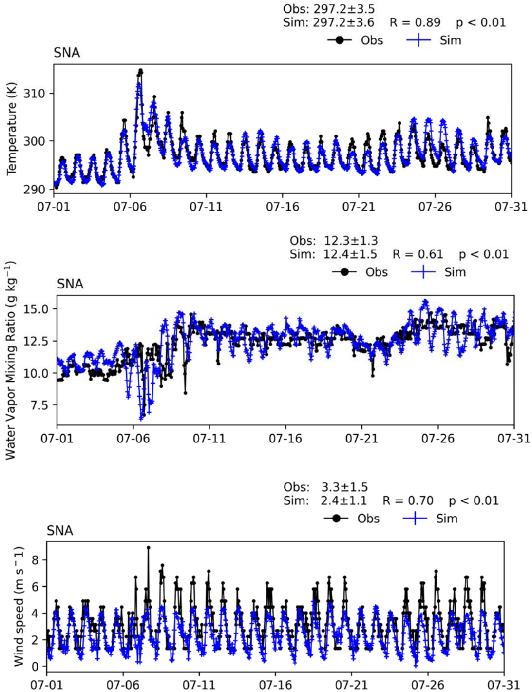
FIGURE V-A20 TIME SERIES OF HOURLY MEASUREMENTS AND WRF BASE SIMULATIONS AT SANTA ANA JOHN WAYNE AIRPORT (SNA) FOR JULY 2018
