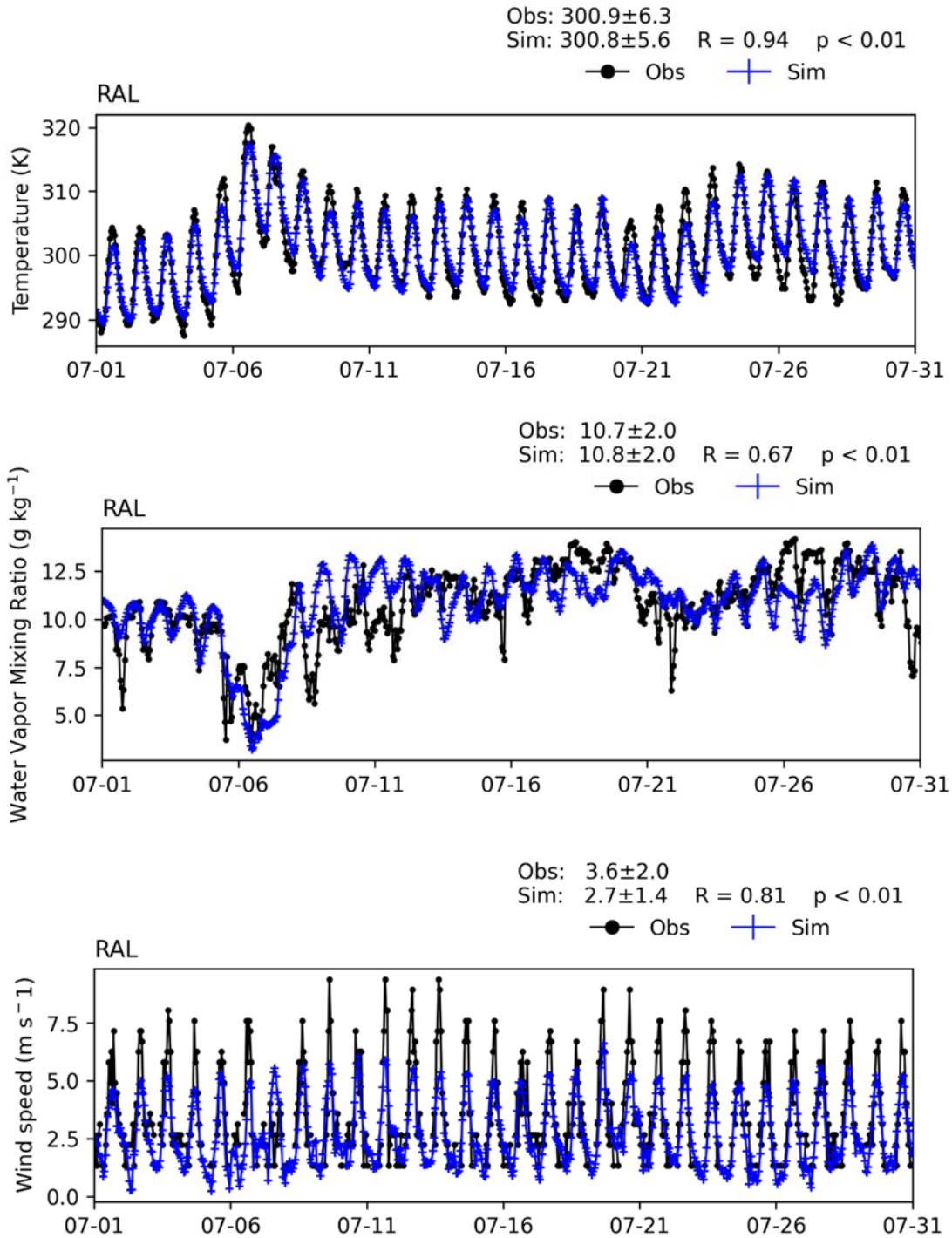
FIGURE V-A12 TIME SERIES OF HOURLY MEASUREMENTS AND WRF BASE SIMULATIONS AT RIVERSIDE MUNICIPAL AIRPORT (RAL) FOR JULY 2018
