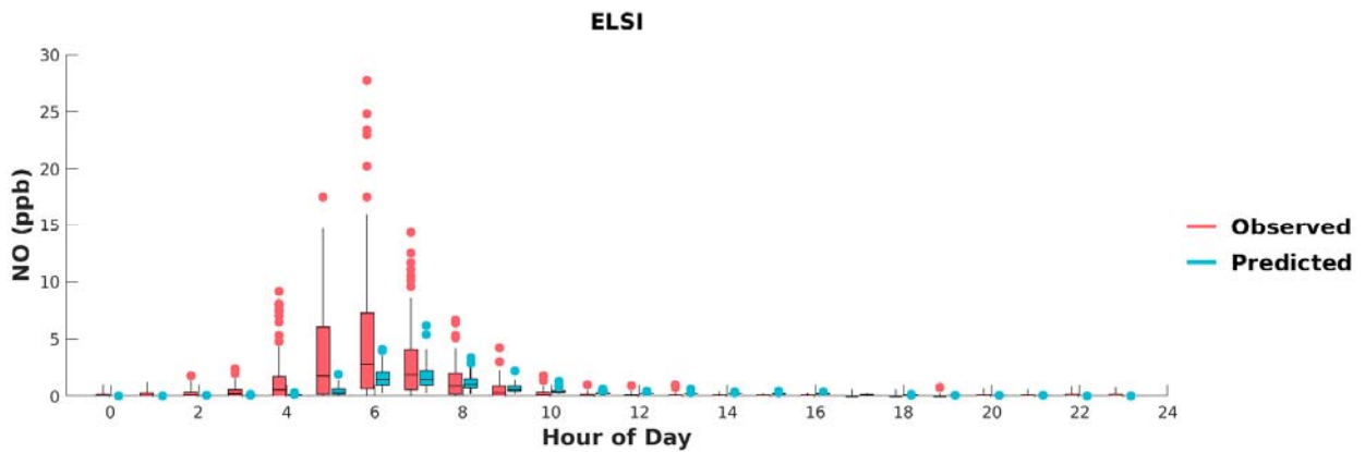
FIGURE G-6: BOX PLOTS OF OBSERVED VS. PREDICTED HOURLY NO DURING MAY 1 ST TO SEPTEMBER 30 TH , 2018, AT LAKE ELSINORE. HORIZONTAL LINES INDICATE 25 TH , 50 TH (MEDIAN), AND 75 TH PERCENTILES.
