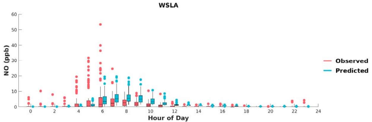
FIGURE G-23: BOX PLOTS OF OBSERVED VS. PREDICTED HOURLY NO DURING MAY 1 ST TO SEPTEMBER 30 TH , 2018, AT WEST LOS ANGELES. HORIZONTAL LINES INDICATE 25 TH , 50 TH (MEDIAN), AND 75 TH PERCENTILES.
