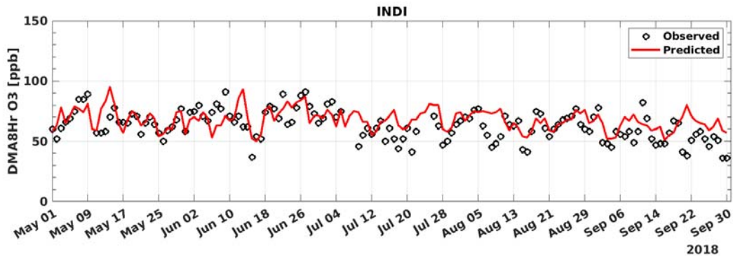
FIGURE A-10: 2018 MAXIMUM DAILY AVERAGE 8-HOUR (MDA8) OZONE MODEL PREDICTION AND MEASUREMENT COMPARISON AT INDI
