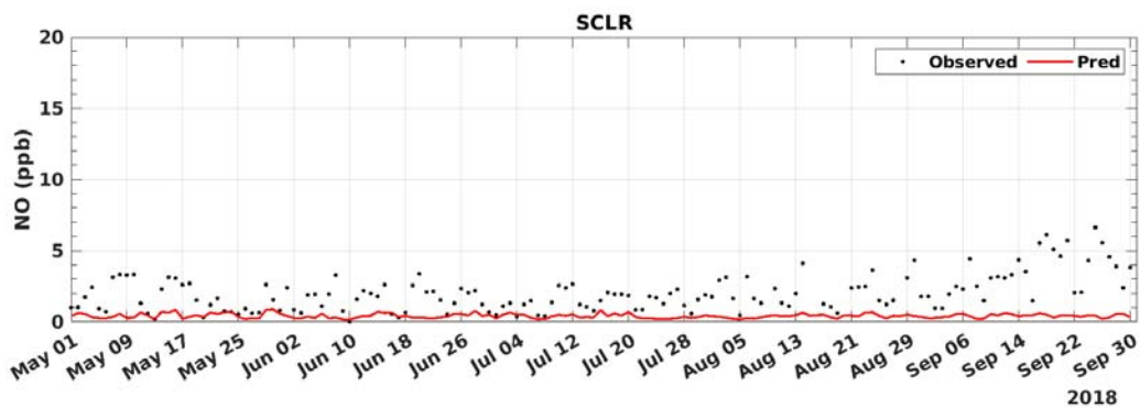
FIGURE B-23: 2018 DAILY AVERAGED NO MODEL PREDICTION AND MEASUREMENT COMPARISON AT SANTA CLARITA
