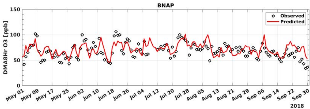
FIGURE A-3: 2018 MAXIMUM DAILY AVERAGE 8-HOUR (MDA8) OZONE MODEL PREDICTION AND MEASUREMENT COMPARISON AT BANNING
