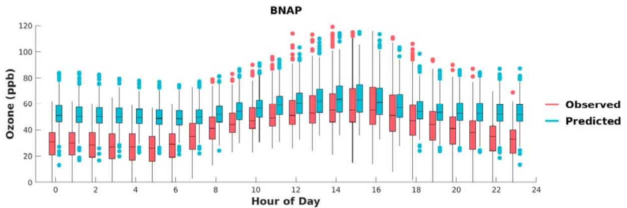
FIGURE F-3: BOX PLOTS OF OBSERVED VS. PREDICTED HOURLY OZONE DURING MAY 1 ST TO SEPTEMBER 30 TH , 2018, AT BANNING. HORIZONTAL LINES INDICATE 25 TH , 50 TH (MEDIAN), AND 75 TH PERCENTILES.
