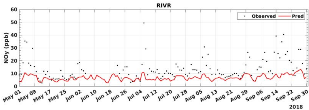
FIGURE E-2: 2018 DAILY AVERAGED NOY MODEL PREDICTION AND MEASUREMENT COMPARISON AT RIVERSIDE
