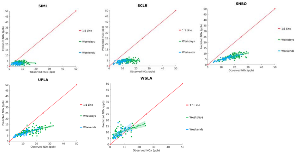
FIGURE N-4: SCATTER PLOT OF OBSERVED VS. PREDICTED DAILY AVERAGE NOX DURING MAY 1 ST TO SEPTEMBER 30 TH , 2018, AT SIMI VALLEY (SIMI), SANTA CLARITA (SCLR), SAN BERNARDION (SNBO),
