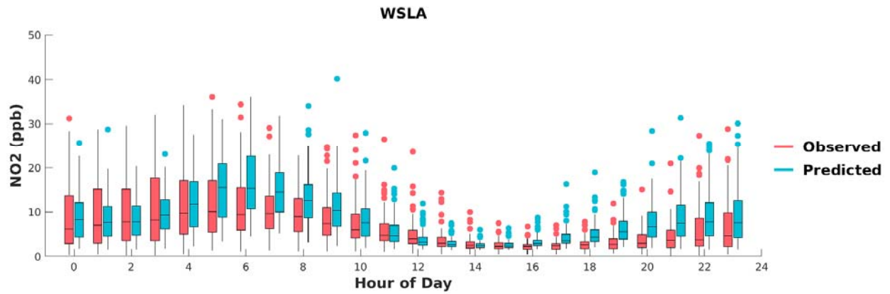
FIGURE H-23: BOX PLOTS OF OBSERVED VS. PREDICTED HOURLY NO 2 DURING MAY 1 ST TO SEPTEMBER 30 TH , 2018, AT WEST LOS ANGELES. HORIZONTAL LINES INDICATE 25 TH , 50 TH (MEDIAN), AND 75 TH PERCENTILES.
