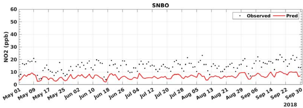
FIGURE C-21: 2018 DAILY AVERAGED NO2 MODEL PREDICTION AND MEASUREMENT COMPARISON AT SAN BERNARDINO
