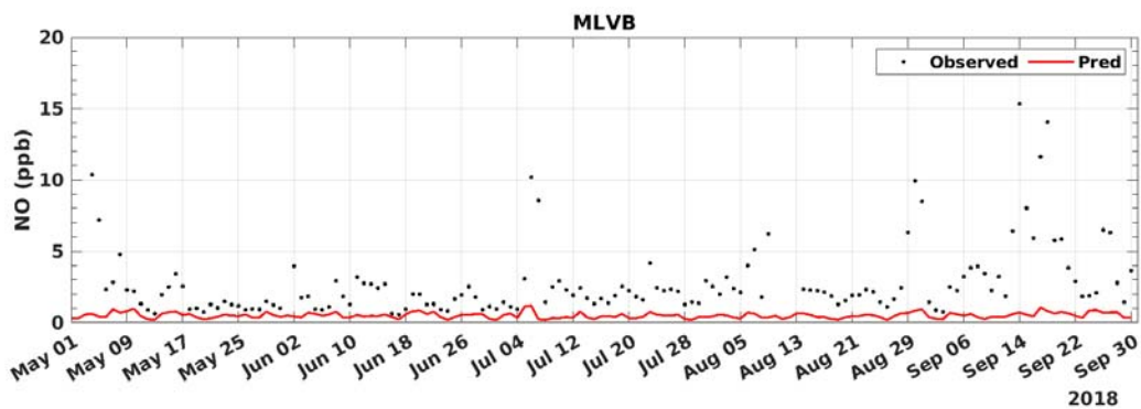
FIGURE B-14: 2018 DAILY AVERAGED NO MODEL PREDICTION AND MEASUREMENT COMPARISON AT MIRA LOMA VAN BUREN
