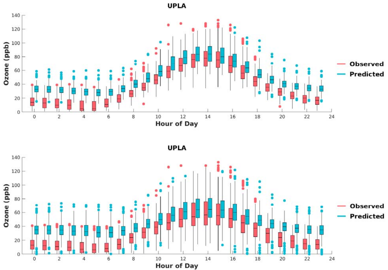
FIGURE F-29: BOX PLOTS OF OBSERVED VS. PREDICTED HOURLY OZONE DURING MAY 1 ST TO SEPTEMBER 30 TH , 2018, AT UPLAND. HORIZONTAL LINES INDICATE 25 TH , 50 TH (MEDIAN), AND 75 TH PERCENTILES.
