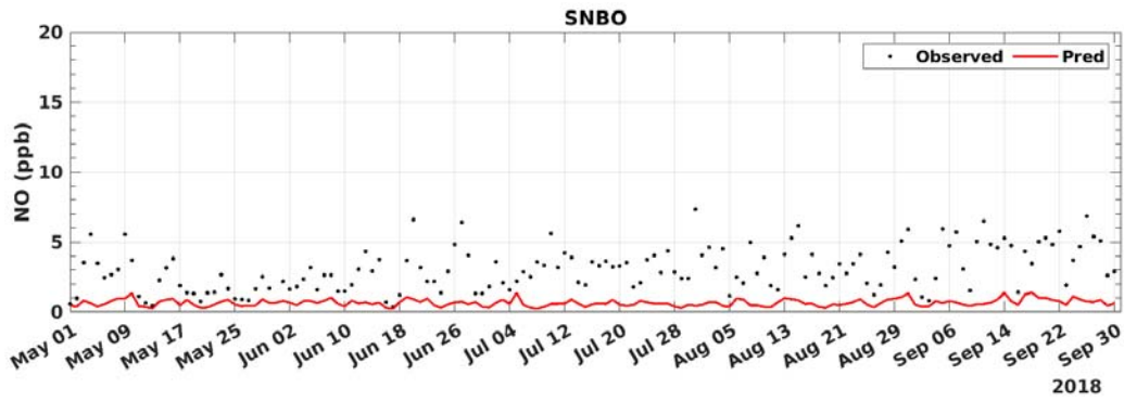
FIGURE B-25: 2018 DAILY AVERAGED NO MODEL PREDICTION AND MEASUREMENT COMPARISON AT SAN BERNARDINO
