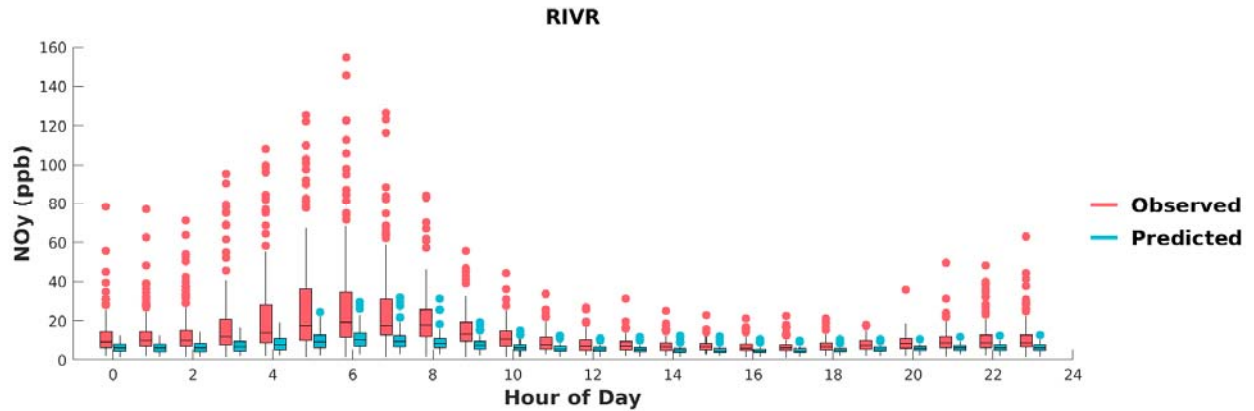
FIGURE J-1: BOX PLOTS OF OBSERVED VS. PREDICTED HOURLY NO y DURING MAY 1 ST TO SEPTEMBER 30 TH , 2018, AT RIVERSIDE. HORIZONTAL LINES INDICATE 25 TH , 50 TH (MEDIAN), AND 75 TH PERCENTILES.
