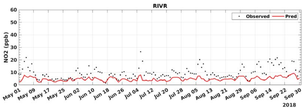
FIGURE C-17: 2018 DAILY AVERAGED NO2 MODEL PREDICTION AND MEASUREMENT COMPARISON AT RIVERSIDE
