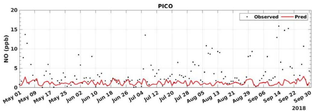
FIGURE B-17: 2018 DAILY AVERAGED NO MODEL PREDICTION AND MEASUREMENT COMPARISON AT PICO RIVERA
