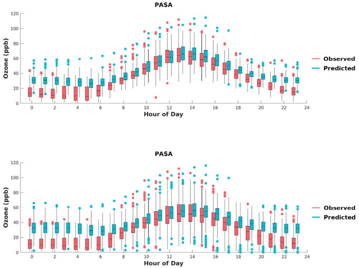
FIGURE F-17: BOX PLOTS OF OBSERVED VS. PREDICTED HOURLY OZONE DURING MAY 1 ST TO SEPTEMBER 30 TH , 2018, AT PASADENA. HORIZONTAL LINES INDICATE 25 TH , 50 TH (MEDIAN), AND 75 TH PERCENTILES.
