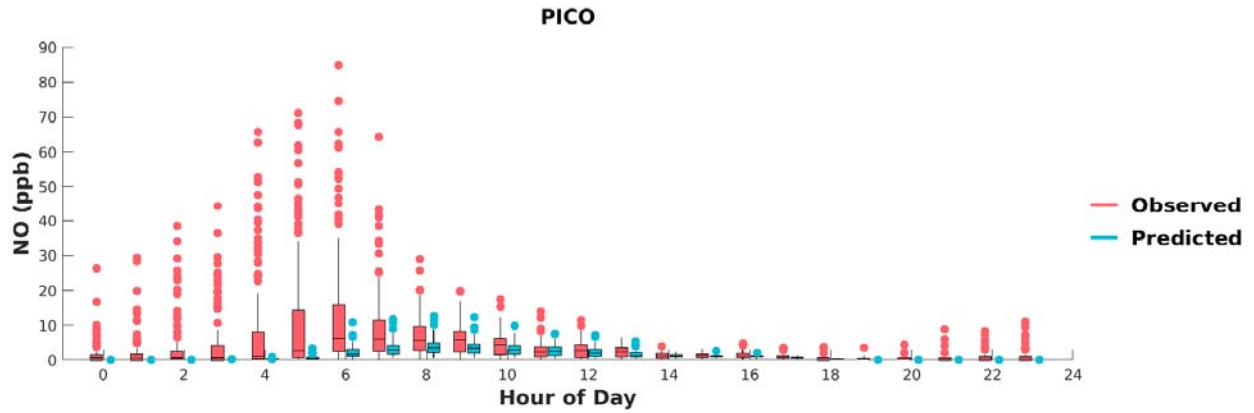
FIGURE G-14: BOX PLOTS OF OBSERVED VS. PREDICTED HOURLY NO DURING MAY 1 ST TO SEPTEMBER 30 TH , 2018, AT PICO RIVERO. HORIZONTAL LINES INDICATE 25 TH , 50 TH (MEDIAN), AND 75 TH PERCENTILES.
