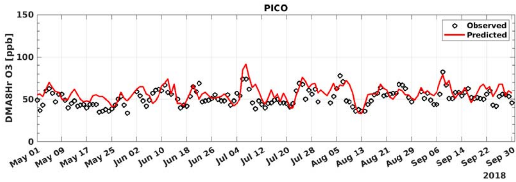
FIGURE A-19: 2018 MAXIMUM DAILY AVERAGE 8-HOUR (MDA8) OZONE MODEL PREDICTION AND MEASUREMENT COMPARISON AT PICO RIVERA
