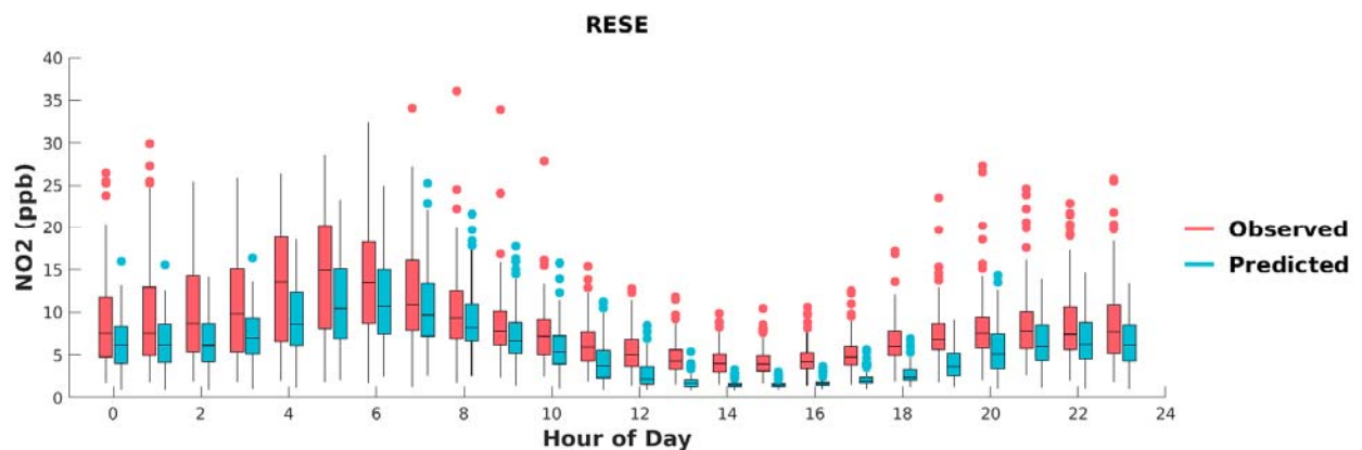
FIGURE H-17: BOX PLOTS OF OBSERVED VS. PREDICTED HOURLY NO 2 DURING MAY 1 ST TO SEPTEMBER 30 TH , 2018, AT RESEDA. HORIZONTAL LINES INDICATE 25 TH , 50 TH (MEDIAN), AND 75 TH PERCENTILES.
