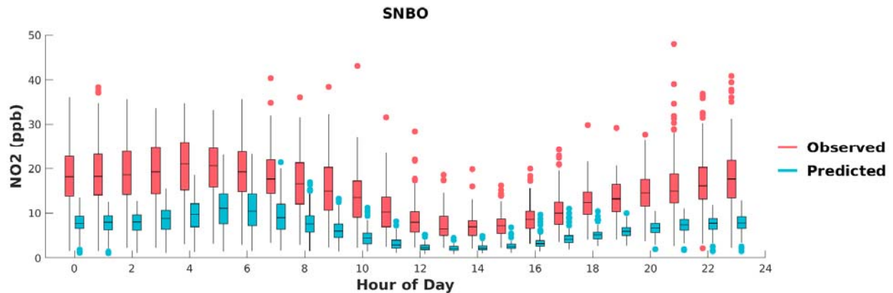
FIGURE H-21: BOX PLOTS OF OBSERVED VS. PREDICTED HOURLY NO 2 DURING MAY 1 ST TO SEPTEMBER 30 TH , 2018, AT SAN BERNARDINO. HORIZONTAL LINES INDICATE 25 TH , 50 TH (MEDIAN), AND 75 TH PERCENTILES.
