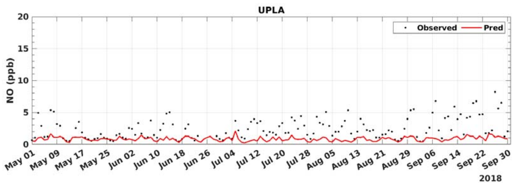
FIGURE B-26: 2018 DAILY AVERAGED NO MODEL PREDICTION AND MEASUREMENT COMPARISON AT UPLAND
