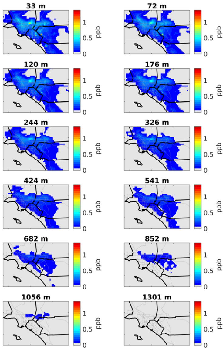
Figure 147: Vertical cross-sections of toluene during July 2018. Heights correspond to the top of each layer.
