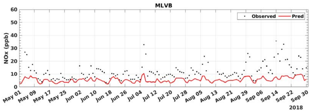
FIGURE D-12: 2018 DAILY AVERAGED NOX MODEL PREDICTION AND MEASUREMENT COMPARISON AT MIRA LOMA VAN BUREN
