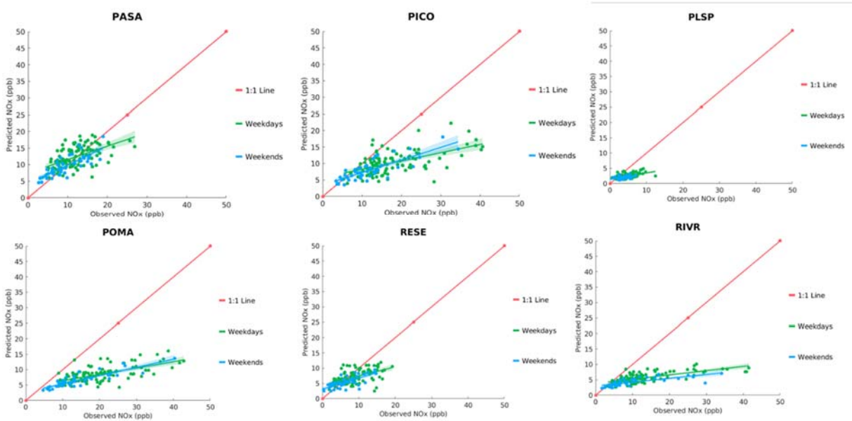
FIGURE N-3: SCATTER PLOT OF OBSERVED VS. PREDICTED DAILY AVERAGE NOX DURING MAY 1 ST TO SEPTEMBER 30 TH , 2018, AT PASADENA (PASA), PICO RIVERO (PICO), PALM SPRINGS (PLSP), POMONA (POMA), RESEDA (RESE), AND RIVERSIDE (RIVR). GREEN AND BLUE LINES INDICATE GENERAL LINEAR MODEL FIT WITH 95% CONFIDENCE INTERVAL (SHADED AREA). THE RED LINE INDICATES 1:1 LINE.
