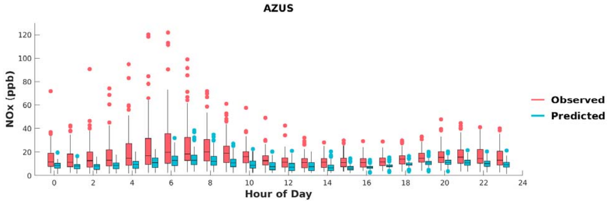
FIGURE I-2: BOX PLOTS OF OBSERVED VS. PREDICTED HOURLY NOX DURING MAY 1 ST TO SEPTEMBER 30 TH , 2018, AT AZUSA. HORIZONTAL LINES INDICATE 25 TH , 50 TH (MEDIAN), AND 75 TH PERCENTILES.
