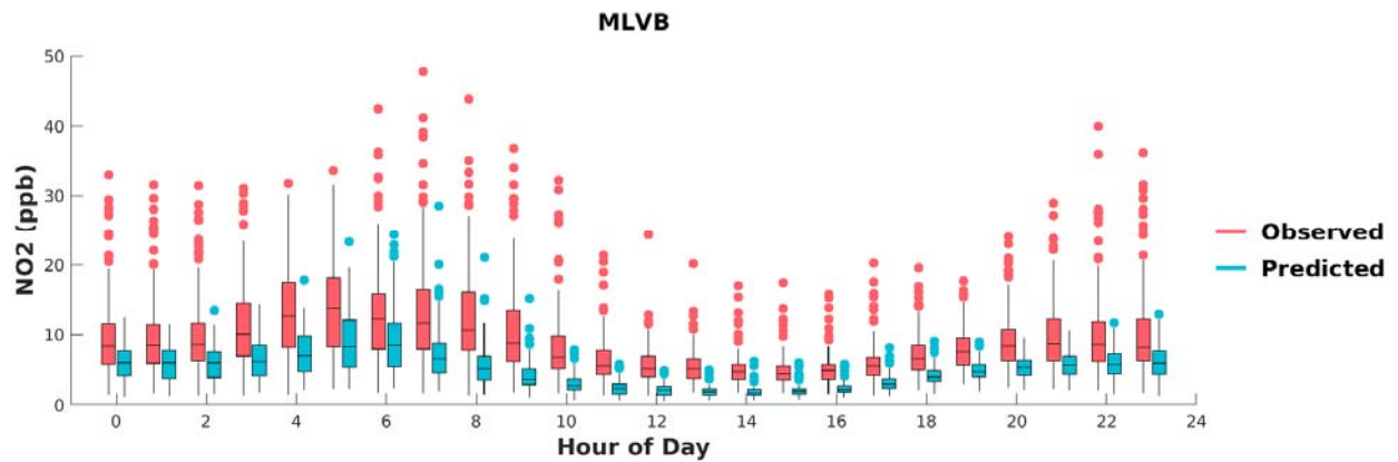
FIGURE H-12: BOX PLOTS OF OBSERVED VS. PREDICTED HOURLY NO2 DURING MAY 1 ST TO SEPTEMBER 30 TH , 2018, AT MIRA LOMA VAN BUREN. HORIZONTAL LINES INDICATE 25 TH , 50 TH (MEDIAN), AND 75 TH PERCENTILES.
