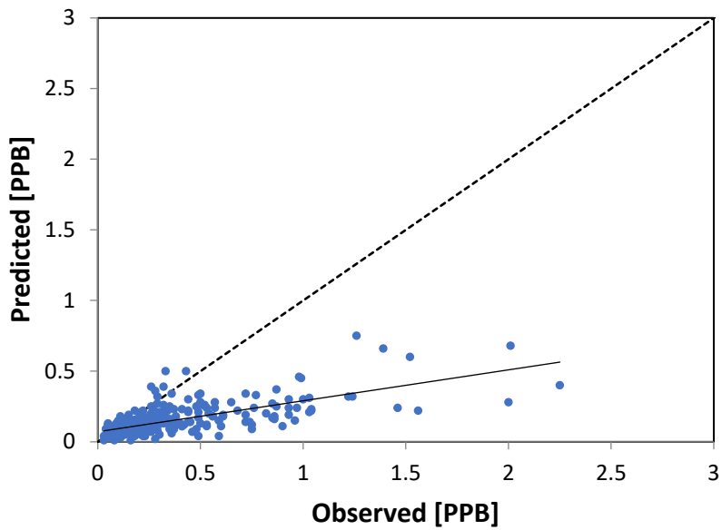
Figure 9. Scatter Plot of Predicted vs. Observed Concentrations m&p-Xylene
