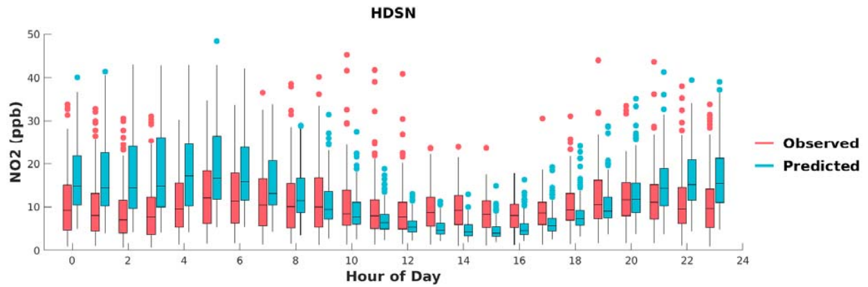
FIGURE H-9: BOX PLOTS OF OBSERVED VS. PREDICTED HOURLY NO 2 DURING MAY 1 ST TO SEPTEMBER 30 TH , 2018, AT HUDSON. HORIZONTAL LINES INDICATE 25 TH , 50 TH (MEDIAN), AND 75 TH PERCENTILES.
