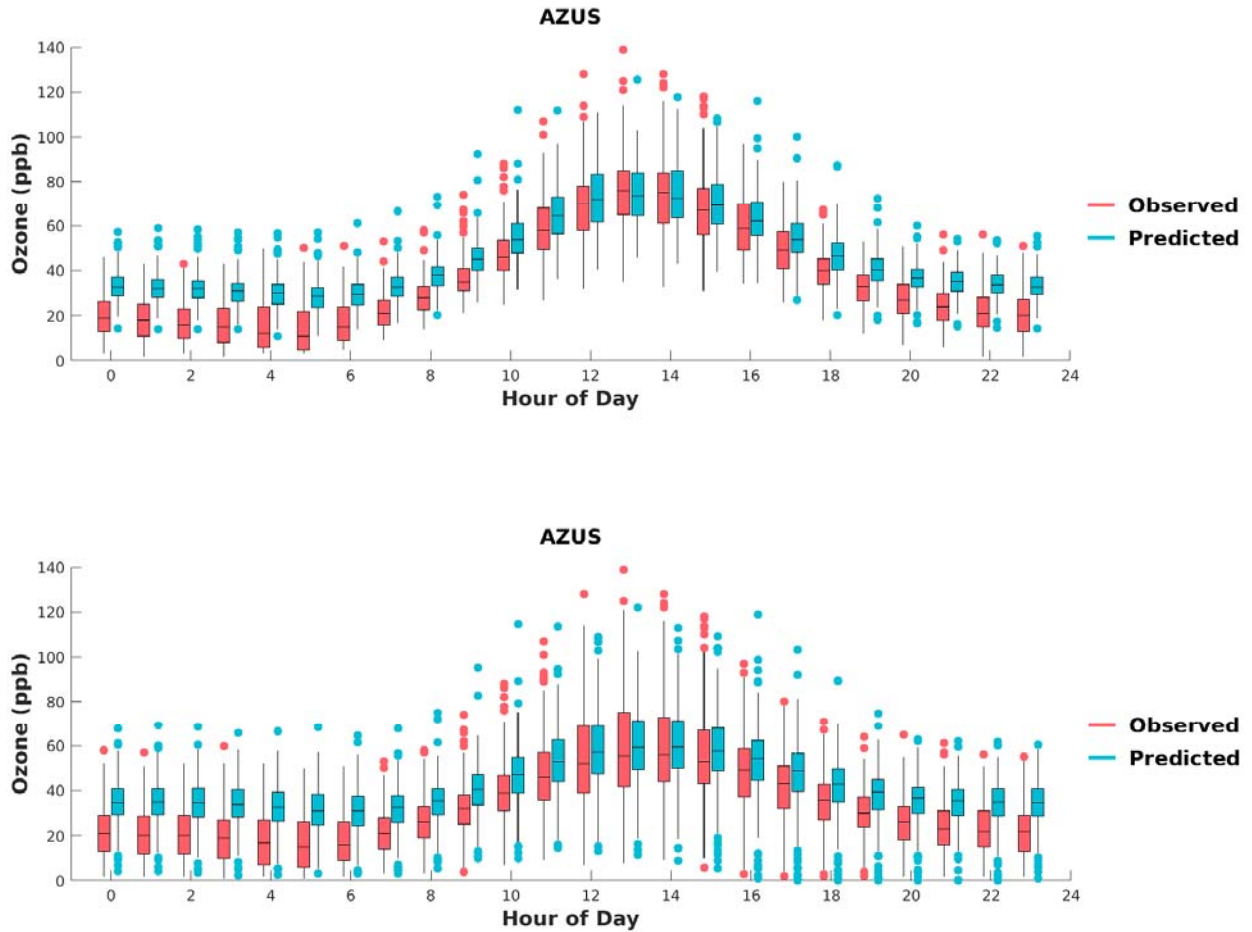
FIGURE F-2: BOX PLOTS OF OBSERVED VS. PREDICTED HOURLY OZONE DURING MAY 1 ST TO SEPTEMBER 30 TH , 2018, AT AZUSA. HORIZONTAL LINES INDICATE 25 TH , 50 TH (MEDIAN), AND 75 TH PERCENTILES.
