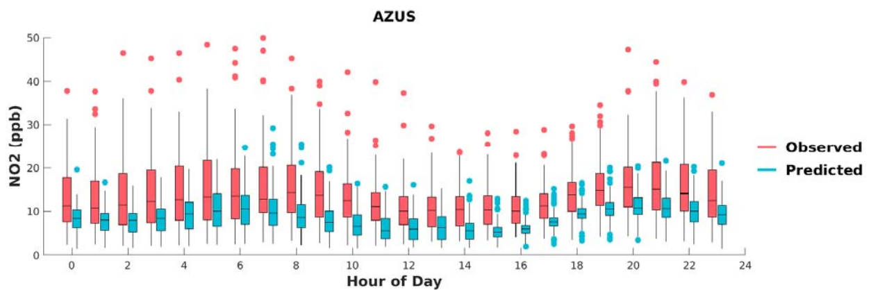
FIGURE H-2: BOX PLOTS OF OBSERVED VS. PREDICTED HOURLY NO2 DURING MAY 1 ST TO SEPTEMBER 30 TH , 2018, AT AZUSA. HORIZONTAL LINES INDICATE 25 TH , 50 TH (MEDIAN), AND 75 TH PERCENTILES.
