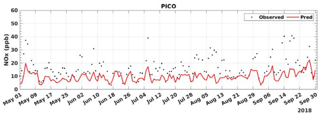
FIGURE D-14: 2018 DAILY AVERAGED NOX MODEL PREDICTION AND MEASUREMENT COMPARISON AT PICO RIVERA
