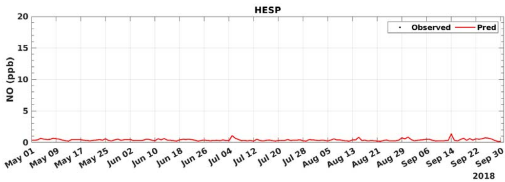
FIGURE B-11: 2018 DAILY AVERAGED NO MODEL PREDICTION AND MEASUREMENT COMPARISON AT HESPERIA
