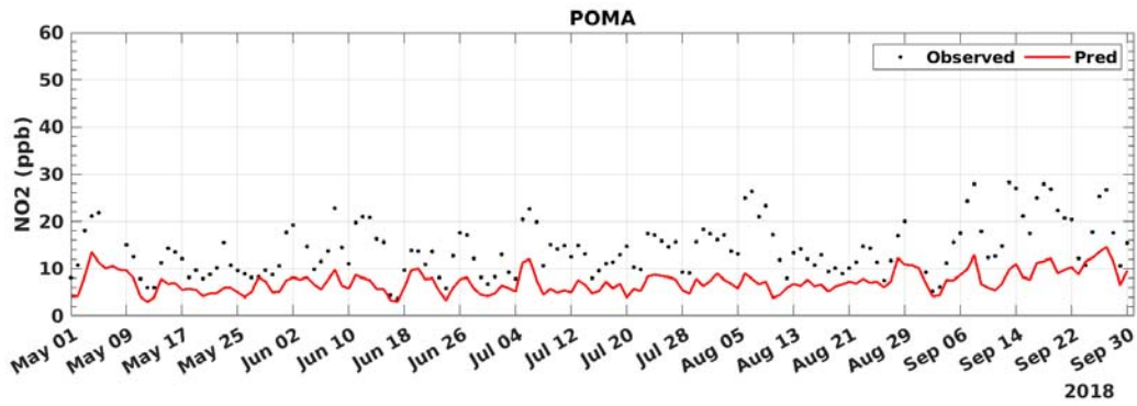
FIGURE C-16: 2018 DAILY AVERAGED NO2 MODEL PREDICTION AND MEASUREMENT COMPARISON AT POMONA
