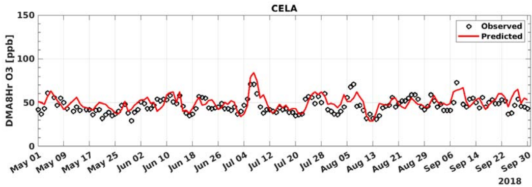
FIGURE A-4: 2018 MAXIMUM DAILY AVERAGE 8-HOUR (MDA8) OZONE MODEL PREDICTION AND MEASUREMENT COMPARISON AT CENTRAL LOS ANGELES
