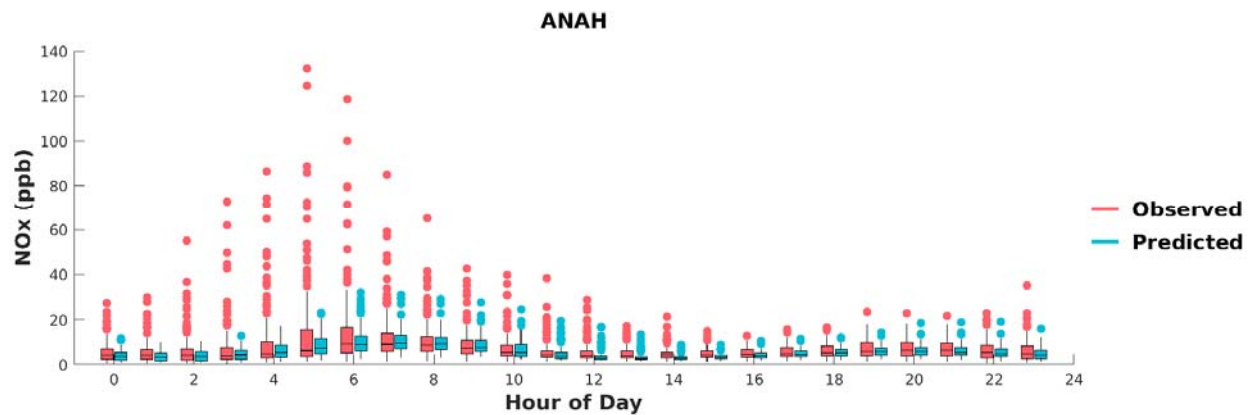
FIGURE I-1: BOX PLOTS OF OBSERVED VS. PREDICTED HOURLY NO x DURING MAY 1 ST TO SEPTEMBER 30 TH , 2018, AT ANAHEIM. HORIZONTAL LINES INDICATE 25 TH , 50 TH (MEDIAN), AND 75 TH PERCENTILES.
