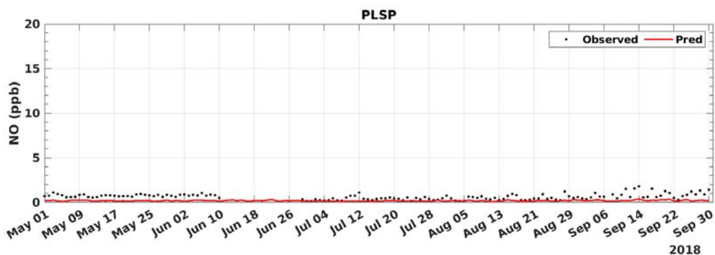
FIGURE B-18: 2018 DAILY AVERAGED NO MODEL PREDICTION AND MEASUREMENT COMPARISON AT PALM SPRINGS
