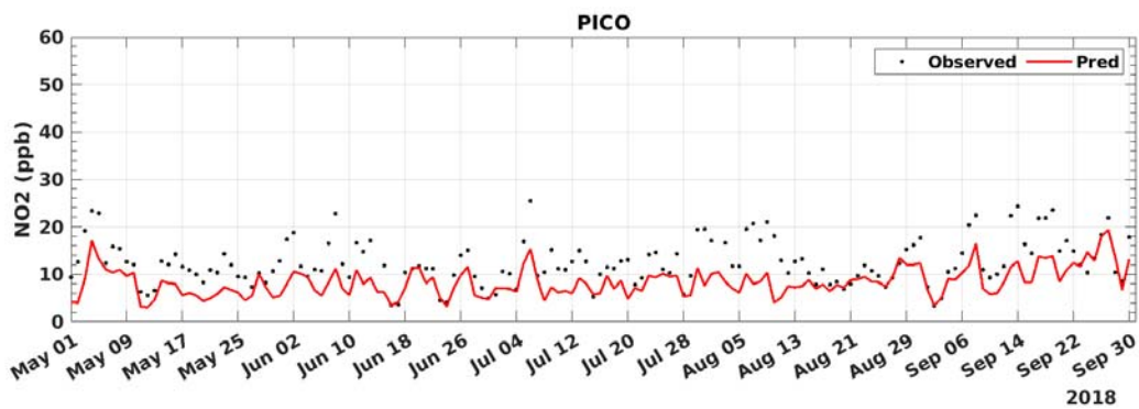
FIGURE C-14: 2018 DAILY AVERAGED NO2 MODEL PREDICTION AND MEASUREMENT COMPARISON AT PICO RIVERA
