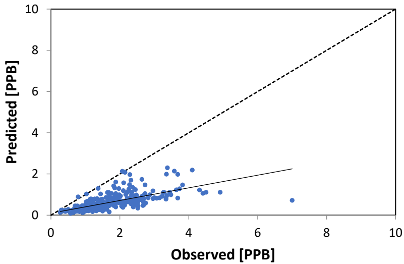
Figure 7. Scatter Plot of Predicted vs. Observed Concentrations Acetaldehyde
