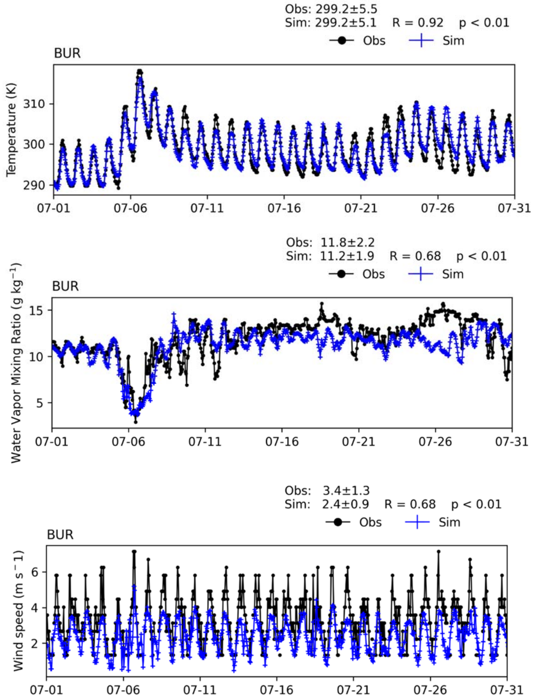
FIGURE V-A2 TIME SERIES OF HOURLY MEASUREMENTS AND WRF BASE SIMULATIONS AT BURBANK AIRPORT (BUR) FOR JULY 2018
