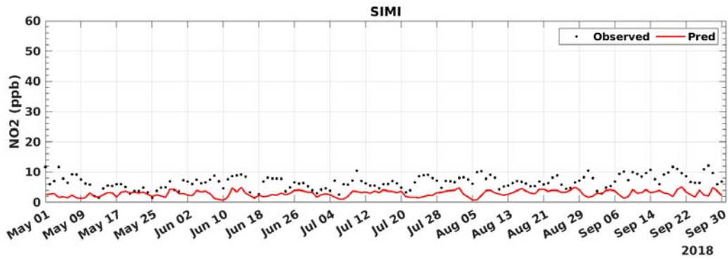
FIGURE C-19: 2018 DAILY AVERAGED NO2 MODEL PREDICTION AND MEASUREMENT COMPARISON AT SIMI VALLEY
