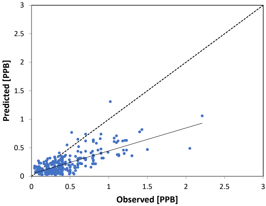
Figure 10. Scatter Plot of Predicted vs. Observed Concentrations Propylene
