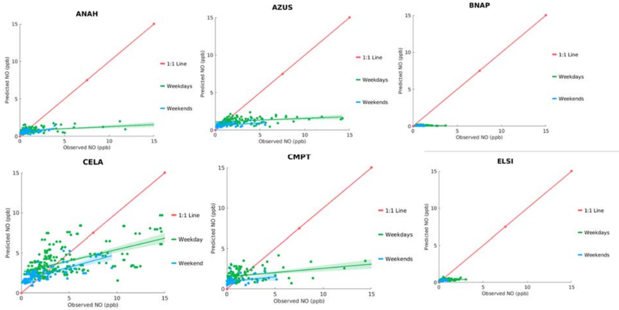
FIGURE L-1: SCATTER PLOT OF OBSERVED VS. PREDICTED DAILY AVERAGE NO DURING MAY 1 ST TO SEPTEMBER 30 TH , 2018, AT ANEHIM (ANAH), AZUSA (AZUS), BANNING (BANP), COMPTON (CMPT), CENTRAL LOS ANGELES (CELA), AND LAKE ELSINORE (ELSI). GREEN AND BLUE LINES INDICATE GENERAL LINEAR MODEL FIT WITH 95% CONFIDENCE INTERVAL (SHADED AREA). THE RED LINE INDICATES 1:1 LINE.
