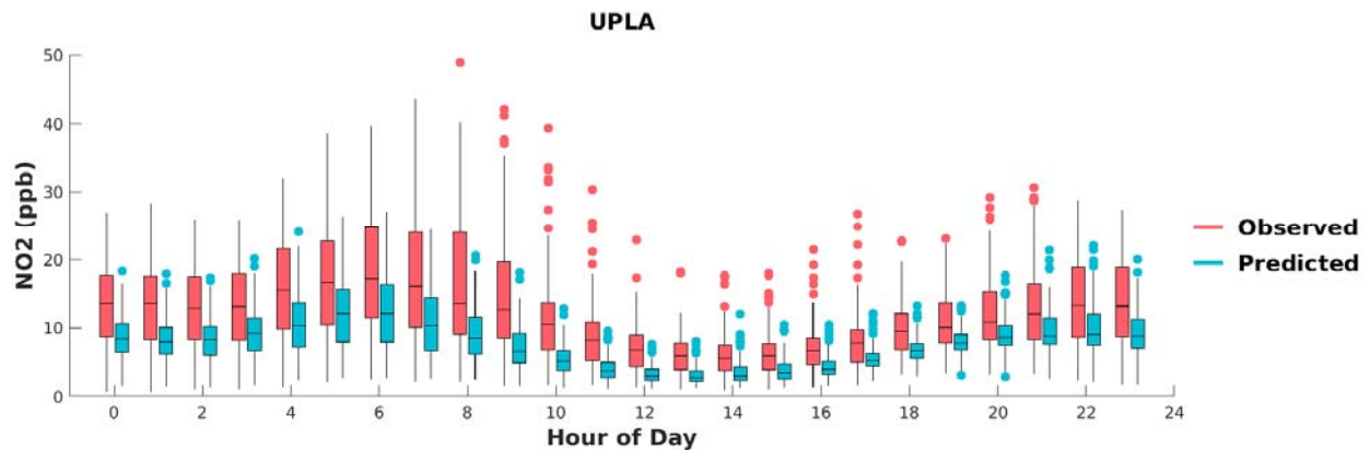
FIGURE H-22: BOX PLOTS OF OBSERVED VS. PREDICTED HOURLY NO 2 DURING MAY 1 ST TO SEPTEMBER 30 TH , 2018, AT UPLAND. HORIZONTAL LINES INDICATE 25 TH , 50 TH (MEDIAN), AND 75 TH PERCENTILES.
