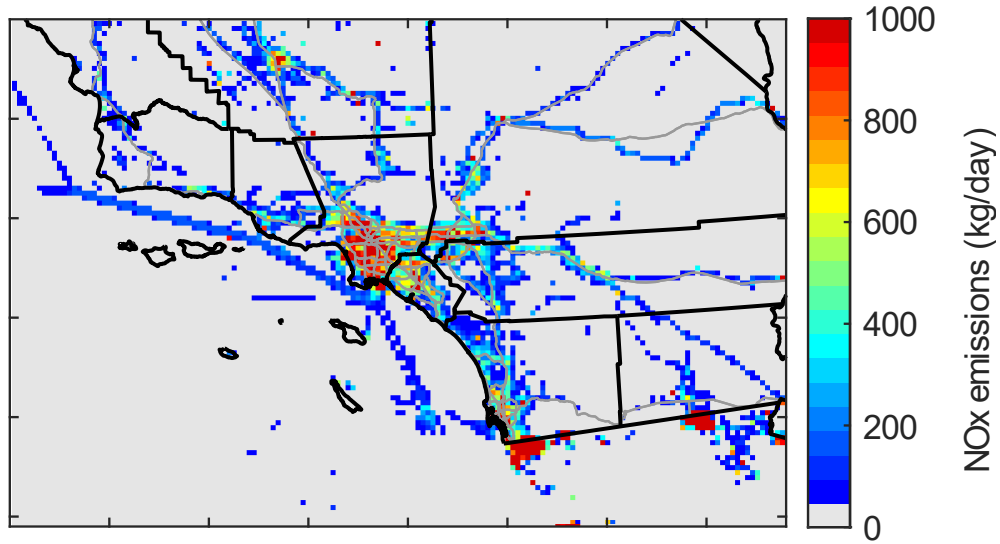
FIGURE V-4-17 SUMMER AVERAGE NO x EMISSIONS IN THE MODELING DOMAIN
