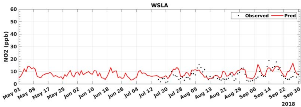
FIGURE C-23: 2018 DAILY AVERAGED NO2 MODEL PREDICTION AND MEASUREMENT COMPARISON AT WEST LOS ANGELES
