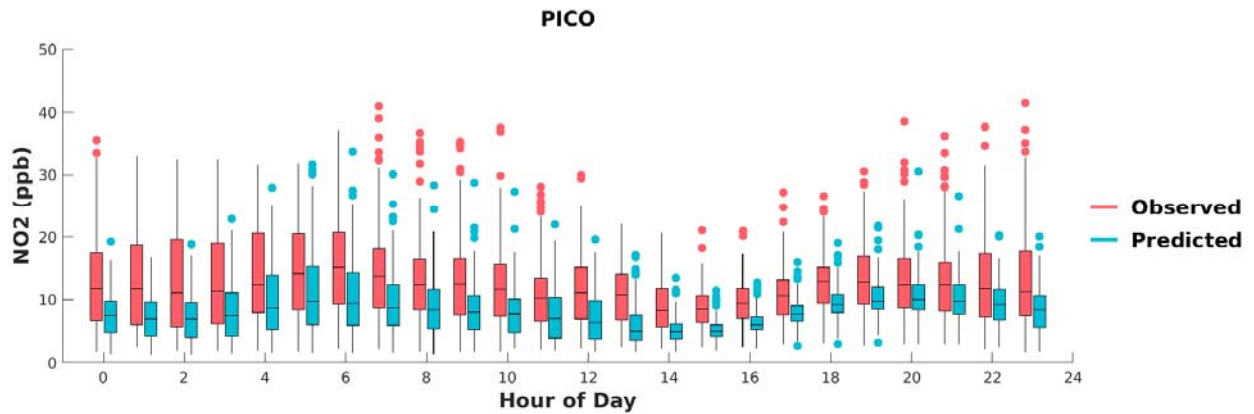
FIGURE H-14: BOX PLOTS OF OBSERVED VS. PREDICTED HOURLY NO 2 DURING MAY 1 ST TO SEPTEMBER 30 TH , 2018, AT PICO RIVERO. HORIZONTAL LINES INDICATE 25 TH , 50 TH (MEDIAN), AND 75 TH PERCENTILES.
