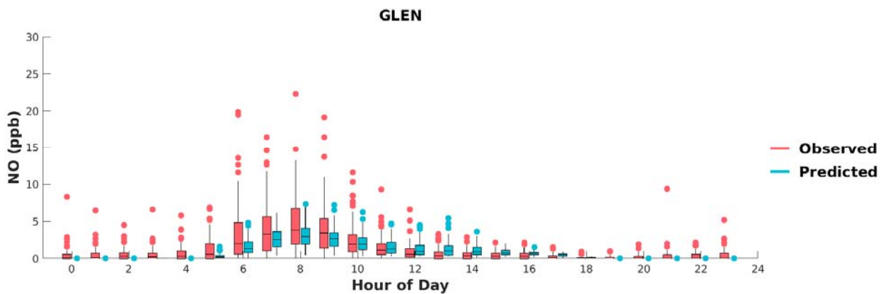
FIGURE G-8: BOX PLOTS OF OBSERVED VS. PREDICTED HOURLY NO DURING MAY 1 ST TO SEPTEMBER 30 TH , 2018, AT GLEN DORA. HORIZONTAL LINES INDICATE 25 TH , 50 TH (MEDIAN), AND 75 TH PERCENTILES.
