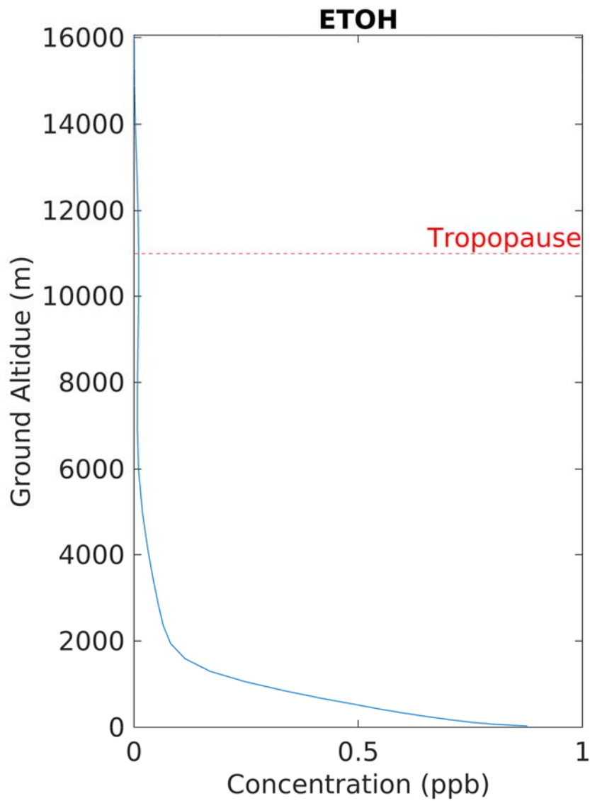
Figure 6: Vertical profile of ethanol averaged over the Basin during July 2018
