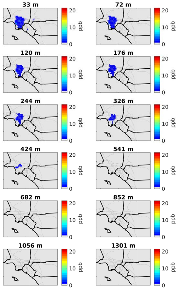
Figure 87: Vertical cross-sections of NO during July 2018. Heights correspond to the top of each layer.
