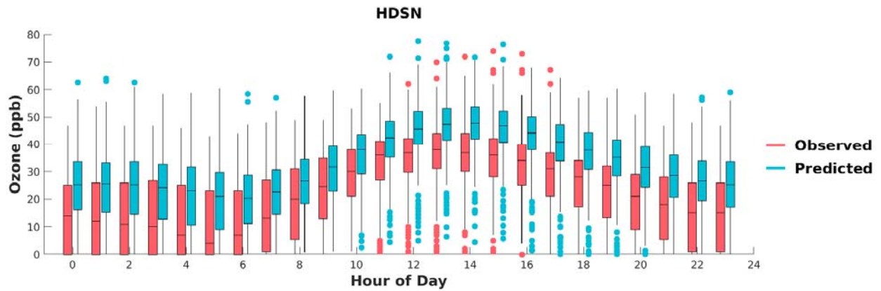
FIGURE F-10: BOX PLOTS OF OBSERVED VS. PREDICTED HOURLY OZONE DURING MAY 1 ST TO SEPTEMBER 30 TH , 2018, AT HUDSON. HORIZONTAL LINES INDICATE 25 TH , 50 TH (MEDIAN), AND 75 TH PERCENTILES.
