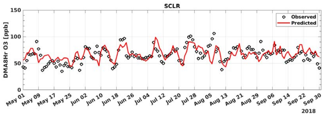
FIGURE A-23: 2018 MAXIMUM DAILY AVERAGE 8-HOUR (MDA8) OZONE MODEL PREDICTION AND MEASUREMENT COMPARISON AT SANTA CLARITA
