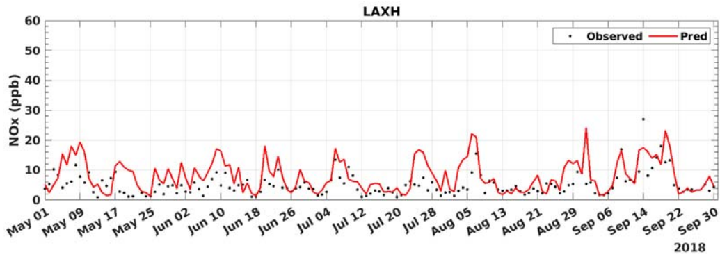
FIGURE D-10: 2018 DAILY AVERAGED NOX MODEL PREDICTION AND MEASUREMENT COMPARISON AT LAX
