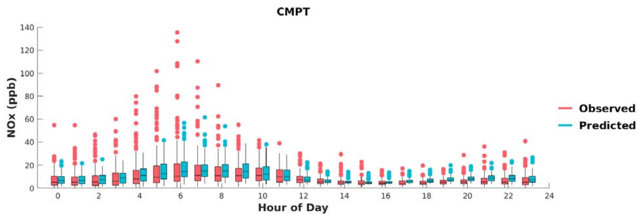
FIGURE I-5: BOX PLOTS OF OBSERVED VS. PREDICTED HOURLY NOx DURING MAY 1 ST TO SEPTEMBER 30 TH , 2018, AT COMPTON. HORIZONTAL LINES INDICATE 25 TH , 50 TH (MEDIAN), AND 75 TH PERCENTILES.
