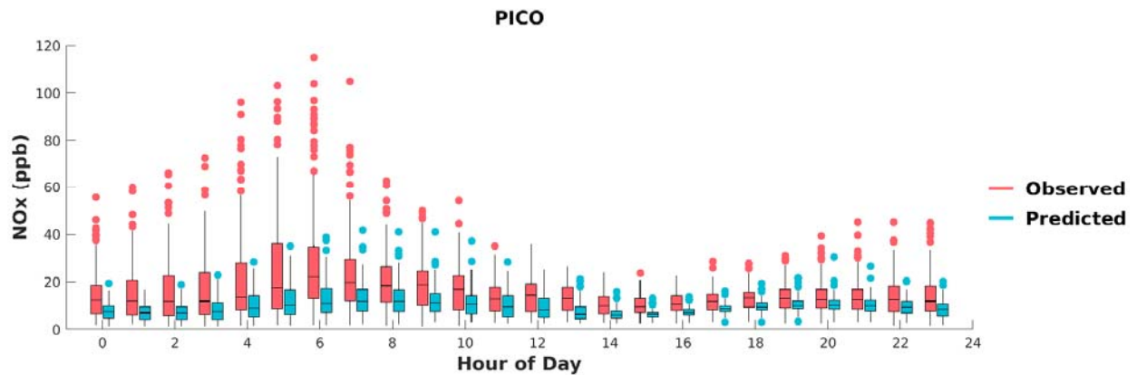
FIGURE I-14: BOX PLOTS OF OBSERVED VS. PREDICTED HOURLY NOX DURING MAY 1 ST TO SEPTEMBER 30 TH , 2018, AT PICO RIVERO. HORIZONTAL LINES INDICATE 25 TH , 50 TH (MEDIAN), AND 75 TH PERCENTILES.
