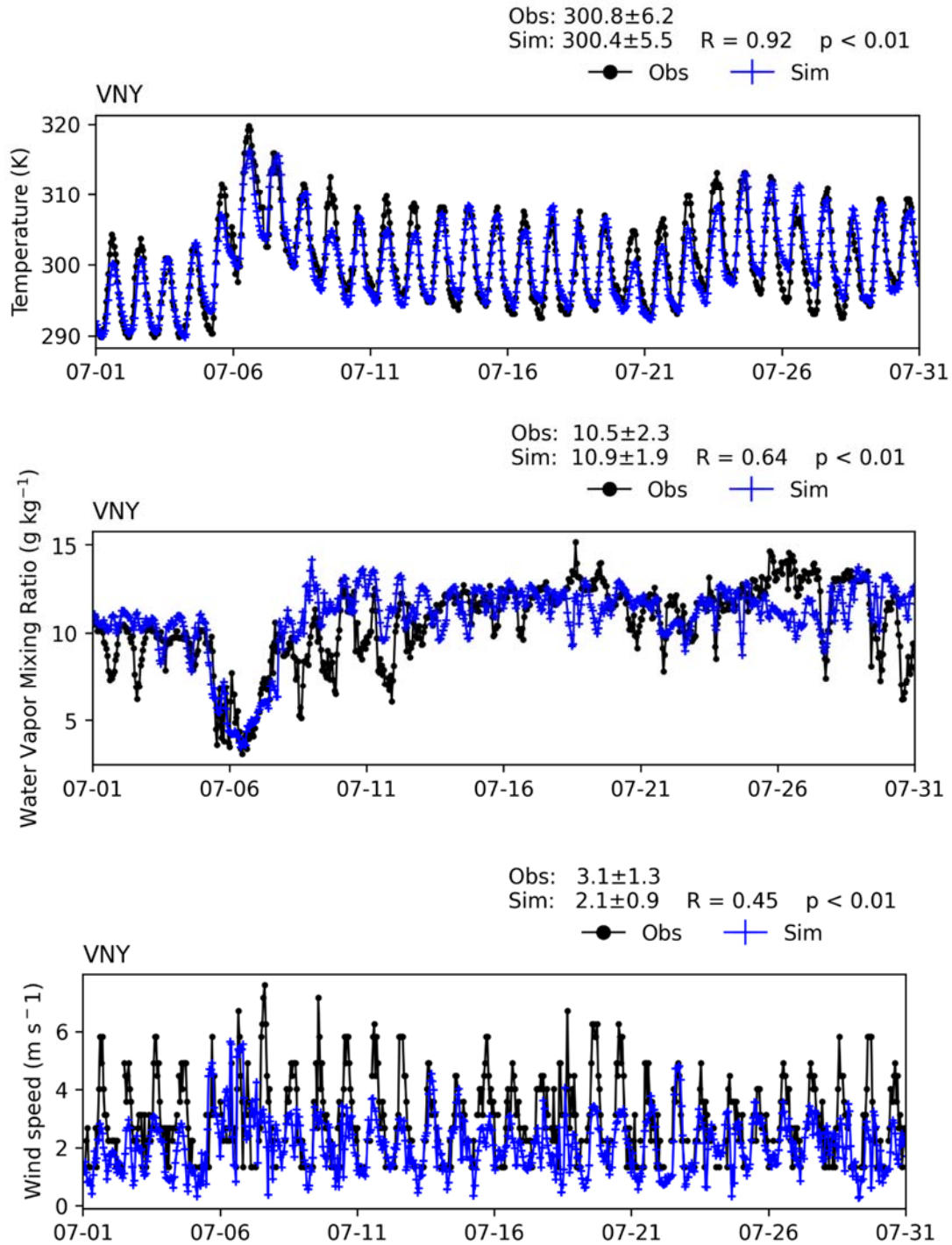
FIGURE V-A24 TIME SERIES OF HOURLY MEASUREMENTS AND WRF BASE SIMULATIONS AT VAN NUYS AIRPORT (VNY) FOR JULY 2018
