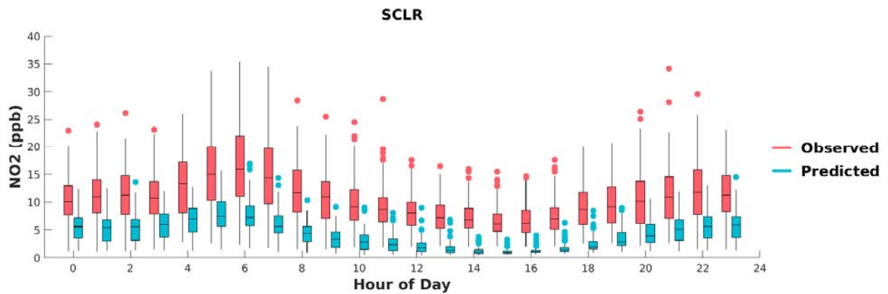
FIGURE H-19: BOX PLOTS OF OBSERVED VS. PREDICTED HOURLY NO2 DURING MAY 1 ST TO SEPTEMBER 30 TH , 2018, AT SANTA CLARITA. HORIZONTAL LINES INDICATE 25 TH , 50 TH (MEDIAN), AND 75 TH PERCENTILES.
