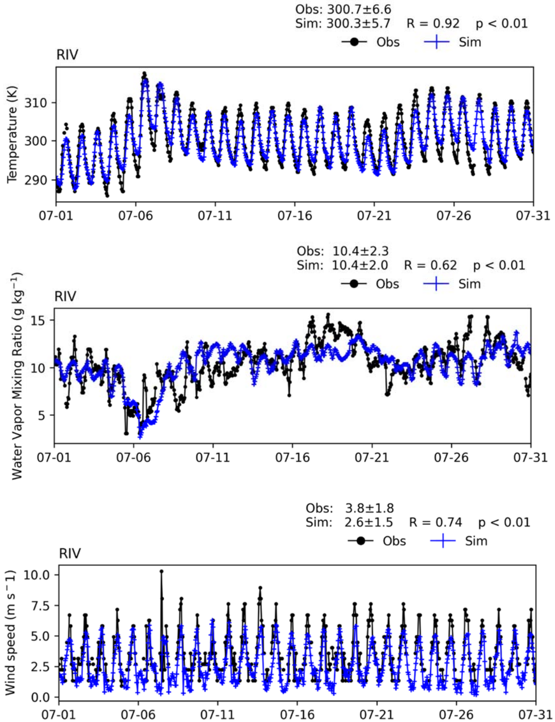
FIGURE V-A14 TIME SERIES OF HOURLY MEASUREMENTS AND WRF BASE SIMULATIONS AT MARCH AIR RESERVE AIRPORT (RIV) FOR JULY 2018
