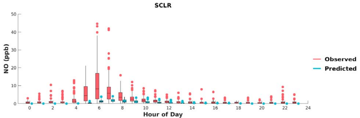
FIGURE G-19: BOX PLOTS OF OBSERVED VS. PREDICTED HOURLY NO DURING MAY 1 ST TO SEPTEMBER 30 TH , 2018, AT SANTA CLARITA. HORIZONTAL LINES INDICATE 25 TH , 50 TH (MEDIAN), AND 75 TH PERCENTILES.
