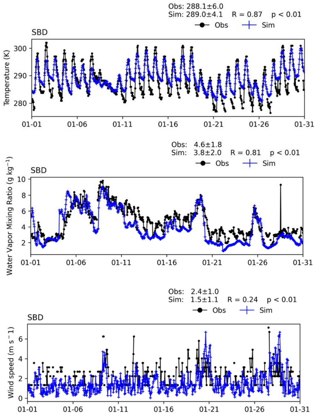
FIGURE V-A15 TIME SERIES OF HOURLY MEASUREMENTS AND WRF BASE SIMULATIONS AT SAN BERNARDINO INTERNATIONAL AIRPORT (SBD) FOR JANUARY 2018
