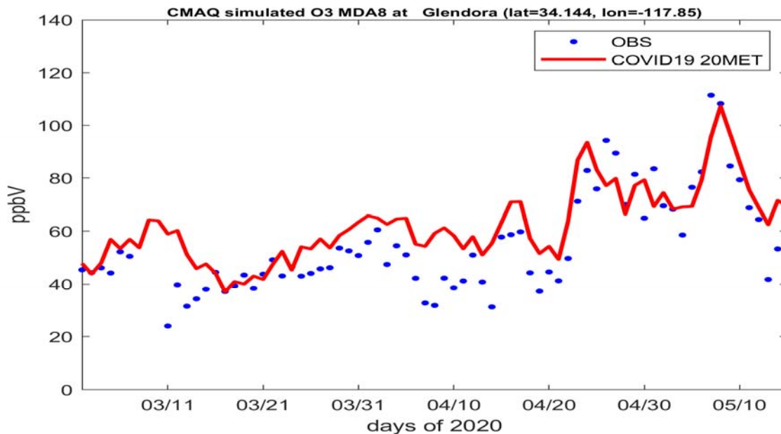
FIGURE V-5-33 MODELED AND OBSERVED 8-HOUR OZONE IN GLENDORA
