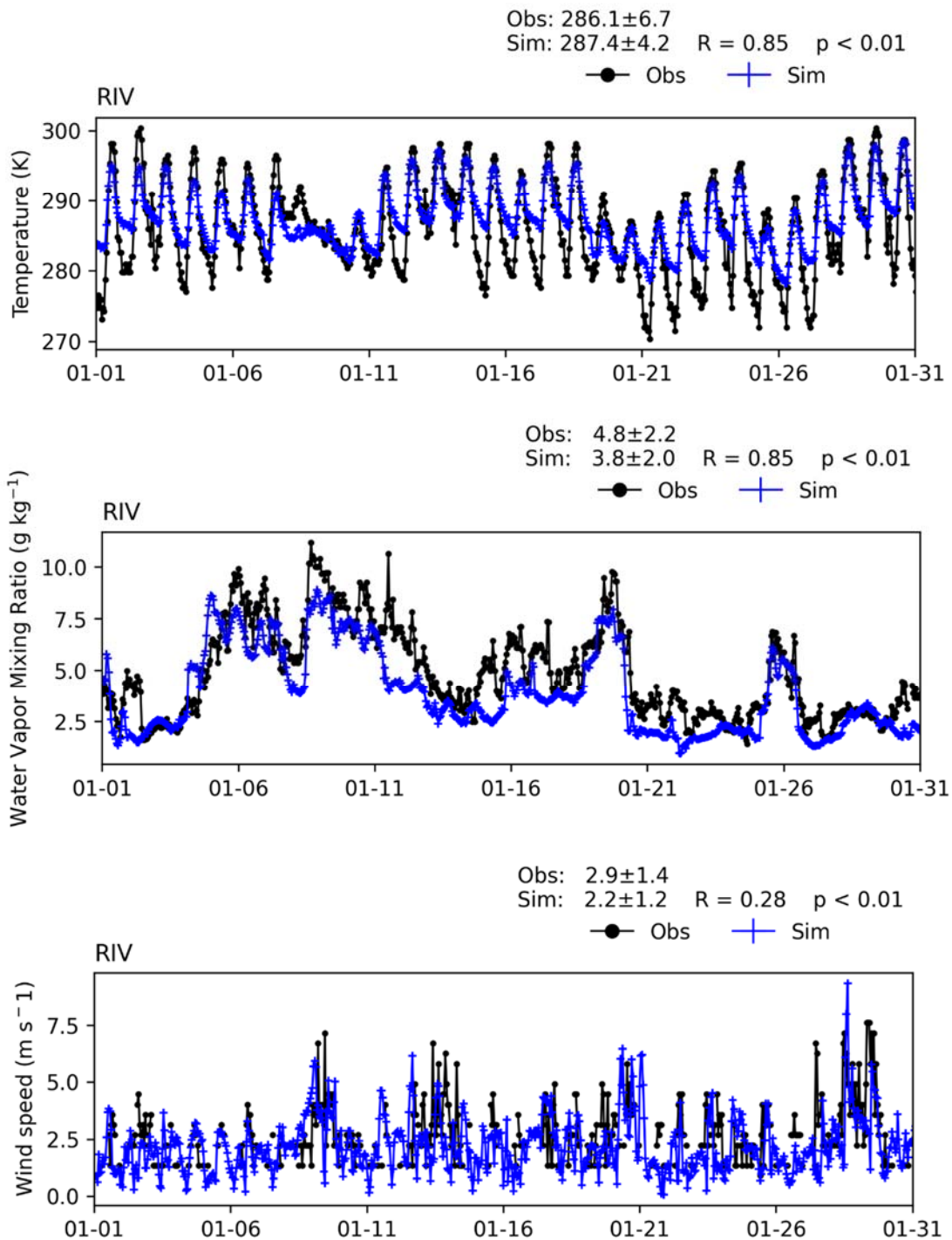
FIGURE V-A13 TIME SERIES OF HOURLY MEASUREMENTS AND WRF BASE SIMULATIONS AT MARCH AIR RESERVE AIRPORT (RIV) FOR JANUARY 2018
