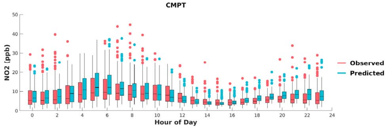
FIGURE H-5: BOX PLOTS OF OBSERVED VS. PREDICTED HOURLY NO 2 DURING MAY 1 ST TO SEPTEMBER 30 TH , 2018, AT COMPTON. HORIZONTAL LINES INDICATE 25 TH , 50 TH (MEDIAN), AND 75 TH PERCENTILES.
