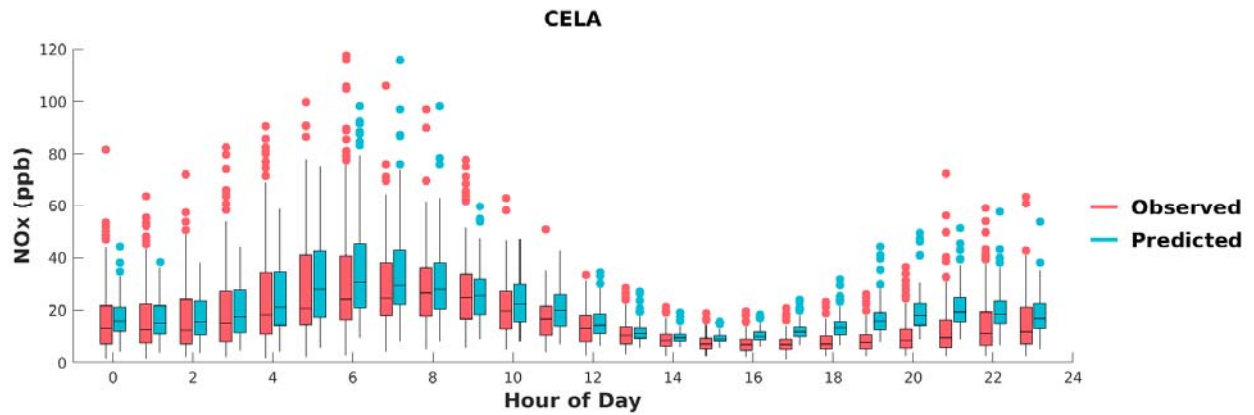
FIGURE I-4: BOX PLOTS OF OBSERVED VS. PREDICTED HOURLY NOx DURING MAY 1 ST TO SEPTEMBER 30 TH , 2018, AT CENTRAL LOS ANGELES. HORIZONTAL LINES INDICATE 25 TH , 50 TH (MEDIAN), AND 75 TH PERCENTILES.
