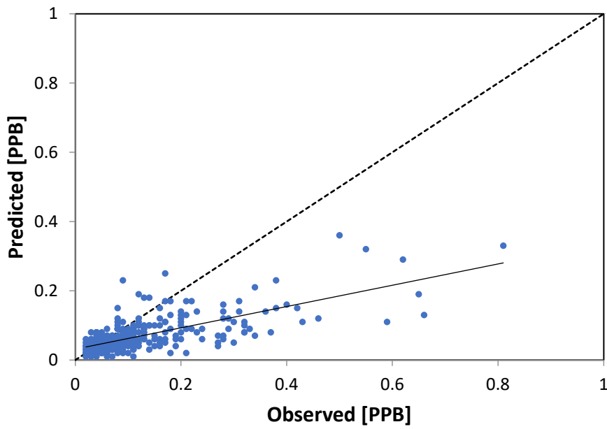
Figure 11. Scatter Plot of Predicted vs. Observed Concentrations o-Xylene
