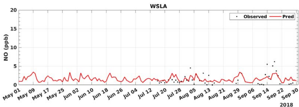
FIGURE B-27: 2018 DAILY AVERAGED NO MODEL PREDICTION AND MEASUREMENT COMPARISON AT WEST LOS ANGELES
