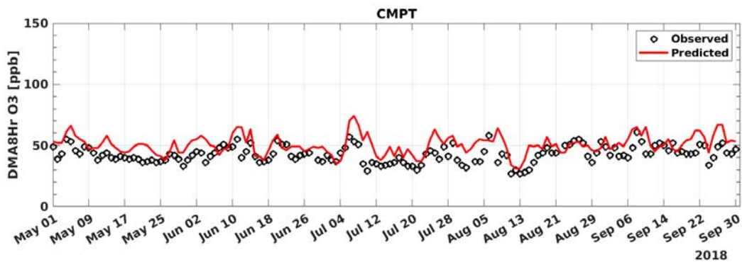
FIGURE A-5: 2018 MAXIMUM DAILY AVERAGE 8-HOUR (MDA8) OZONE MODEL PREDICTION AND MEASUREMENT COMPARISON AT COMPTON
