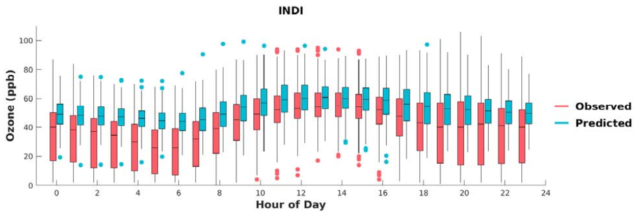
FIGURE F-12: BOX PLOTS OF OBSERVED VS. PREDICTED HOURLY OZONE DURING MAY 1 ST TO SEPTEMBER 30 TH , 2018, AT INDIO. HORIZONTAL LINES INDICATE 25 TH , 50 TH (MEDIAN), AND 75 TH PERCENTILES.
