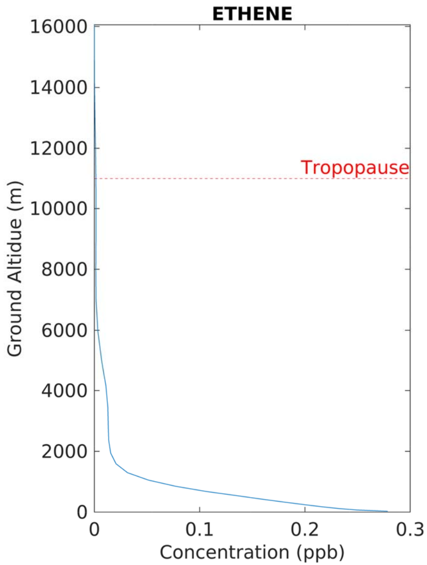
Figure 5: Vertical profile of ethene averaged over the Basin during July 2018
