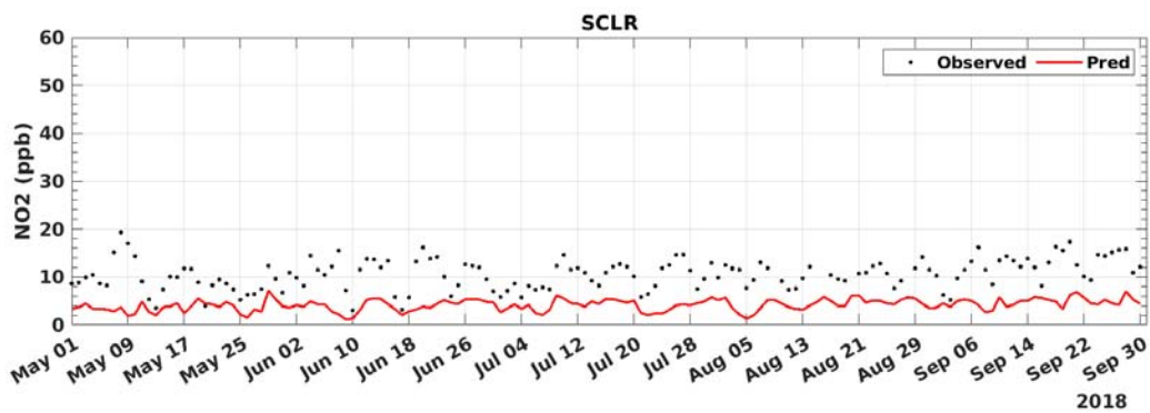
FIGURE C-20: 2018 DAILY AVERAGED NO2 MODEL PREDICTION AND MEASUREMENT COMPARISON AT SANTA CLARITA
