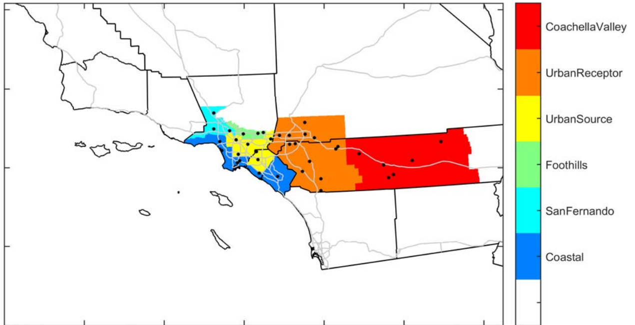
FIGURE V-5-1 PERFORMANCE EVALUATION ZONES
