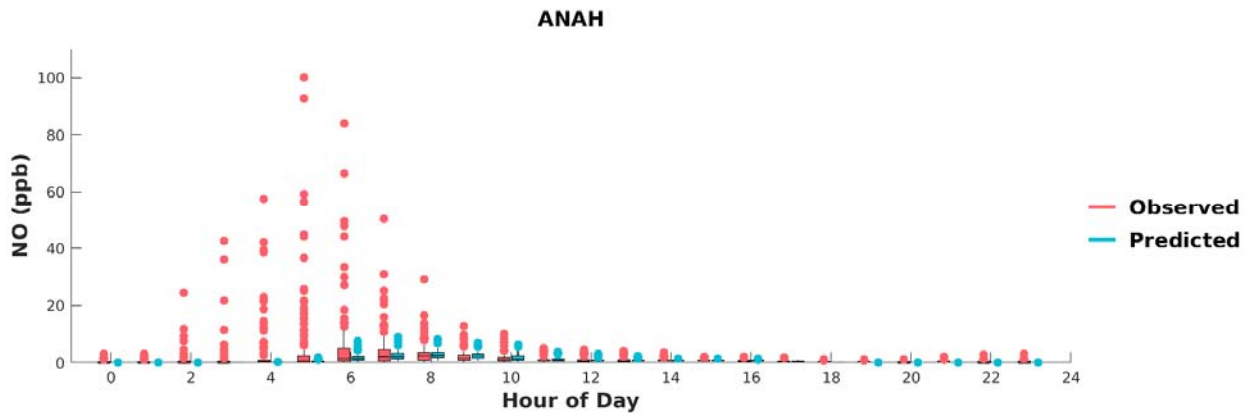
FIGURE G-1: BOX PLOTS OF OBSERVED VS. PREDICTED HOURLY NO DURING MAY 1 ST TO SEPTEMBER 30 TH , 2018, AT ANAHEIM. HORIZONTAL LINES INDICATE 25 TH , 50 TH (MEDIAN), AND 75 TH PERCENTILES.
