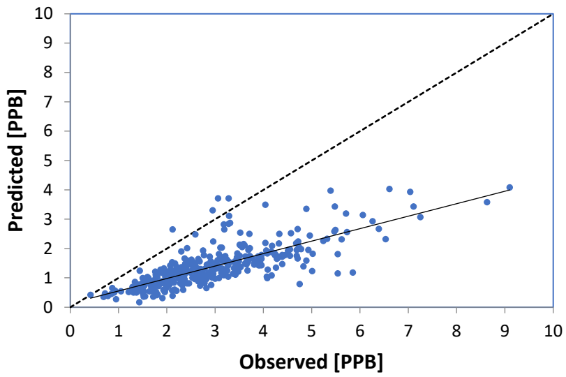
Figure 2. Scatter Plot of Predicted vs. Observed Concentrations Formaldehyde
