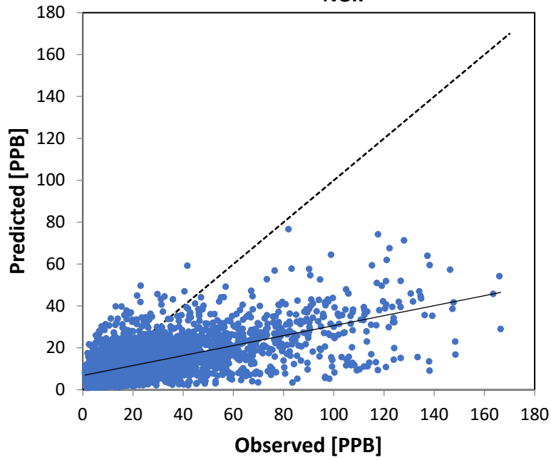
Figure 34. Scatter Plot of Predicted vs. Observed Concentrations NOx
