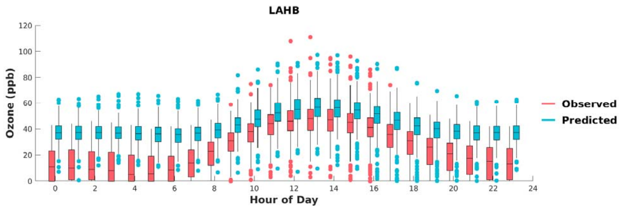
FIGURE F-13: BOX PLOTS OF OBSERVED VS. PREDICTED HOURLY OZONE DURING MAY 1 ST TO SEPTEMBER 30 TH , 2018, AT LA HABRA. HORIZONTAL LINES INDICATE 25 TH , 50 TH (MEDIAN), AND 75 TH PERCENTILES.
