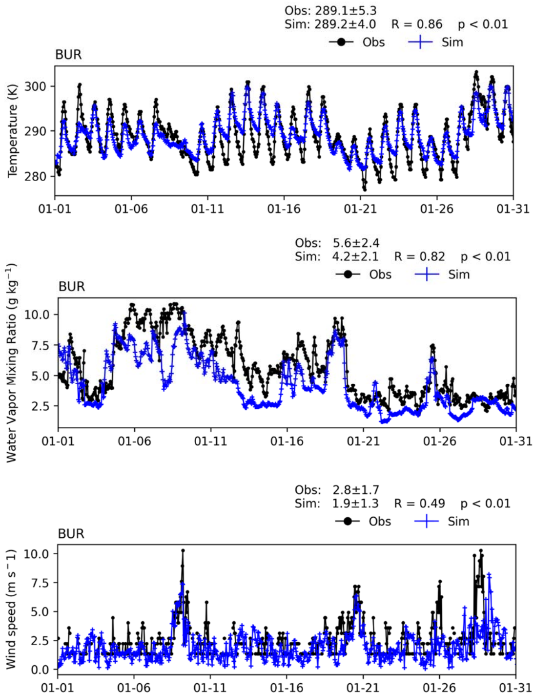
FIGURE V-A1 TIME SERIES OF HOURLY MEASUREMENTS AND WRF BASE SIMULATIONS AT BURBANK AIRPORT (BUR) FOR JANUARY 2018
