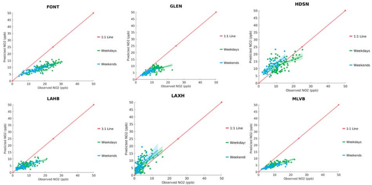
FIGURE M-2: SCATTER PLOT OF OBSERVED VS. PREDICTED DAILY AVERAGE NO 2 DURING MAY 1 ST TO SEPTEMBER 30 TH , 2018, AT FONTANA (FONT), SANTA GLENDORA (GLEN), HUDSON (HDSN), LA HABRA (LAHB), LAX (LAX) AND MIRA LOMA (MLVB). GREEN AND BLUE LINES INDICATE GENERAL LINEAR MODEL FIT WITH 95% CONFIDENCE INTERVAL (SHADED AREA). THE RED LINE INDICATES 1:1 LINE.
