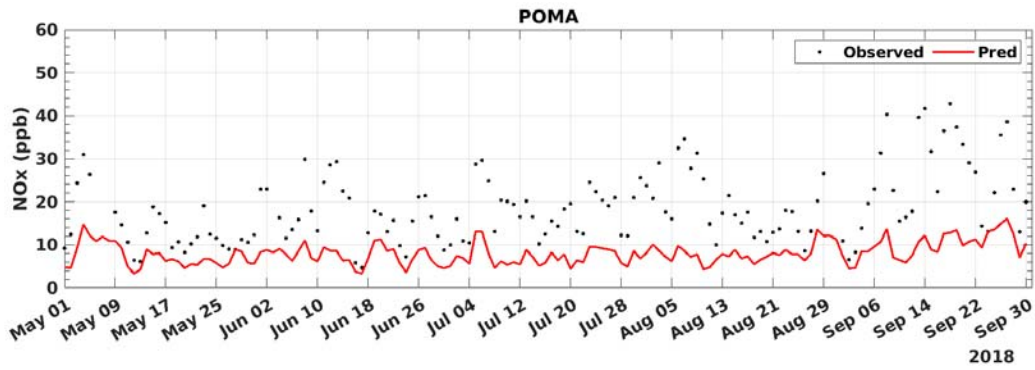
FIGURE D-16: 2018 DAILY AVERAGED NOX MODEL PREDICTION AND MEASUREMENT COMPARISON AT POMONA
