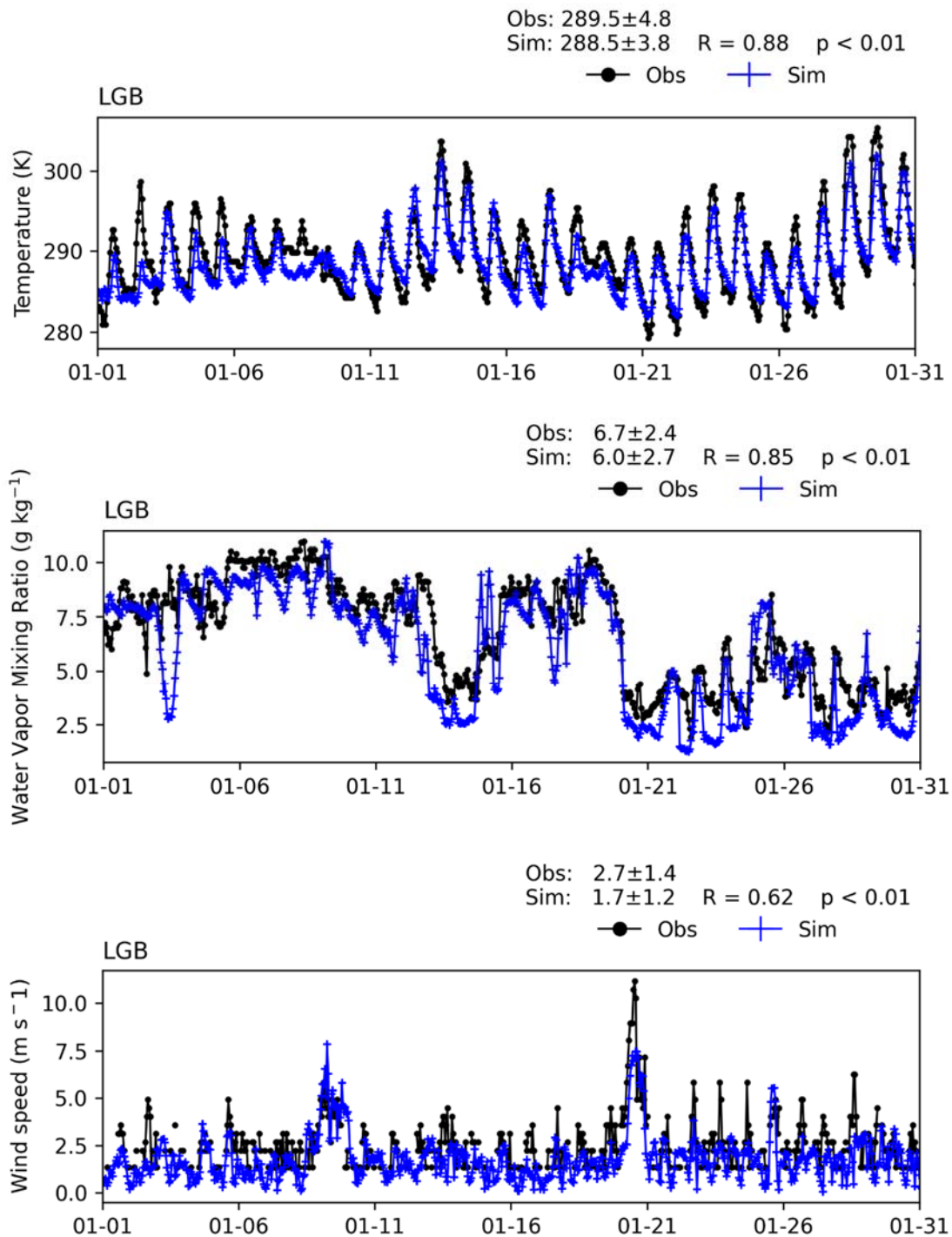
FIGURE V-A7 TIME SERIES OF HOURLY MEASUREMENTS AND WRF BASE SIMULATIONS AT LONG BEACH AIRPORT (LGB) FOR JANUARY 2018
