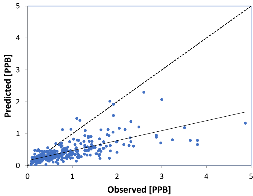
Figure 4. Scatter Plot of Predicted vs. Observed Concentrations Toluene
