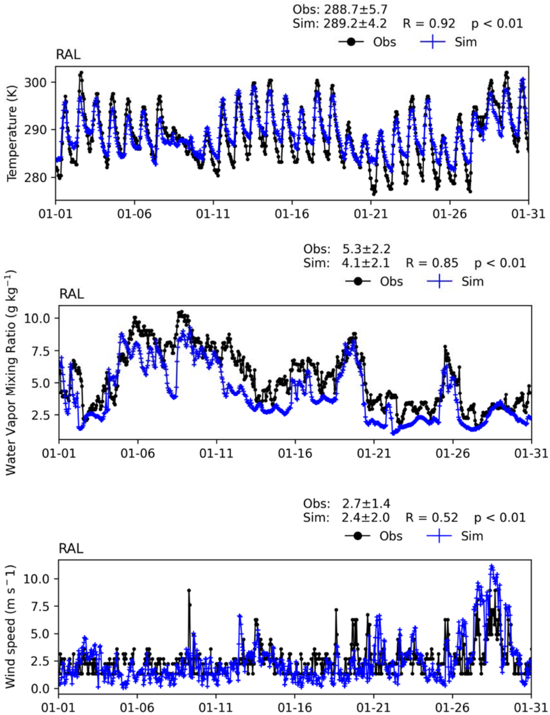
FIGURE V-A11 TIME SERIES OF HOURLY MEASUREMENTS AND WRF BASE SIMULATIONS AT RIVERSIDE MUNICIPAL AIRPORT (RAL) FOR JANUARY 2018
