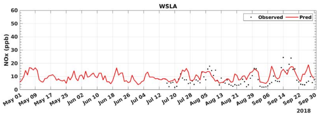
FIGURE D-23: 2018 DAILY AVERAGED NOX MODEL PREDICTION AND MEASUREMENT COMPARISON AT WEST LOS ANGELES
