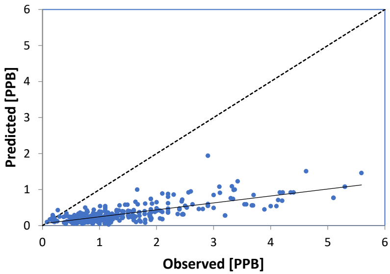
Figure 3. Scatter Plot of Predicted vs. Observed Concentrations Acetylene
