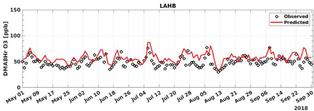
FIGURE A-11: 2018 MAXIMUM DAILY AVERAGE 8-HOUR (MDA8) OZONE MODEL PREDICTION AND MEASUREMENT COMPARISON AT LA HABRA
