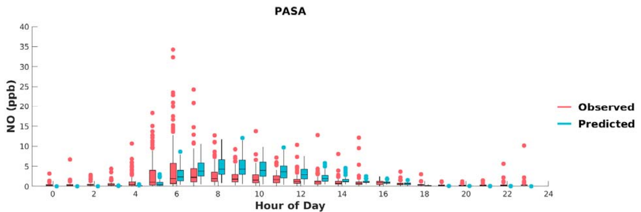
FIGURE G-13: BOX PLOTS OF OBSERVED VS. PREDICTED HOURLY NO DURING MAY 1 ST TO SEPTEMBER 30 TH , 2018, AT PASADENA. HORIZONTAL LINES INDICATE 25 TH , 50 TH (MEDIAN), AND 75 TH PERCENTILES.
