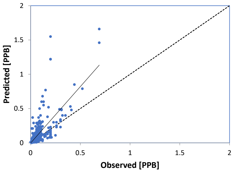
Figure 5. Scatter Plot of Predicted vs. Observed Concentrations Isoprene
