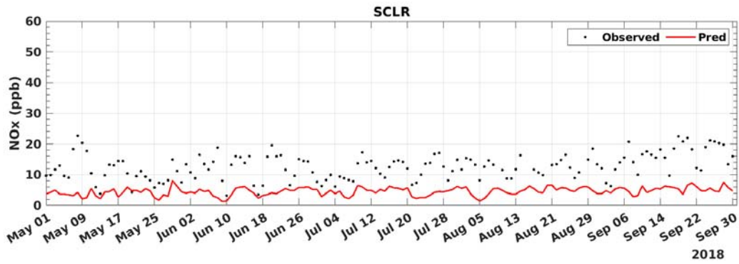
FIGURE D-19: 2018 DAILY AVERAGED NOX MODEL PREDICTION AND MEASUREMENT COMPARISON AT SANTA CLARITA
