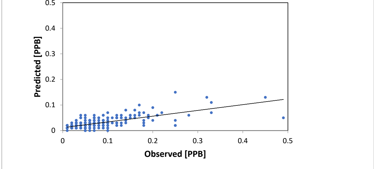
Figure 13. Scatter Plot of Predicted vs. Observed Concentrations 1,3-Butadiene
