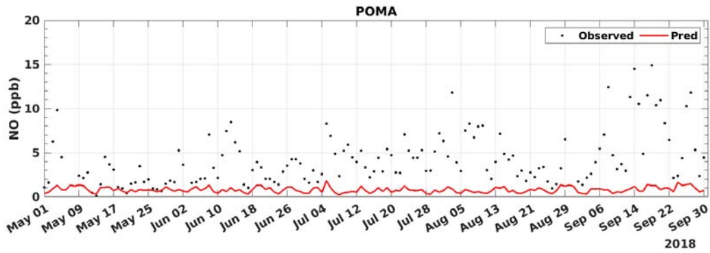
FIGURE B-19: 2018 DAILY AVERAGED NO MODEL PREDICTION AND MEASUREMENT COMPARISON AT POMONA
