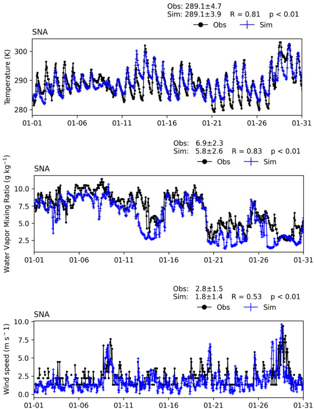
FIGURE V-A19 TIME SERIES OF HOURLY MEASUREMENTS AND WRF BASE SIMULATIONS AT SANTA ANA JOHN WAYNE AIRPORT (SNA) FOR JANUARY 2018
