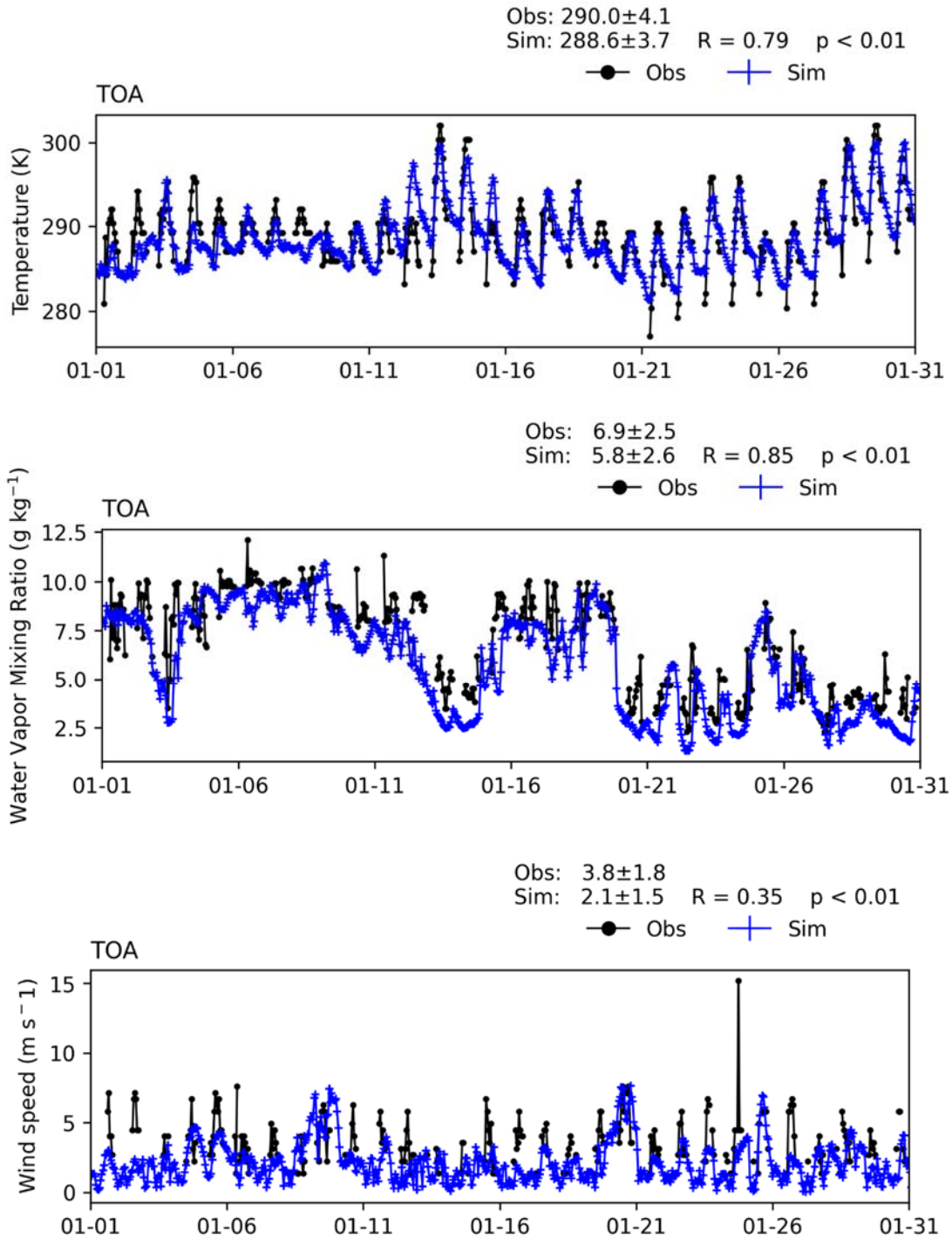
FIGURE V-A21 TIME SERIES OF HOURLY MEASUREMENTS AND WRF BASE SIMULATIONS AT TORRANCE (TOA) FOR JANUARY 2018
