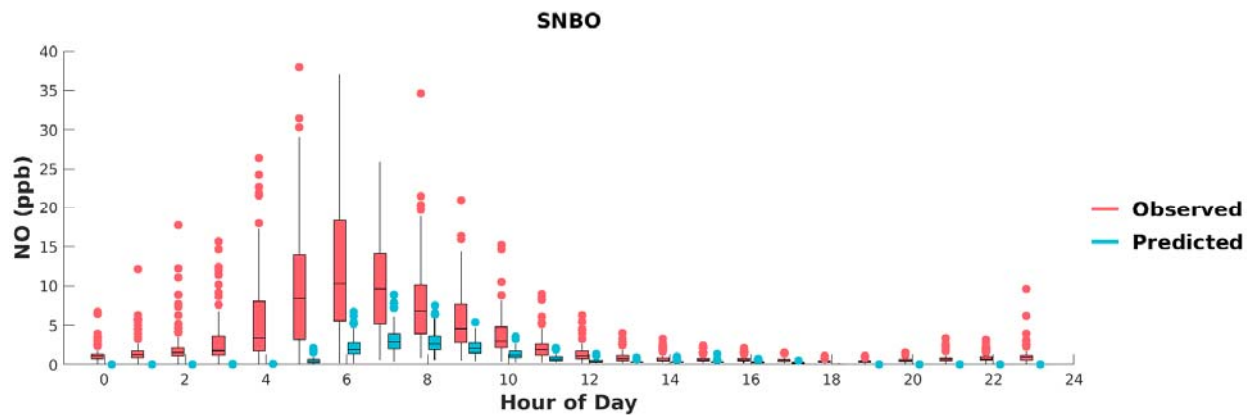
FIGURE G-21: BOX PLOTS OF OBSERVED VS. PREDICTED HOURLY NO DURING MAY 1 ST TO SEPTEMBER 30 TH , 2018, AT SAN BERNARDINO. HORIZONTAL LINES INDICATE 25 TH , 50 TH (MEDIAN), AND 75 TH PERCENTILES.
