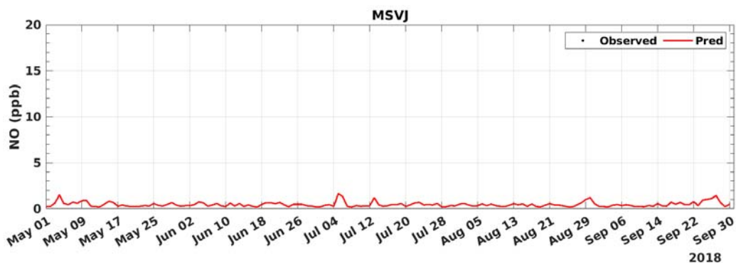
FIGURE B-15: 2018 DAILY AVERAGED NO MODEL PREDICTION AND MEASUREMENT COMPARISON AT MISSION VIEJO
