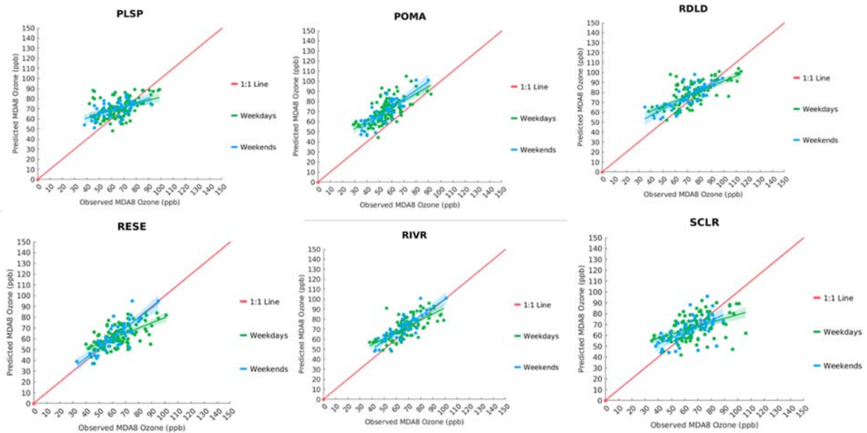
FIGURE K-4: SCATTER PLOT OF OBSERVED VS. PREDICTED MDA8 OZONE DURING MAY 1 ST TO SEPTEMBER 30 TH , 2018, AT PALM SPRINGS (PLSP), POMONA (POMA), RED LANDS (RDL), RESEDA (RESE), RIVERSIDE (RIVR), AND SANTA CLARITA (SCLR). GREEN AND BLUE LINES INDICATE GENERAL LINEAR MODEL FIT WITH 95% CONFIDENCE INTERVAL (SHADED AREA). THE RED LINE INDICATES 1:1 LINE.
