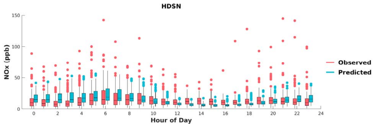
FIGURE I-9: BOX PLOTS OF OBSERVED VS. PREDICTED HOURLY NOX DURING MAY 1 ST TO SEPTEMBER 30 TH , 2018, AT HUDSON. HORIZONTAL LINES INDICATE 25 TH , 50 TH (MEDIAN), AND 75 TH PERCENTILES.
