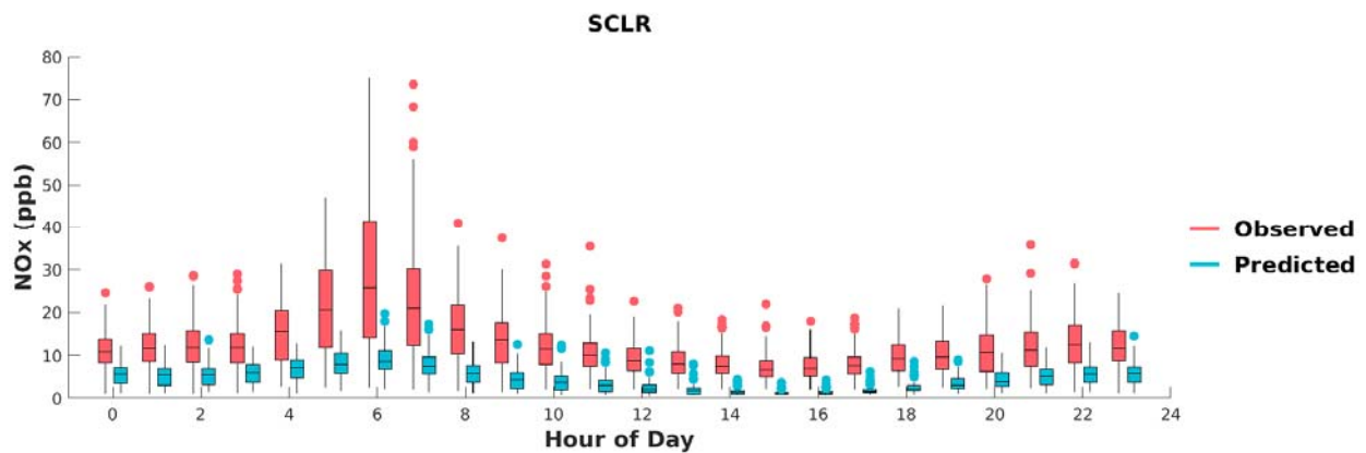
FIGURE I-19: BOX PLOTS OF OBSERVED VS. PREDICTED HOURLY NOX DURING MAY 1 ST TO SEPTEMBER 30 TH , 2018, AT SANTA CLARITA. HORIZONTAL LINES INDICATE 25 TH , 50 TH (MEDIAN), AND 75 TH PERCENTILES.
