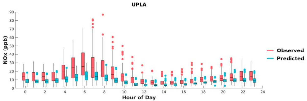
FIGURE I-22: BOX PLOTS OF OBSERVED VS. PREDICTED HOURLY NOx DURING MAY 1 ST TO SEPTEMBER 30 TH , 2018, AT UPLAND. HORIZONTAL LINES INDICATE 25 TH , 50 TH (MEDIAN), AND 75 TH PERCENTILES.
