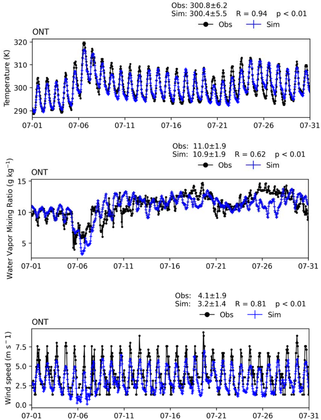
FIGURE V-A10 TIME SERIES OF HOURLY MEASUREMENTS AND WRF BASE SIMULATIONS AT ONTARIO INTERNATIONAL AIRPORT (ONT) FOR JULY 2018
