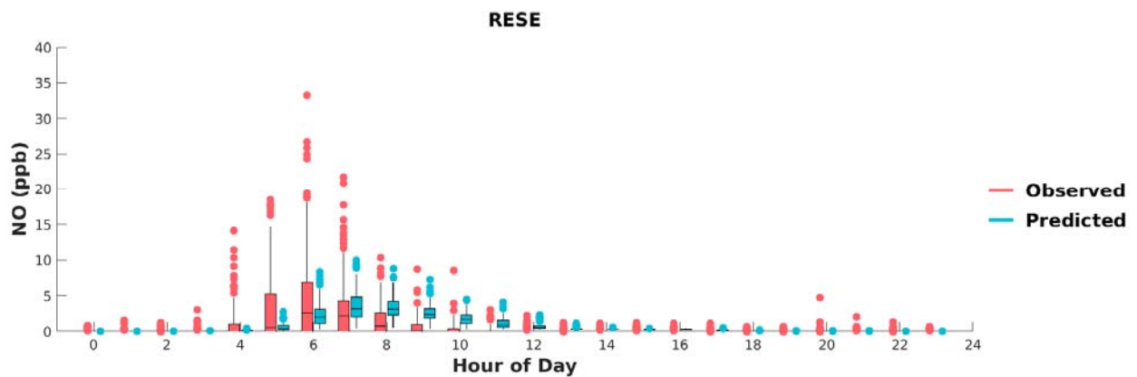
FIGURE G-17: BOX PLOTS OF OBSERVED VS. PREDICTED HOURLY NO DURING MAY 1 ST TO SEPTEMBER 30 TH , 2018, AT RESEDA. HORIZONTAL LINES INDICATE 25 TH , 50 TH (MEDIAN), AND 75 TH PERCENTILES.
