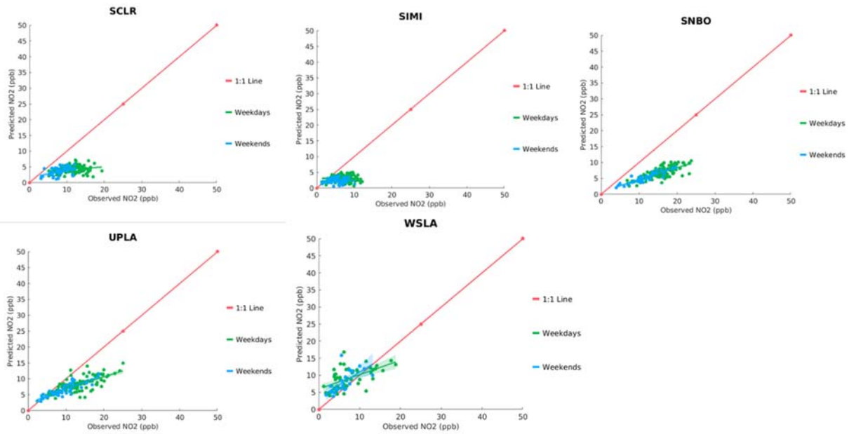
FIGURE M-4: SCATTER PLOT OF OBSERVED VS. PREDICTED DAILY AVERAGE NO 2 DURING MAY 1 ST TO SEPTEMBER 30 TH , 2018, AT SANTA CLARIRA (SCLR), SIMI VALLEY (SIMI), SAN BERNARDION (SNBO), UPLAND (UPLA), AND WEST LOS ANGELES (WSLA). GREEN AND BLUE LINES INDICATE GENERAL LINEAR MODEL FIT WITH 95% CONFIDENCE INTERVAL (SHADED AREA). THE RED LINE INDICATES 1:1 LINE.
