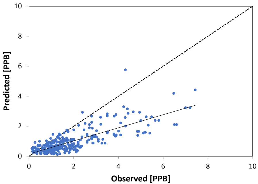
Figure 12. Scatter Plot of Predicted vs. Observed Concentrations Ethylene
