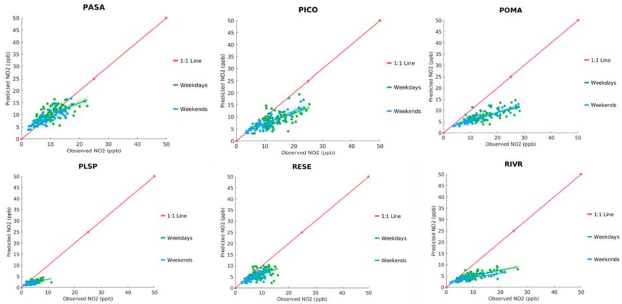
FIGURE M-3: SCATTER PLOT OF OBSERVED VS. PREDICTED DAILY AVERAGE NO 2 DURING MAY 1 ST TO SEPTEMBER 30 TH , 2018, AT PASADENA (PASA), PICO RIVERO (PICO), POMONA (POMA), PALM SPRINGS (PLSP), RESEDA (RESE), AND RIVERSIDE (RIVR). GREEN AND BLUE LINES INDICATE GENERAL LINEAR MODEL FIT WITH 95% CONFIDENCE INTERVAL (SHADED AREA). THE RED LINE INDICATES 1:1 LINE.
