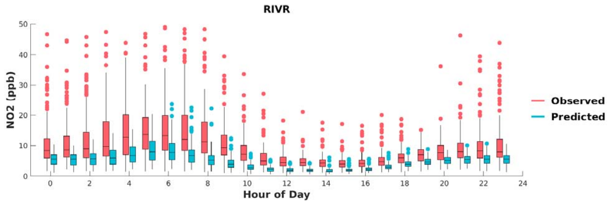
FIGURE H-18: BOX PLOTS OF OBSERVED VS. PREDICTED HOURLY NO2 DURING MAY 1 ST TO SEPTEMBER 30 TH , 2018, AT RIVERSIDE. HORIZONTAL LINES INDICATE 25 TH , 50 TH (MEDIAN), AND 75 TH PERCENTILES.
