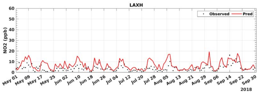
FIGURE C-11: 2018 DAILY AVERAGED NO2 MODEL PREDICTION AND MEASUREMENT COMPARISON AT LAX
