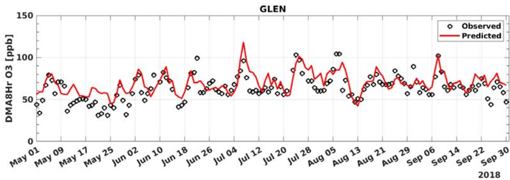
FIGURE A-9: 2018 MAXIMUM DAILY AVERAGE 8-HOUR (MDA8) OZONE MODEL PREDICTION AND MEASUREMENT COMPARISON AT GLENDORA
