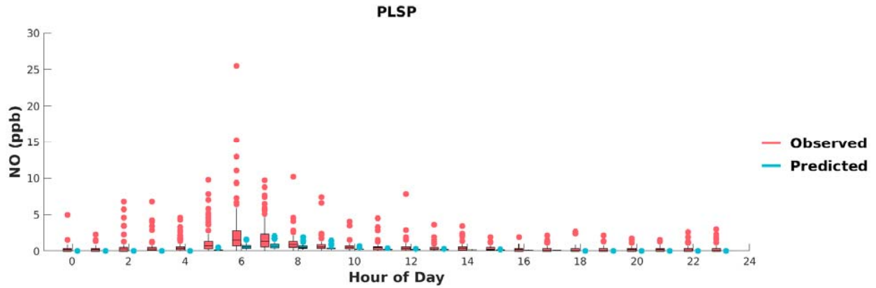
FIGURE G-16: BOX PLOTS OF OBSERVED VS. PREDICTED HOURLY NO DURING MAY 1 ST TO SEPTEMBER 30 TH , 2018, AT PALM SPRINGS. HORIZONTAL LINES INDICATE 25 TH , 50 TH (MEDIAN), AND 75 TH PERCENTILES.
