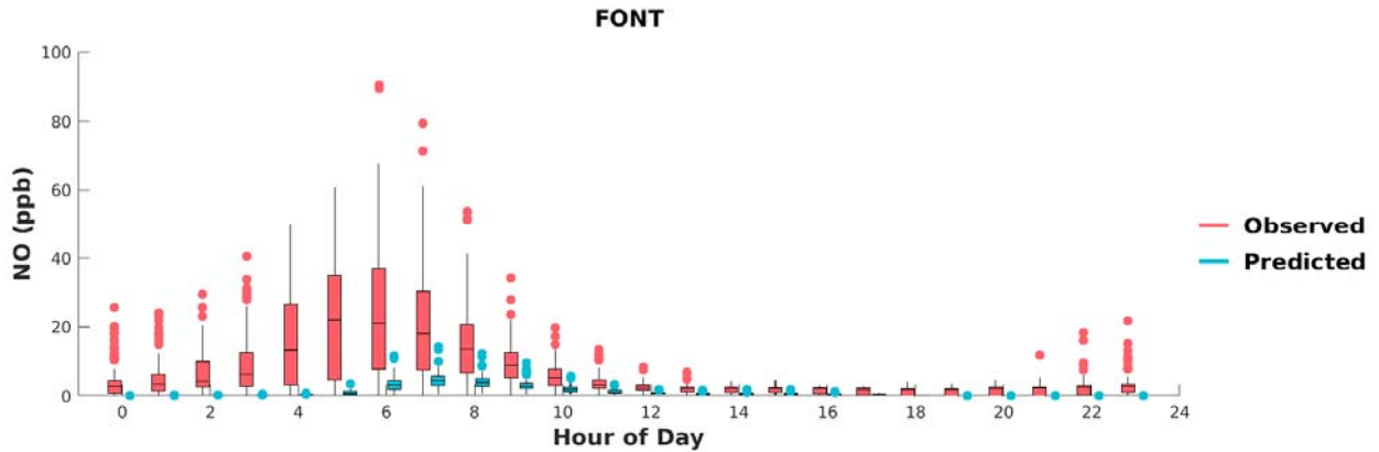
FIGURE G-7: BOX PLOTS OF OBSERVED VS. PREDICTED HOURLY NO DURING MAY 1 ST TO SEPTEMBER 30 TH , 2018, AT FONTANA. HORIZONTAL LINES INDICATE 25 TH , 50 TH (MEDIAN), AND 75 TH PERCENTILES.
