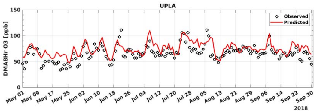
FIGURE A-26: 2018 MAXIMUM DAILY AVERAGE 8-HOUR (MDA8) OZONE MODEL PREDICTION AND MEASUREMENT COMPARISON AT UPLAND
