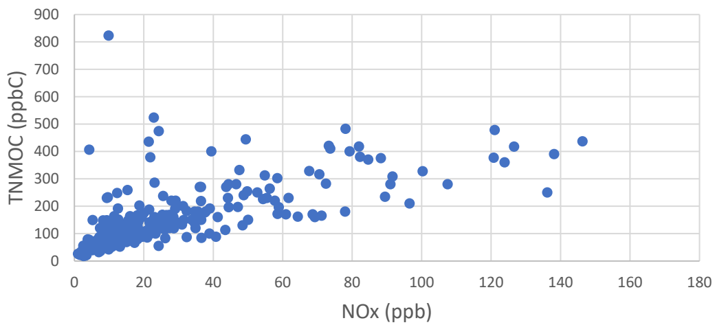
Figure 35. Observed TNMOC and NOx Concentrations
