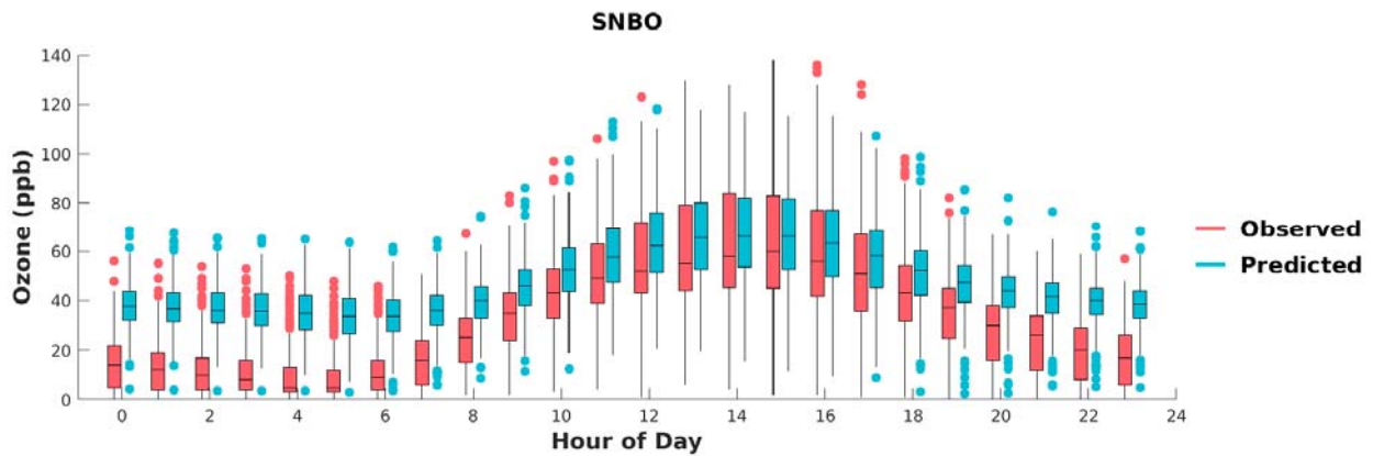
FIGURE F-28: BOX PLOTS OF OBSERVED VS. PREDICTED HOURLY OZONE DURING MAY 1 ST TO SEPTEMBER 30 TH , 2018, AT SAN BERNARDINO. HORIZONTAL LINES INDICATE 25 TH , 50 TH (MEDIAN), AND 75 TH PERCENTILES.
