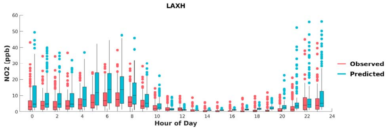
FIGURE H-11: BOX PLOTS OF OBSERVED VS. PREDICTED HOURLY NO2 DURING MAY 1 ST TO SEPTEMBER 30 TH , 2018, AT LAX. HORIZONTAL LINES INDICATE 25 TH , 50 TH (MEDIAN), AND 75 TH PERCENTILES.
