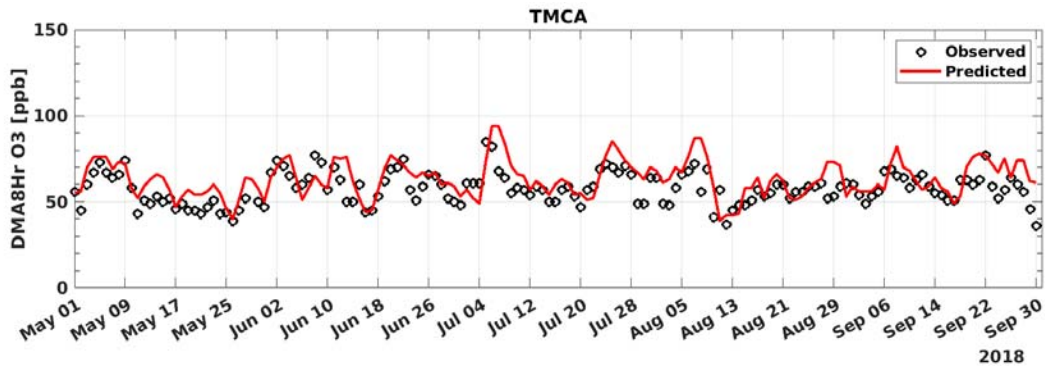
FIGURE A-25: 2018 MAXIMUM DAILY AVERAGE 8-HOUR (MDA8) OZONE MODEL PREDICTION AND MEASUREMENT COMPARISON AT TEMECULA
