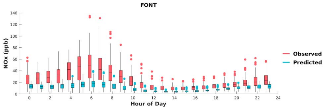
FIGURE I-7: BOX PLOTS OF OBSERVED VS. PREDICTED HOURLY NOX DURING MAY 1 ST TO SEPTEMBER 30 TH , 2018, AT FONTANA. HORIZONTAL LINES INDICATE 25 TH , 50 TH (MEDIAN), AND 75 TH PERCENTILES.
