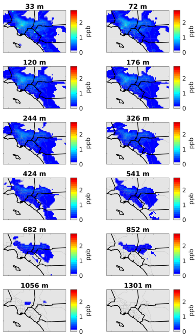
Figure 137: Vertical cross-sections of ethene during July 2018. Heights correspond to the top of each layer.
