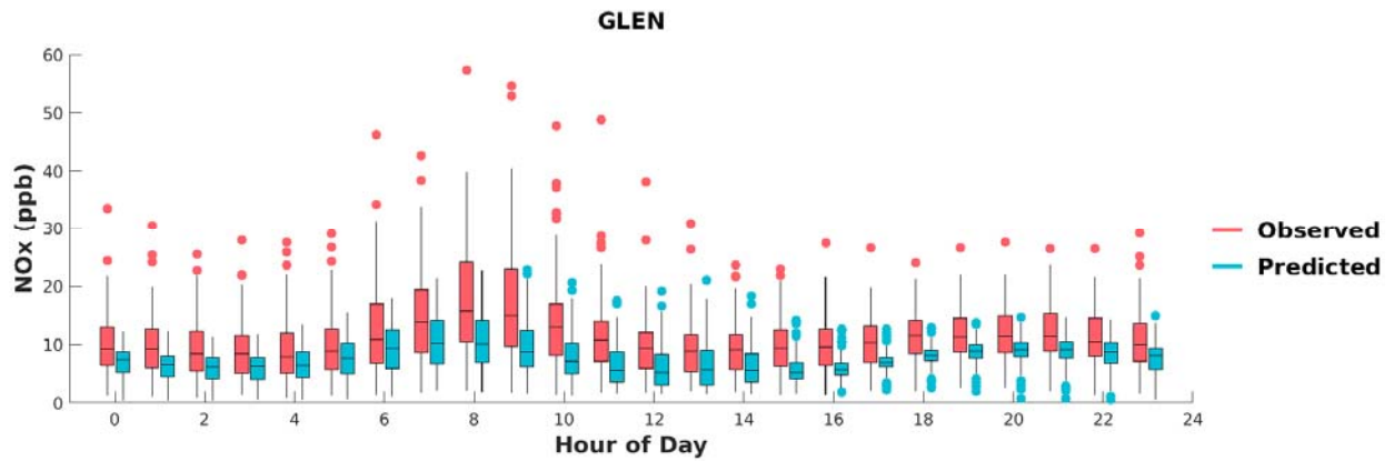
FIGURE I-8: BOX PLOTS OF OBSERVED VS. PREDICTED HOURLY NOX DURING MAY 1 ST TO SEPTEMBER 30 TH , 2018, AT GLENDORA. HORIZONTAL LINES INDICATE 25 TH , 50 TH (MEDIAN), AND 75 TH PERCENTILES.
