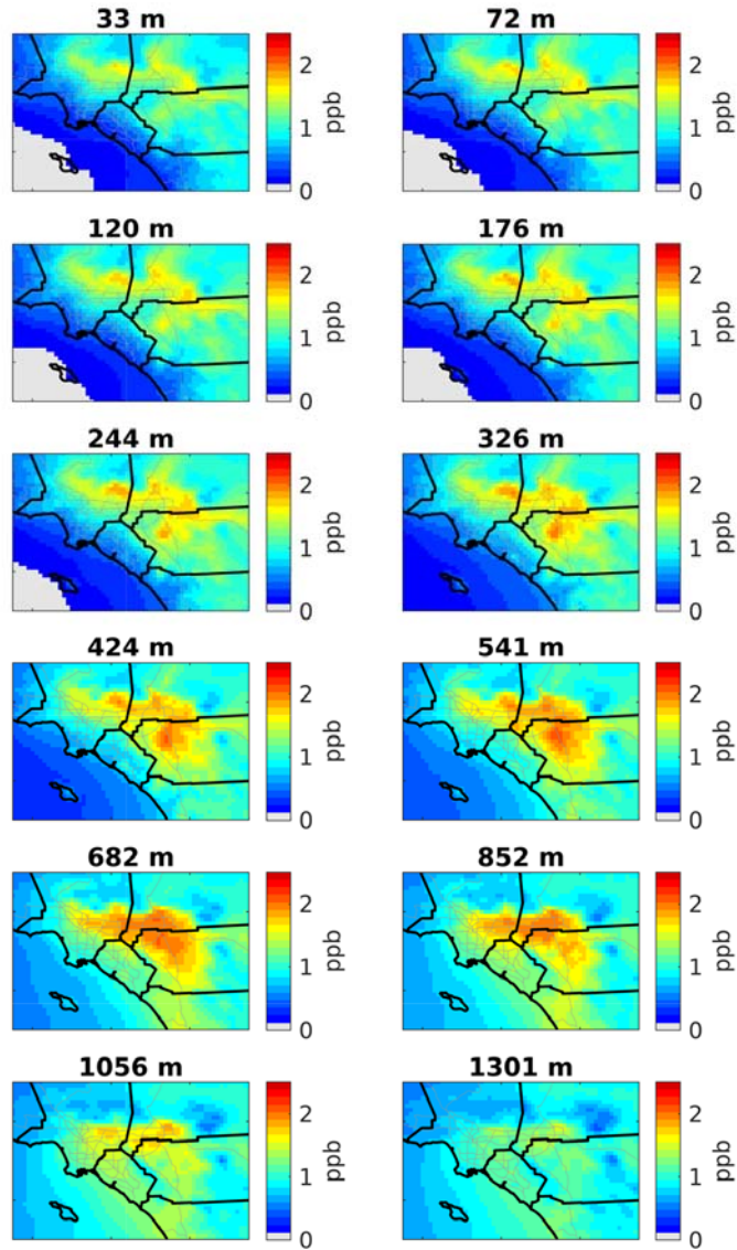
Figure 107: Vertical cross-sections of HNO 3 during July 2018. Heights correspond to the top of each layer.
