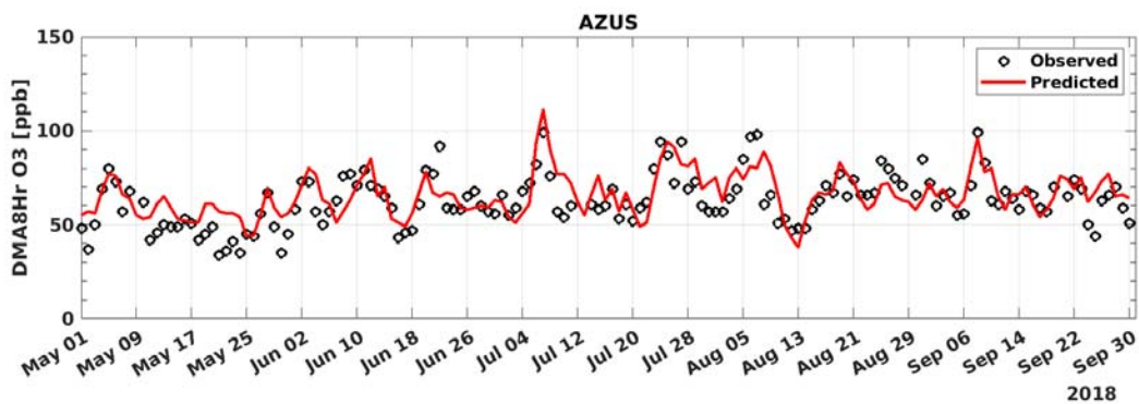
FIGURE A-2: 2018 MAXIMUM DAILY AVERAGE 8-HOUR (MDA8) OZONE MODEL PREDICTION AND MEASUREMENT COMPARISON AT AZUSA
