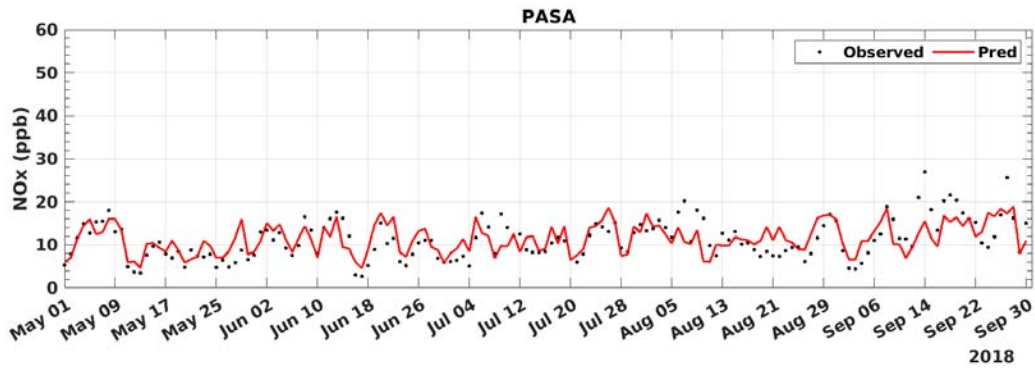
FIGURE D-13: 2018 DAILY AVERAGED NOX MODEL PREDICTION AND MEASUREMENT COMPARISON AT PASADENA
