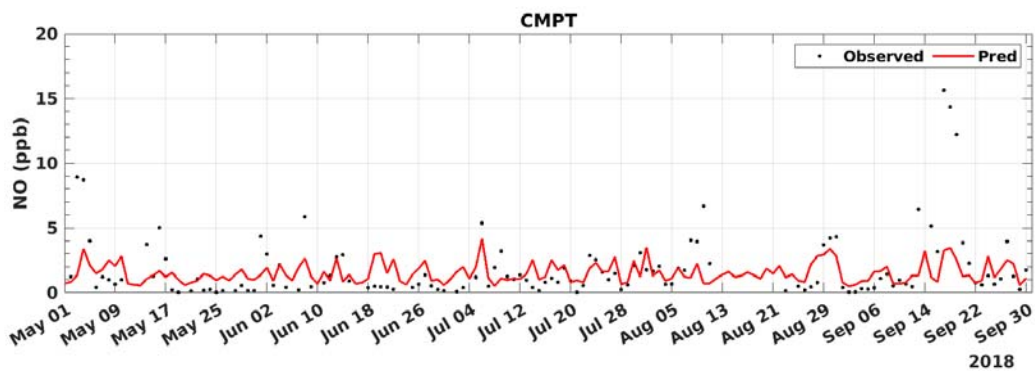
FIGURE B-5: 2018 DAILY AVERAGED NO MODEL PREDICTION AND MEASUREMENT COMPARISON AT COMPTON
