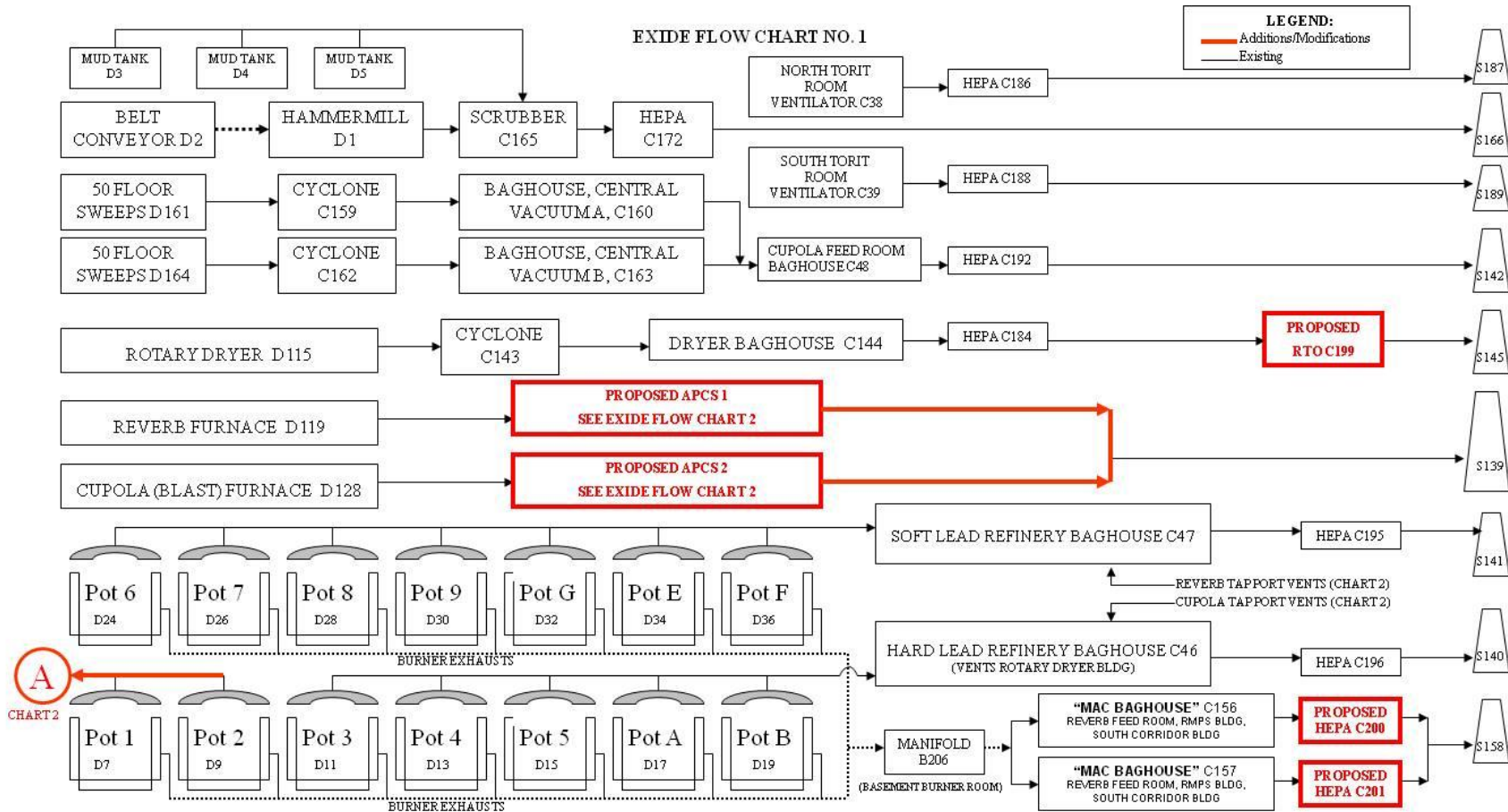
Figure 1-3 Flow Chart 1 of the Changes to the Exide Facility
