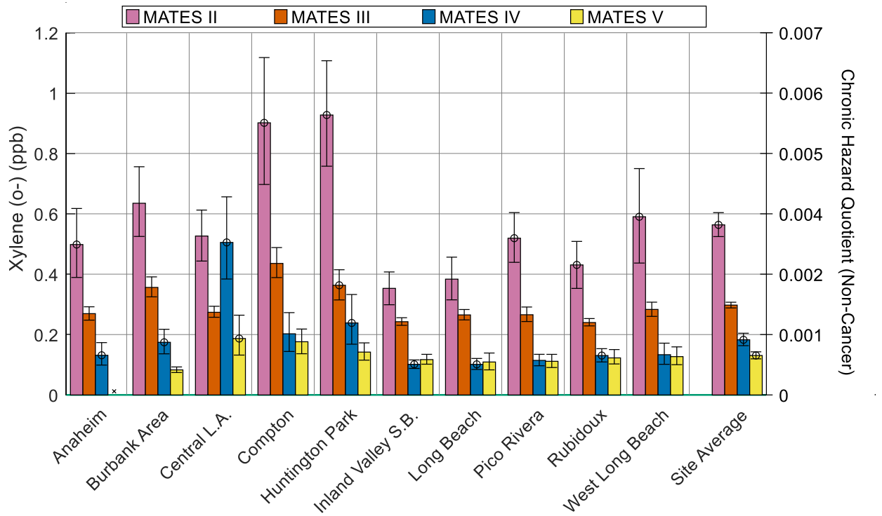
Figure 2-16 Average Concentrations of Xylene (o-). “x” in the place of a bar indicates that there are no data for a given station/MATES iteration. “o” at the top of a bar or in the location of a missing bar indicates that valid measurements do not exist for at least 75% of the sampling days in all quarters. Error bars denote the 95% confidence interval.
