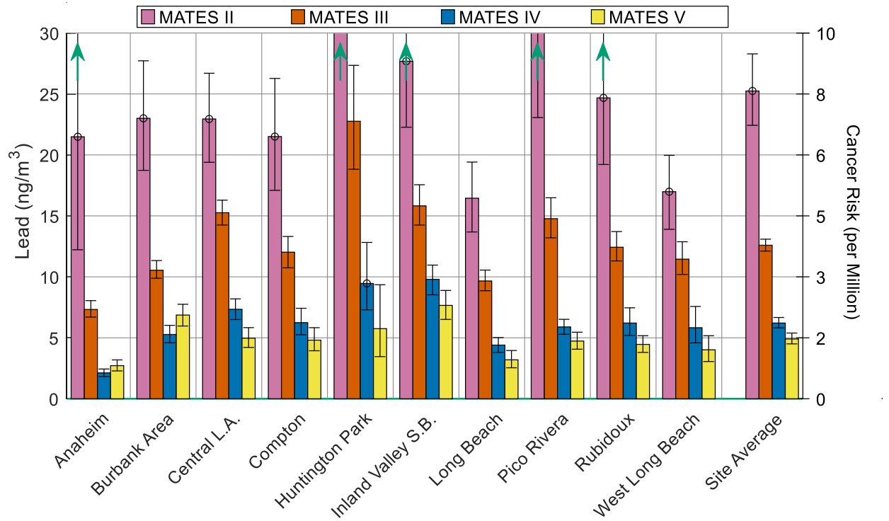
Figure 2-29 Average Concentrations of TSP Lead. The upward arrows indicate that the data extends above the y-axis shown. “o” indicates that valid measurements do not exist for at least 75% of the sampling days in each quarter. Error bars denote the 95% confidence interval.
