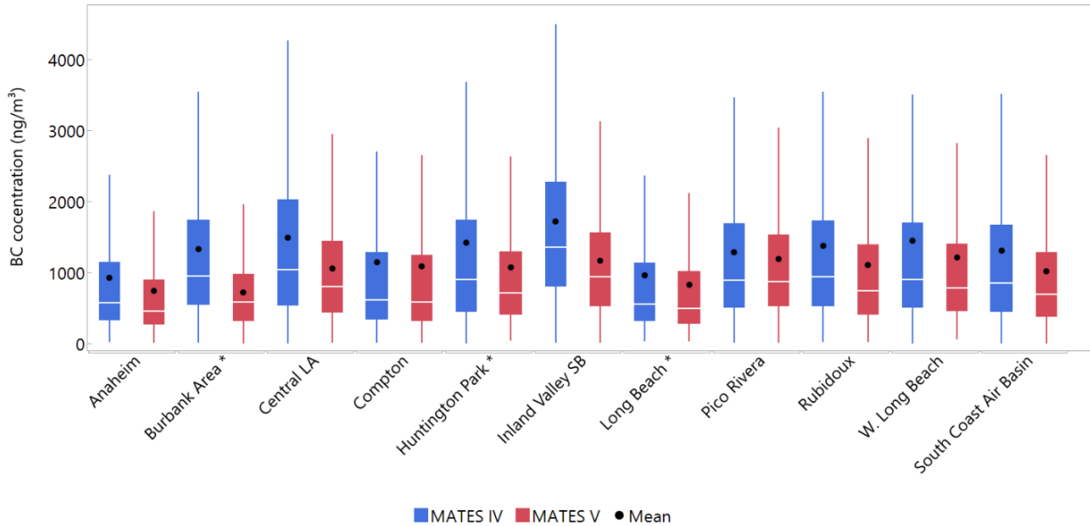
Figure 5-7. A comparison between the spatial distribution of BC levels during MATES IV and MATES V. *Refers to sites that have been relocated between the two study periods.
