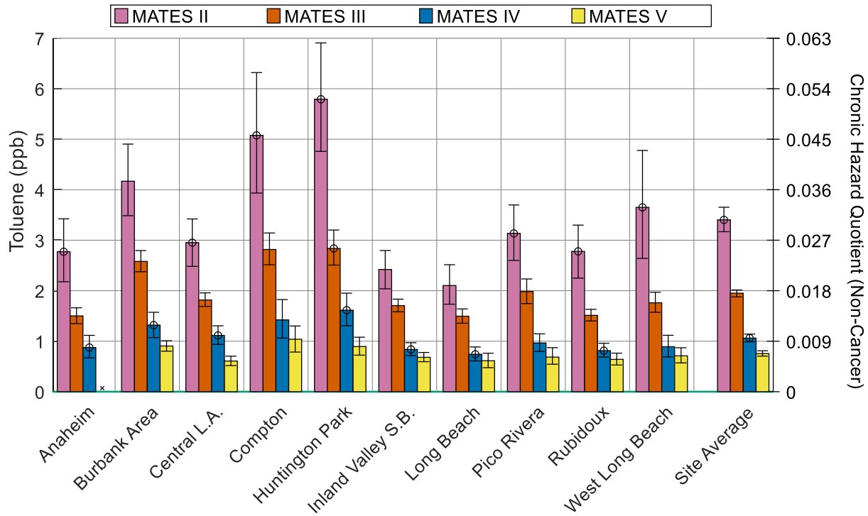
Figure 2-8 Average Concentrations of Toluene. “x” in the place of a bar indicates that there are no data for a given station/MATES iteration. “o” at the top of a bar or in the location of a missing bar indicates that valid measurements do not exist for at least 75% of the sampling days in all quarters. Error bars denote the 95% confidence interval.
