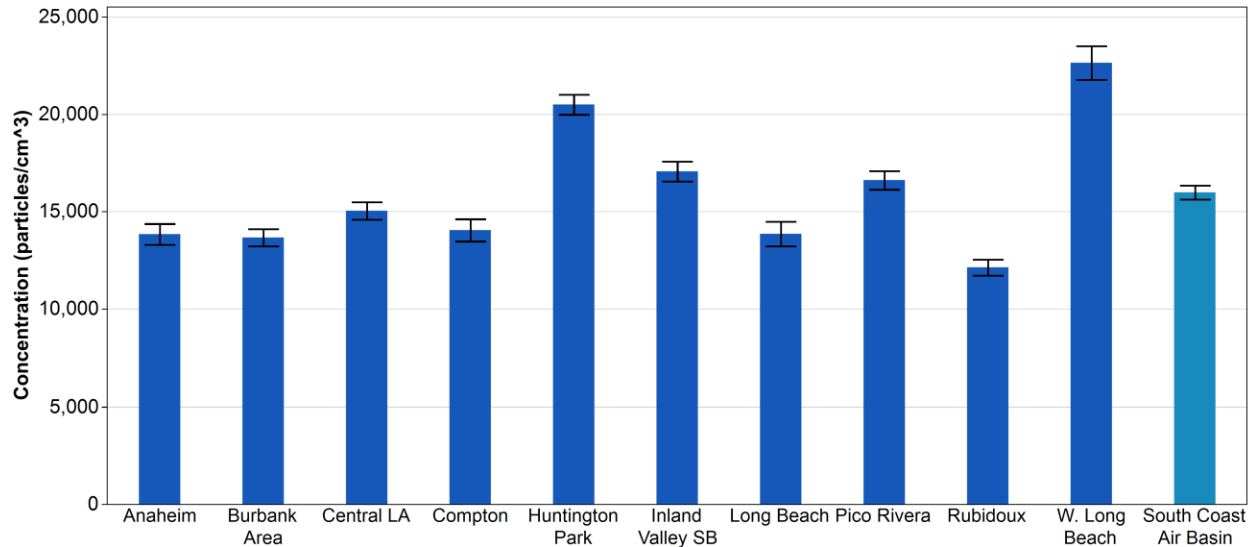
Figure 5-1. Ultrafine particle concentration mean and 95% confidence interval for each site and the South Coast Air Basin (10 site average)
