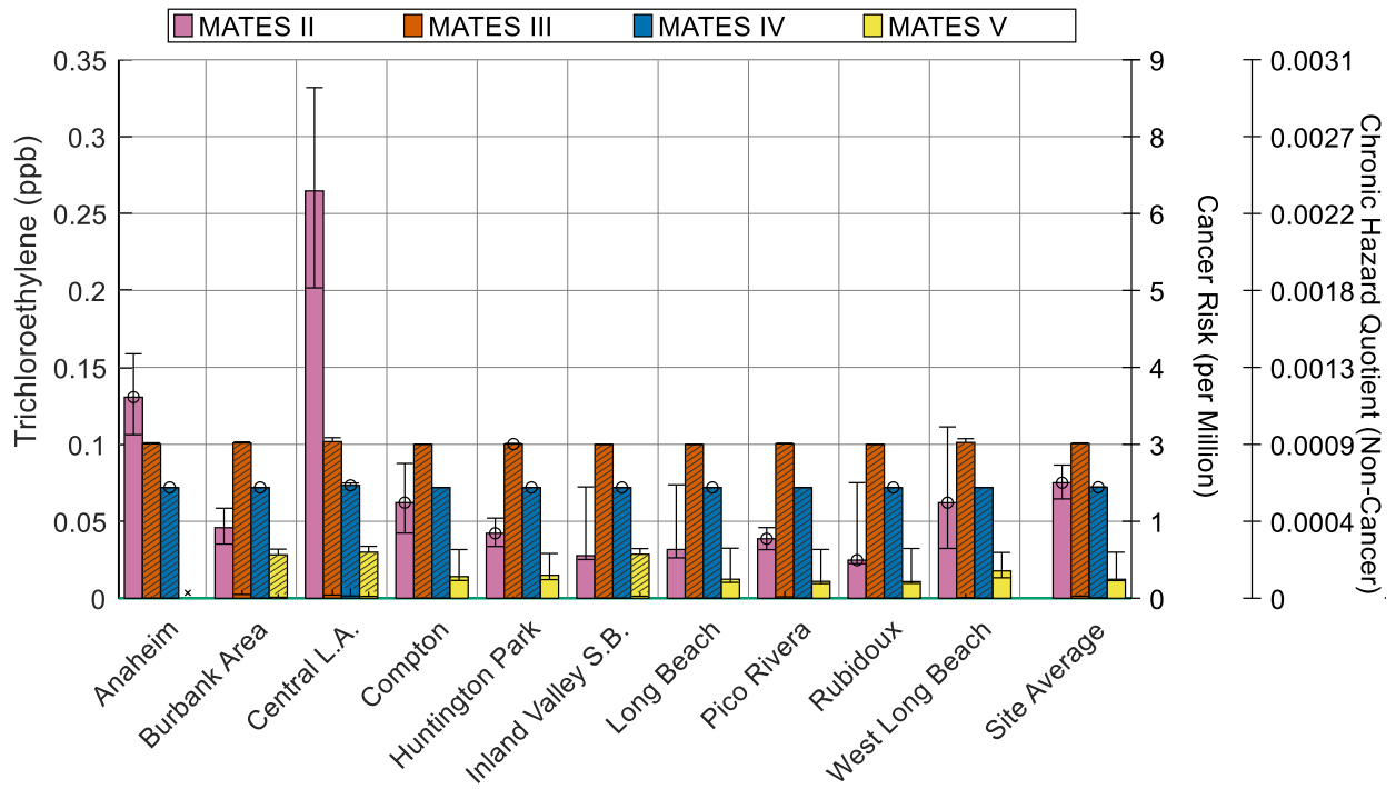
Figure 2-21 Average Concentrations of Trichloroethylene. The diagonal lines (shading) on the bars indicate that more than 80% of the measurements for those stations were below the method detection limits (MDLs). The lower edge of the shading shows the mean with zero substituted for all measurements below the MDL. The upper edge of the shading shows the mean with the MDL substituted for all measurements below the MDL. All other averages are calculated using the KM mean. “x” in the place of a bar indicates that there are no data for a given station/MATES iteration. “o” at the top of a bar or in the location of a missing bar indicates that valid measurements do not exist for at least 75% of the sampling days in all quarters. Error bars denote the 95% confidence interval.
