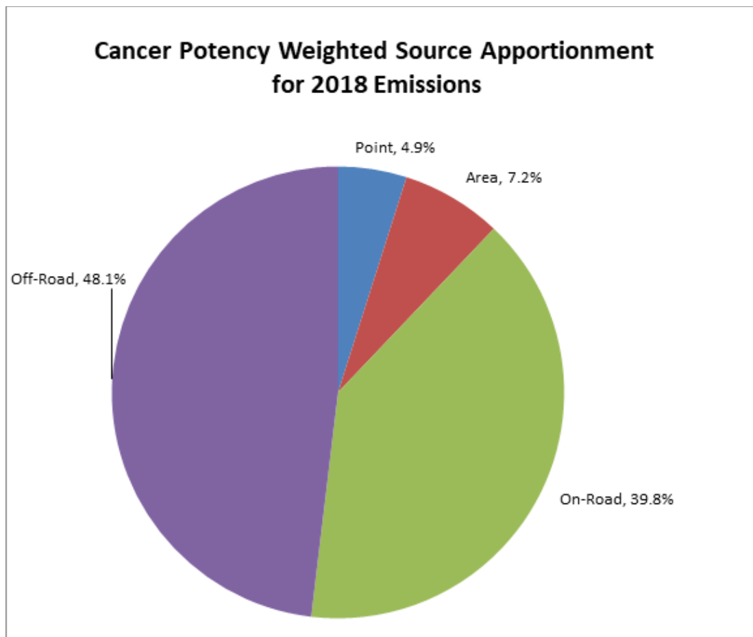
Figure 3-2. Cancer Potency Weighted Source Apportionment for 2018 Emissions.
