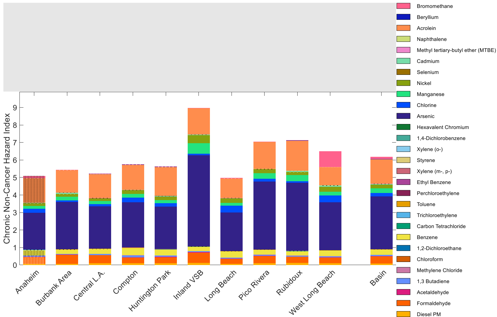
Figure 2-53 Bar charts of the cumulative chronic non-cancer hazard indices by station for MATES V. 1,2 Dibromoethane is excluded because of high uncertainty due to all measurements being below detection limit for each station. Dots are used to mark bar segments that are more uncertain due to either substitution for data that were unavailable or data for which more than 80% of measurements were below detection limit.
