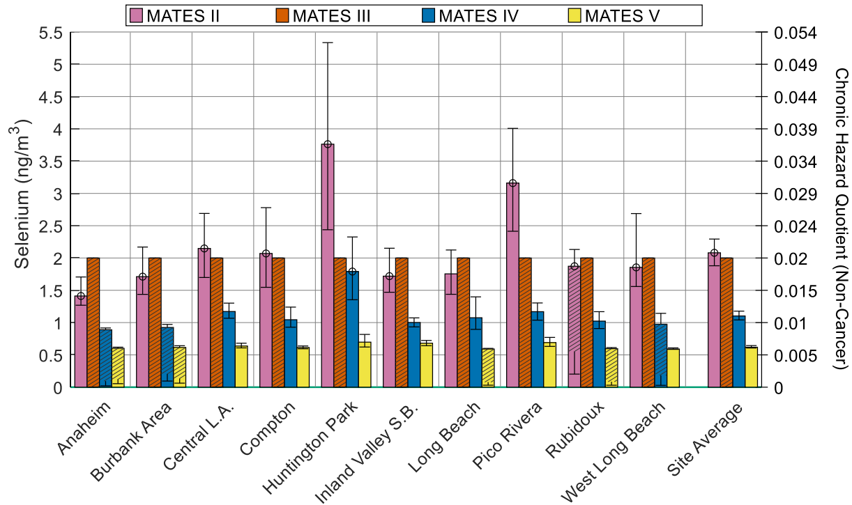
Figure 2-35 Average Concentrations of TSP Selenium. The diagonal lines (shading) on the bars indicate that more than 80% of the measurements for those stations were below the method detection limits (MDLs). The lower edge of the shading shows the mean with zero substituted for all measurements below the MDL. The upper edge of the shading shows the mean with the MDL substituted for all measurements below the MDL. All other averages are calculated using the KM mean. “o” indicates that valid measurements do not exist for at least 75% of the sampling days in each quarter. Error bars denote the 95% confidence interval.
