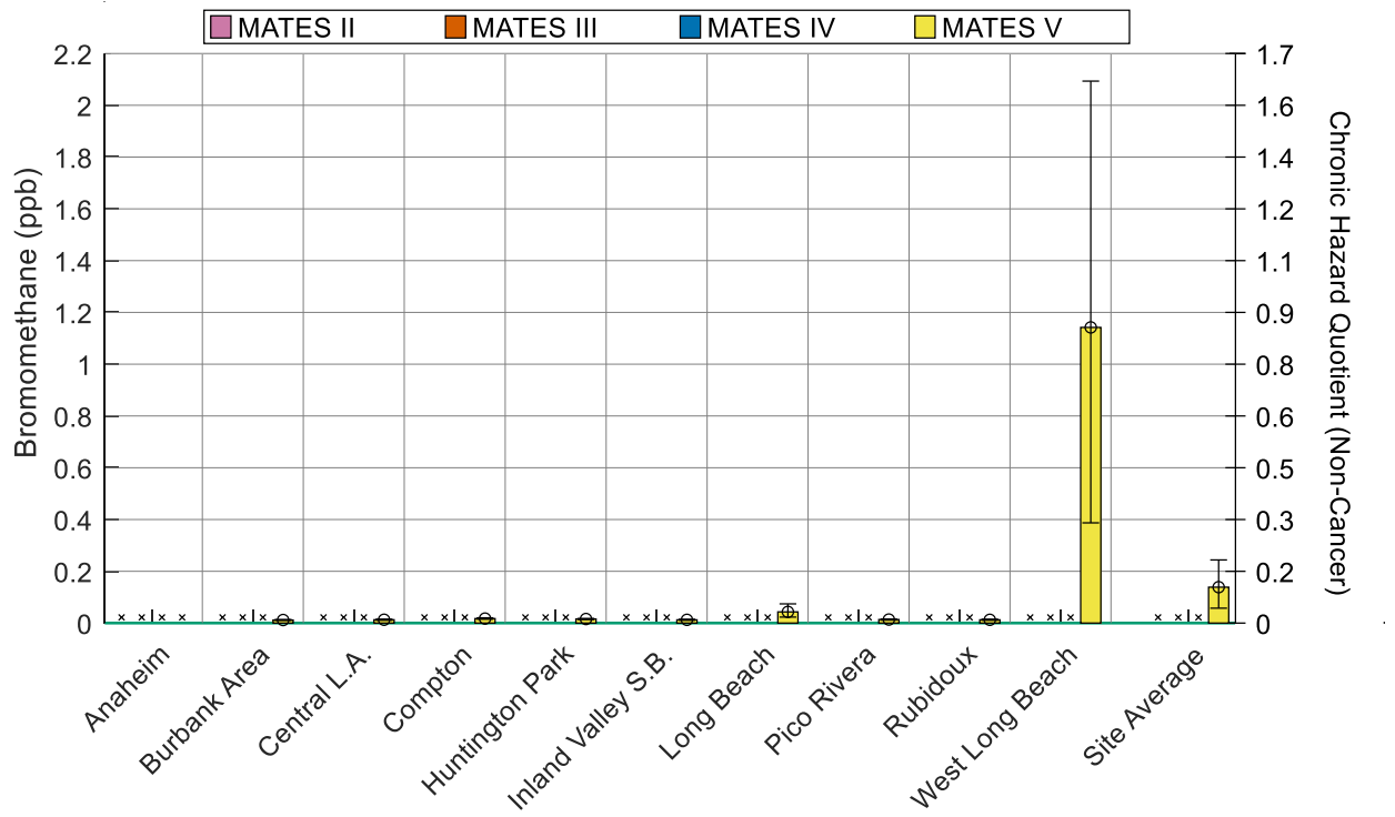
Figure 2-18 Average Concentrations of Bromomethane. “x” indicates that there is no data for a given station/MATES iteration. Note that bromomethane measurements began on August 12, 2018 and therefore, do not constitute a complete year of measurements. “o” indicates that valid measurements do not exist for at least 75% of the sampling days in each quarter. Error bars denote the 95% confidence interval.
