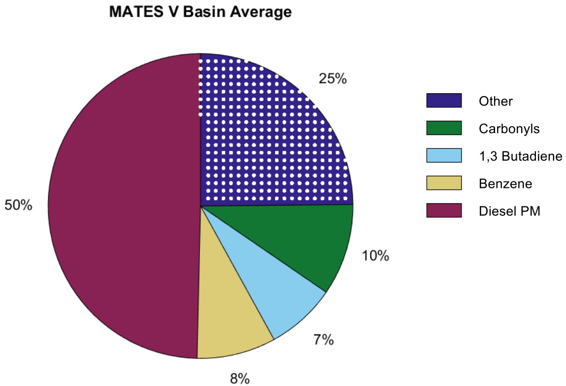
Figure 2-49 Pie charts of the basin-wide cumulative cancer risks for MATES V. 1,2 Dibromoethane is excluded because of high uncertainty due to all measurements being below detection limit for each station. Dots are used to mark segments that are more uncertain due to either substitution for data that were unavailable or data for which more than 80% of measurements were below detection limit. Numbers may not sum to 100 due to rounding.
