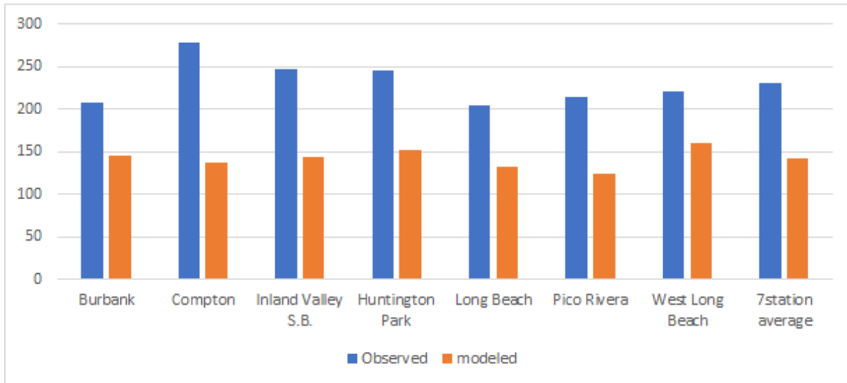
Figure 4-12 MATES V Simulated vs. Measured Non-Diesel Inhalation Air Toxics Cancer Risk (Per Million)
