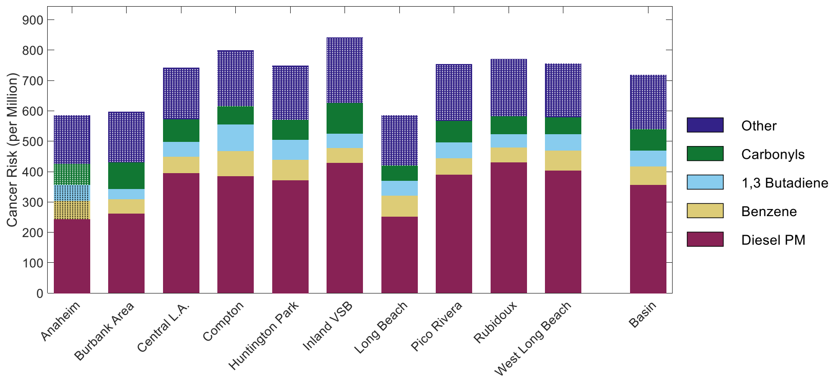
Figure 2-48 Bar charts of the cumulative cancer risks by station for MATES V with grouped analytes. 1,2 Dibromoethane is excluded because of high uncertainty due to all measurements being below detection limit for each station. Dots are used to mark bar segments that are more uncertain due to either substitution for data that were unavailable or data for which more than 80% of measurements were below detection limit.
