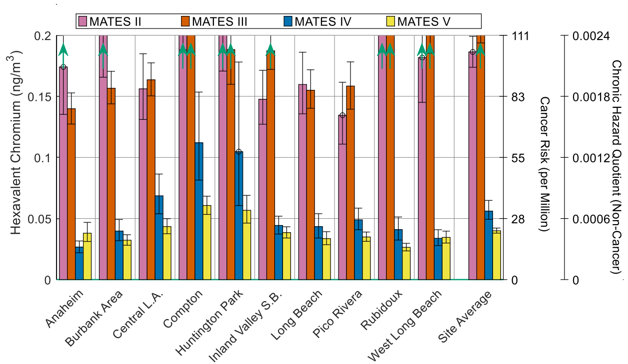
Figure 2-32 Average Concentrations of TSP Hexavalent Chromium. The upward arrows indicate that the data extends above the y-axis shown. “o” indicates that valid measurements do not exist for at least 75% of the sampling days in each quarter. Error bars denote the 95% confidence interval.
