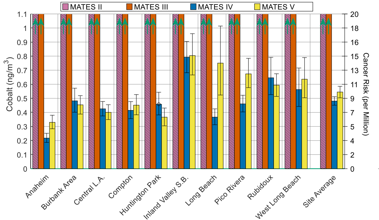
Figure 2-38 Average Concentrations of TSP Cobalt. The upward arrows indicate that the data extends above the y-axis shown. “o” indicates that valid measurements do not exist for at least 75% of the sampling days in each quarter. Error bars denote the 95% confidence interval.
